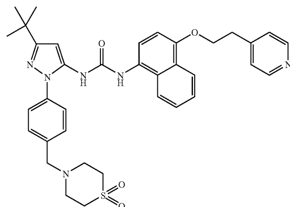
Example 117
