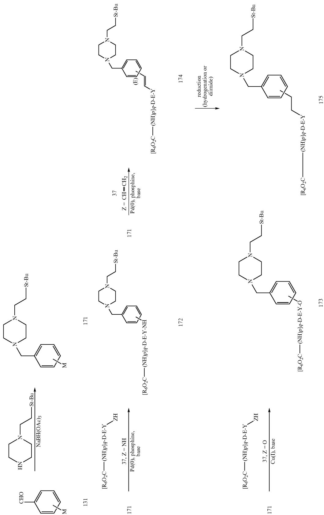
Scheme 28.1
