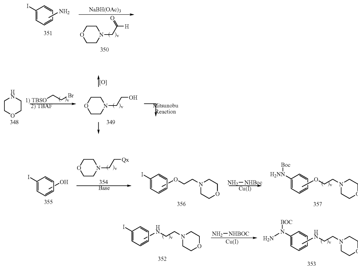
Scheme 63
