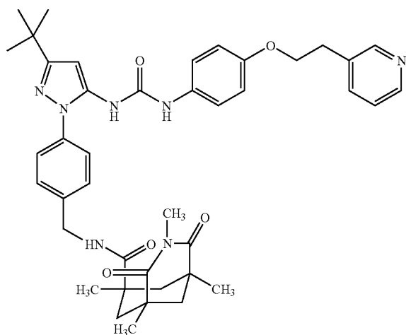
Example 114
