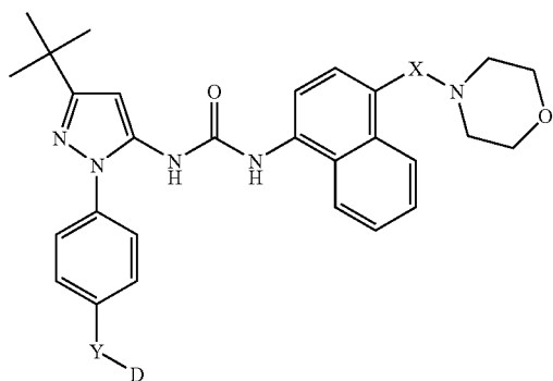
Example 73
