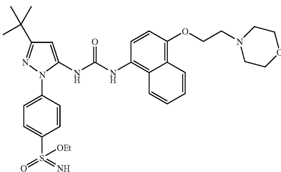
Example 139
