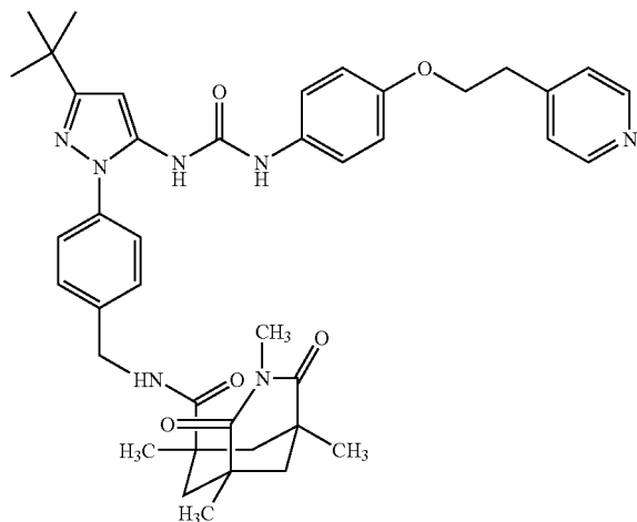
Example 112
