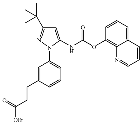
Example 172
