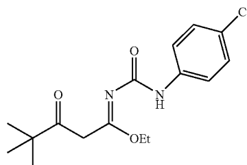
Example QQ
