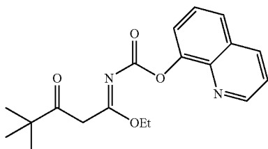
Example MM
