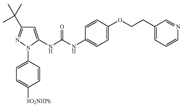
Example 138
