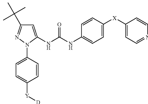
Example 76
