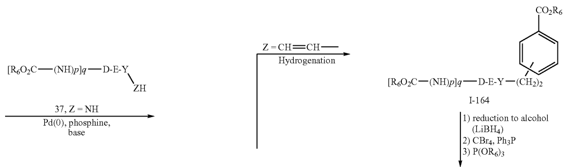
Scheme 26
