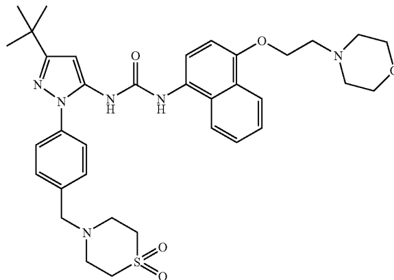
Example 115
