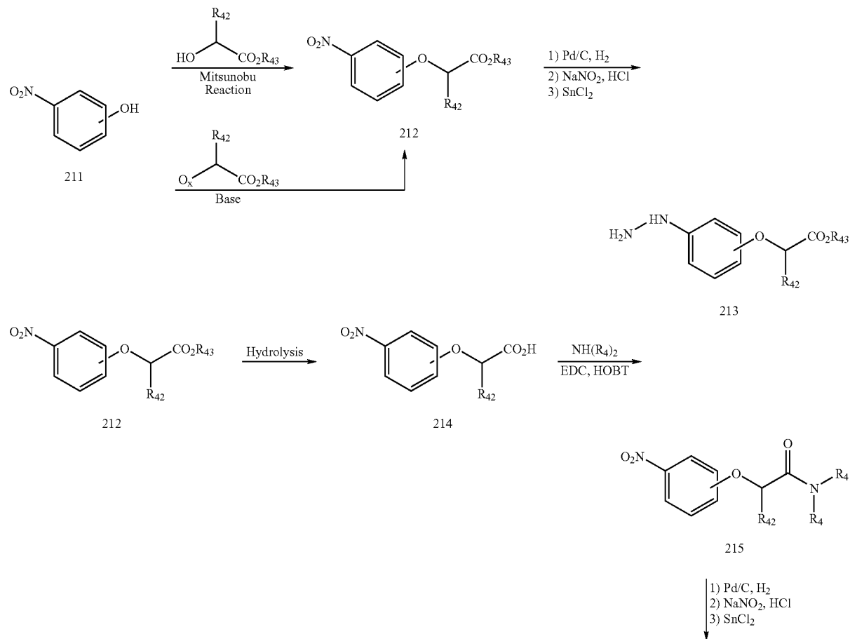
Scheme 39
