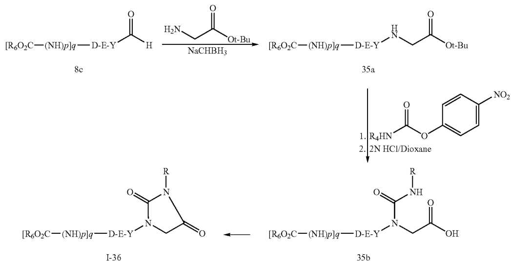
Scheme 6.1
