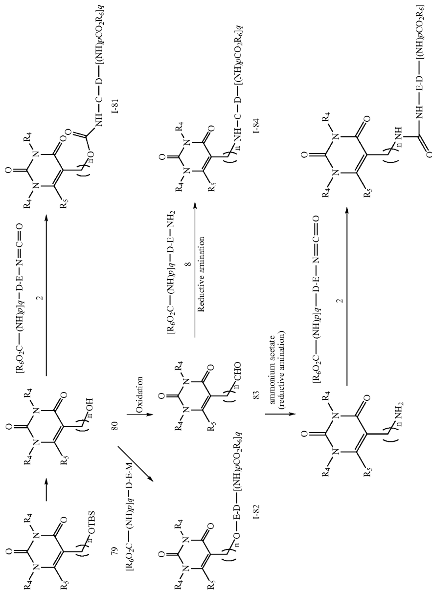
Scheme 14
