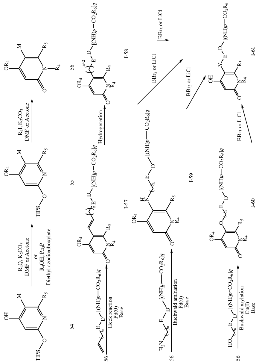
Scheme 10
