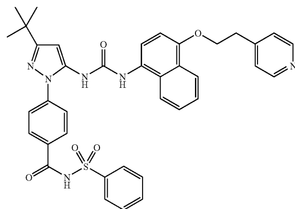
Example 123
