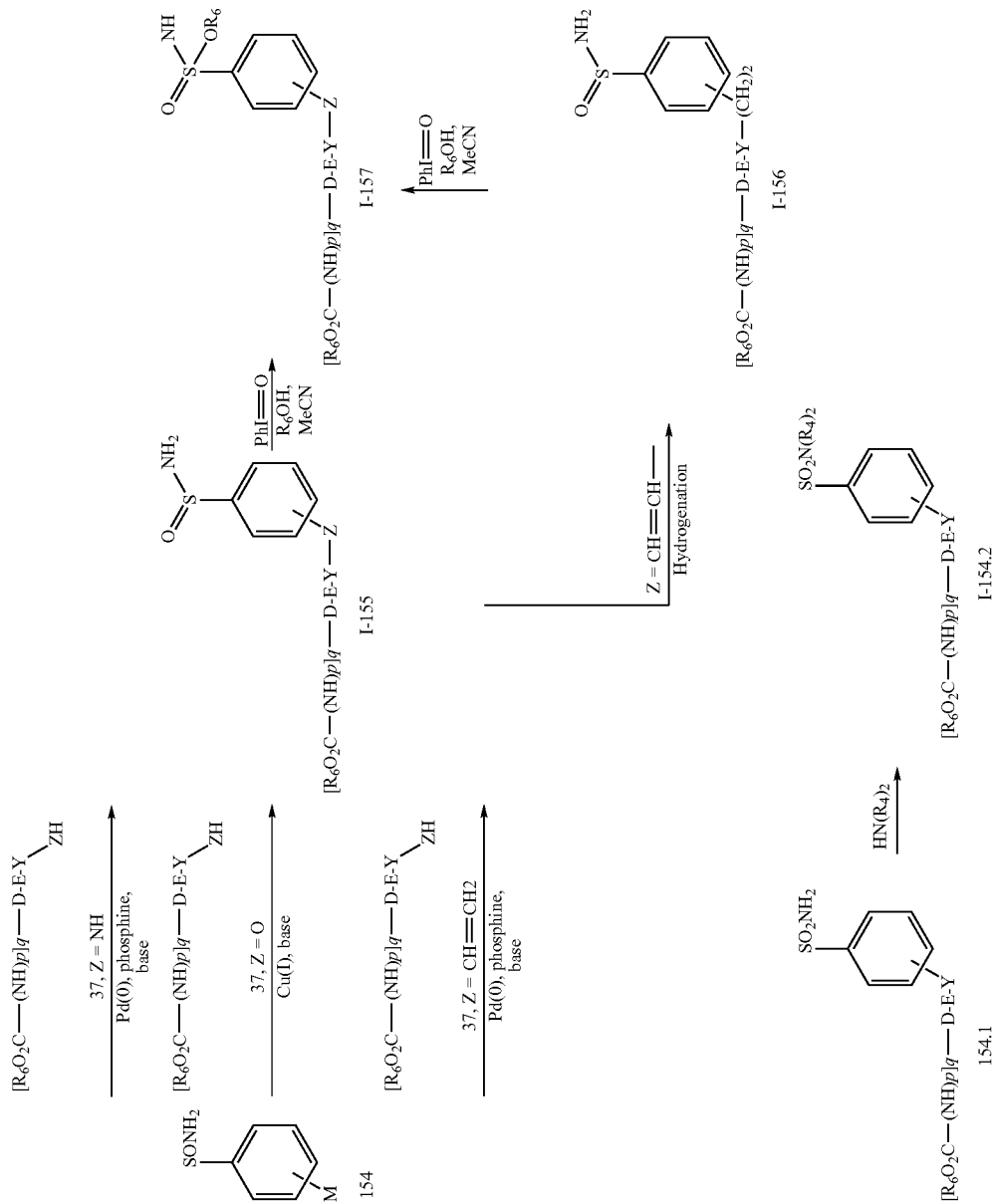
Scheme 24
