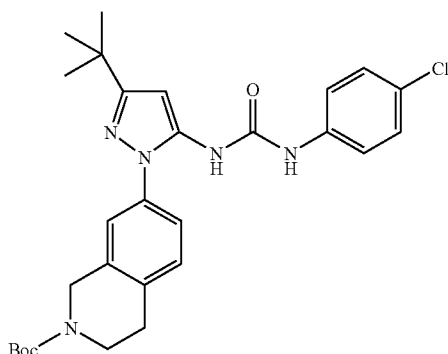
Example 250
