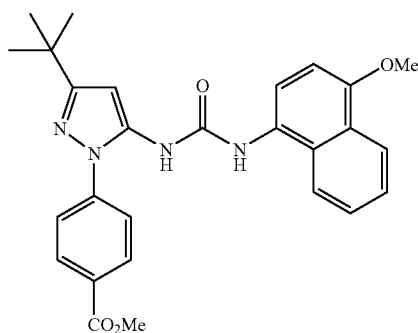
Example 58
