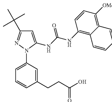
Example 175
