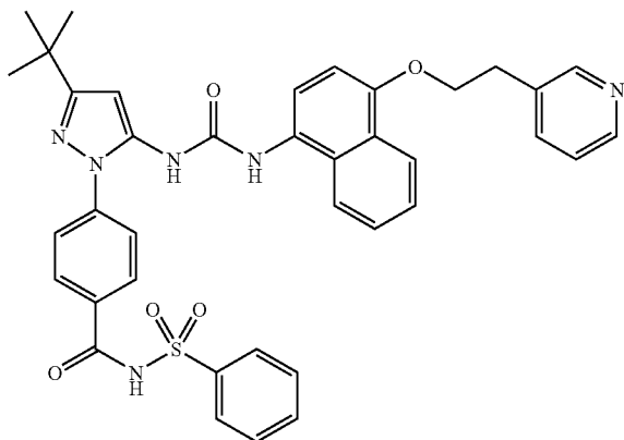
Example 125
