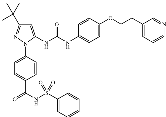
Example 126
