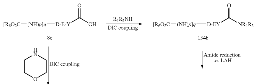
Scheme 21.2
