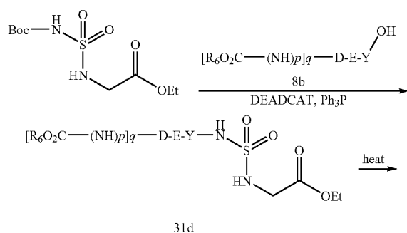
Scheme 5.3
