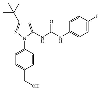
Example 60
