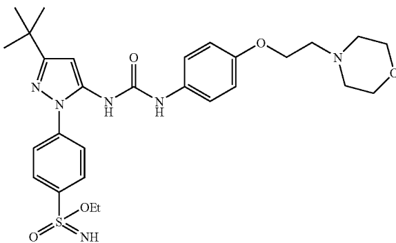
Example 140
