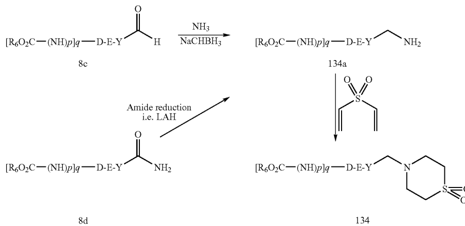
Scheme 21.1
