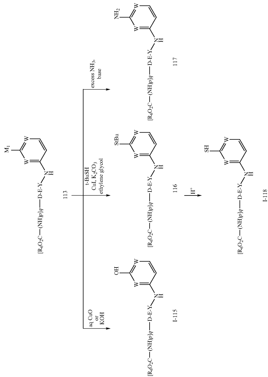
Scheme 19.2
