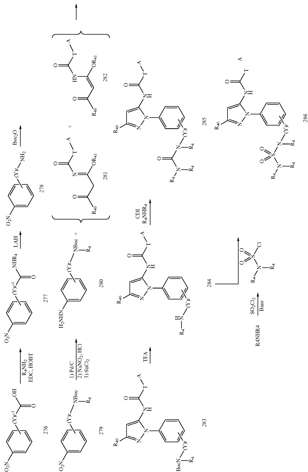
Scheme 52
