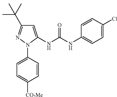
Example 57
