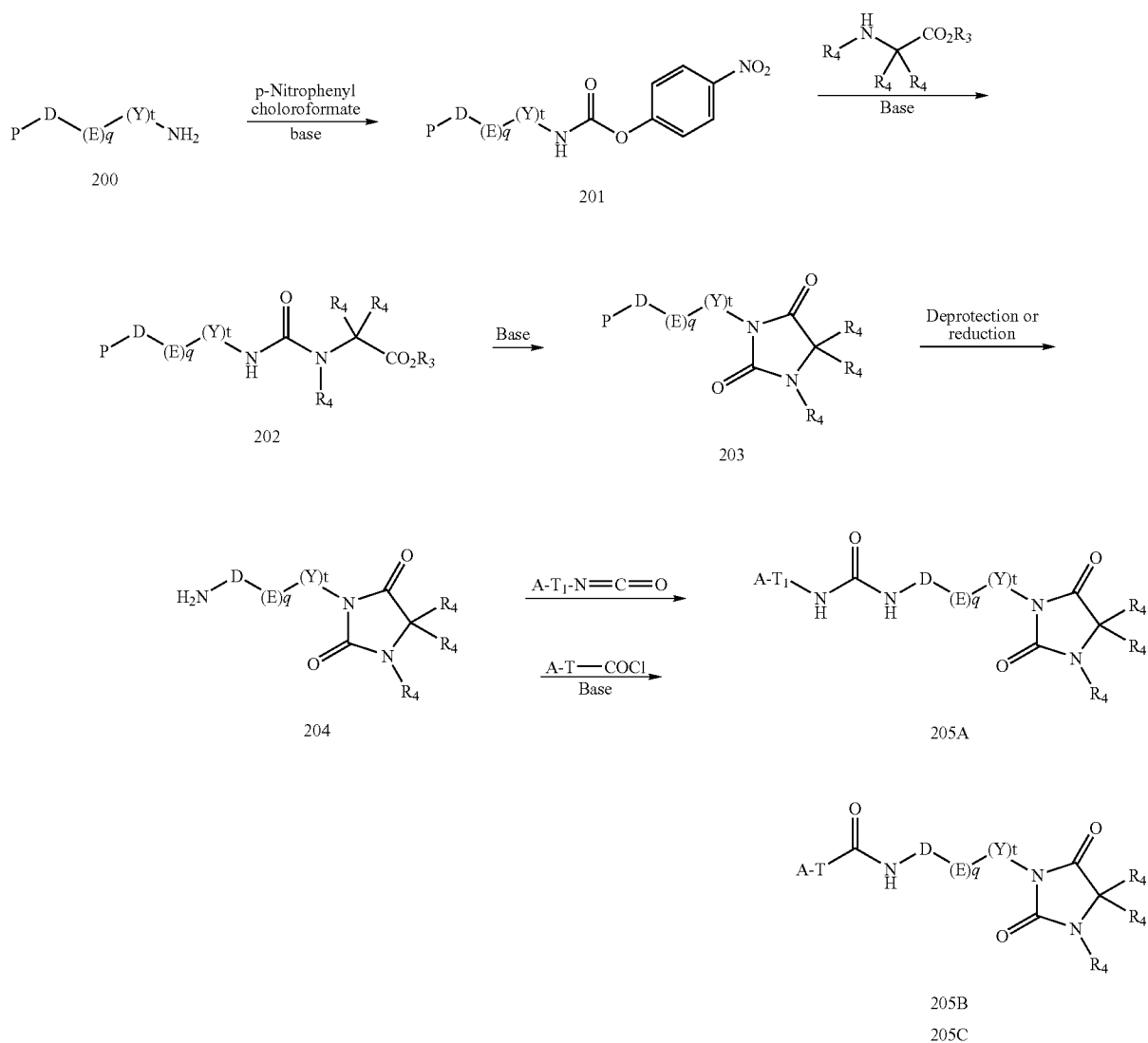
Scheme 37
