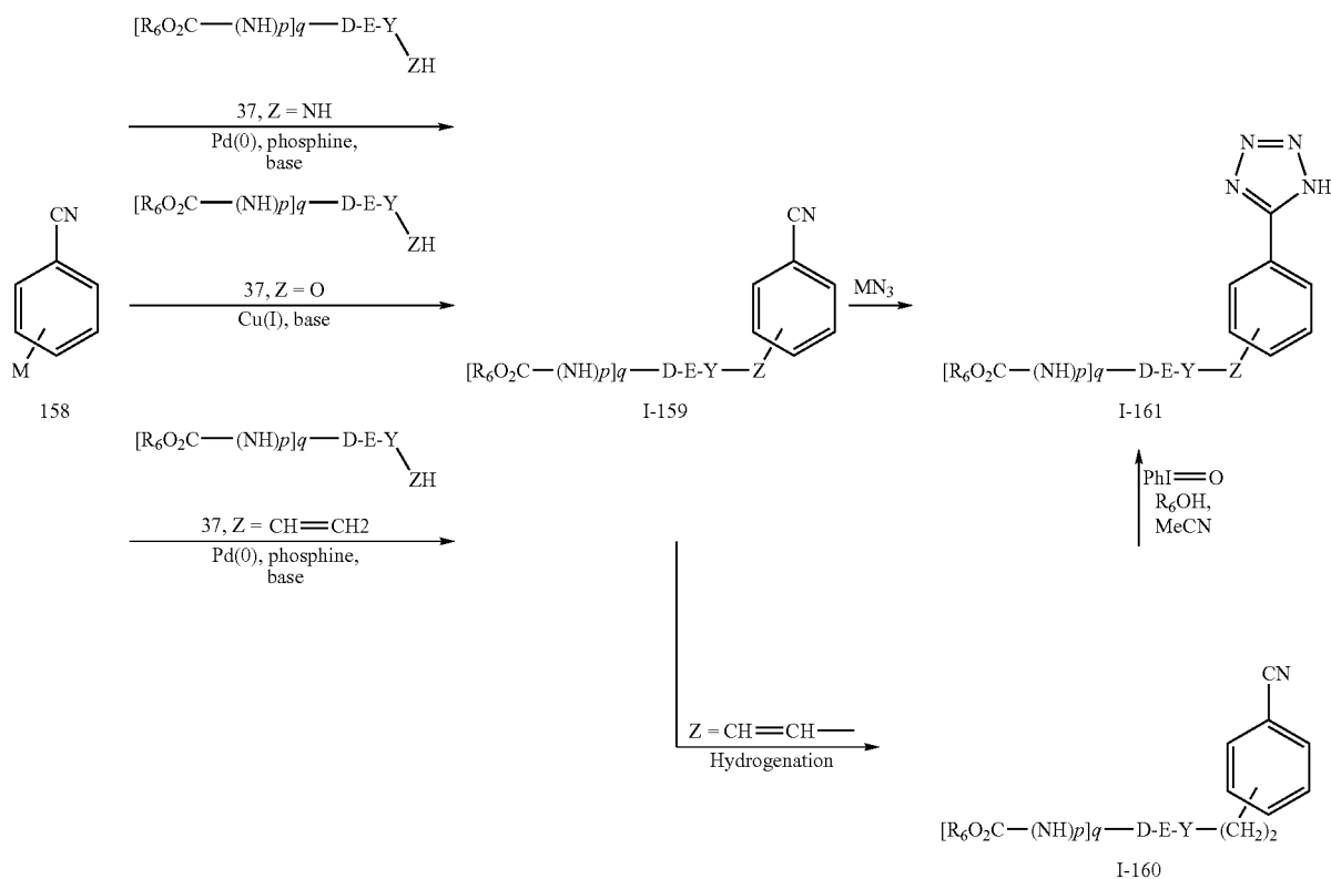
Scheme 25
