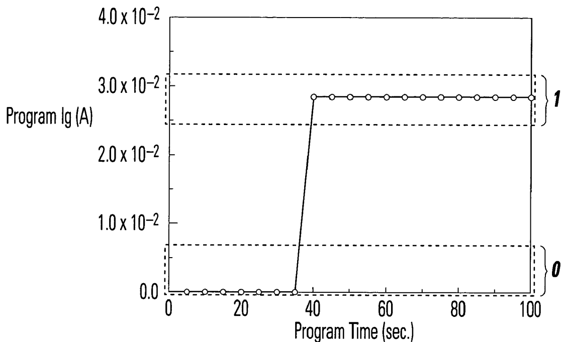
FIG. 4 (Prior Art)
