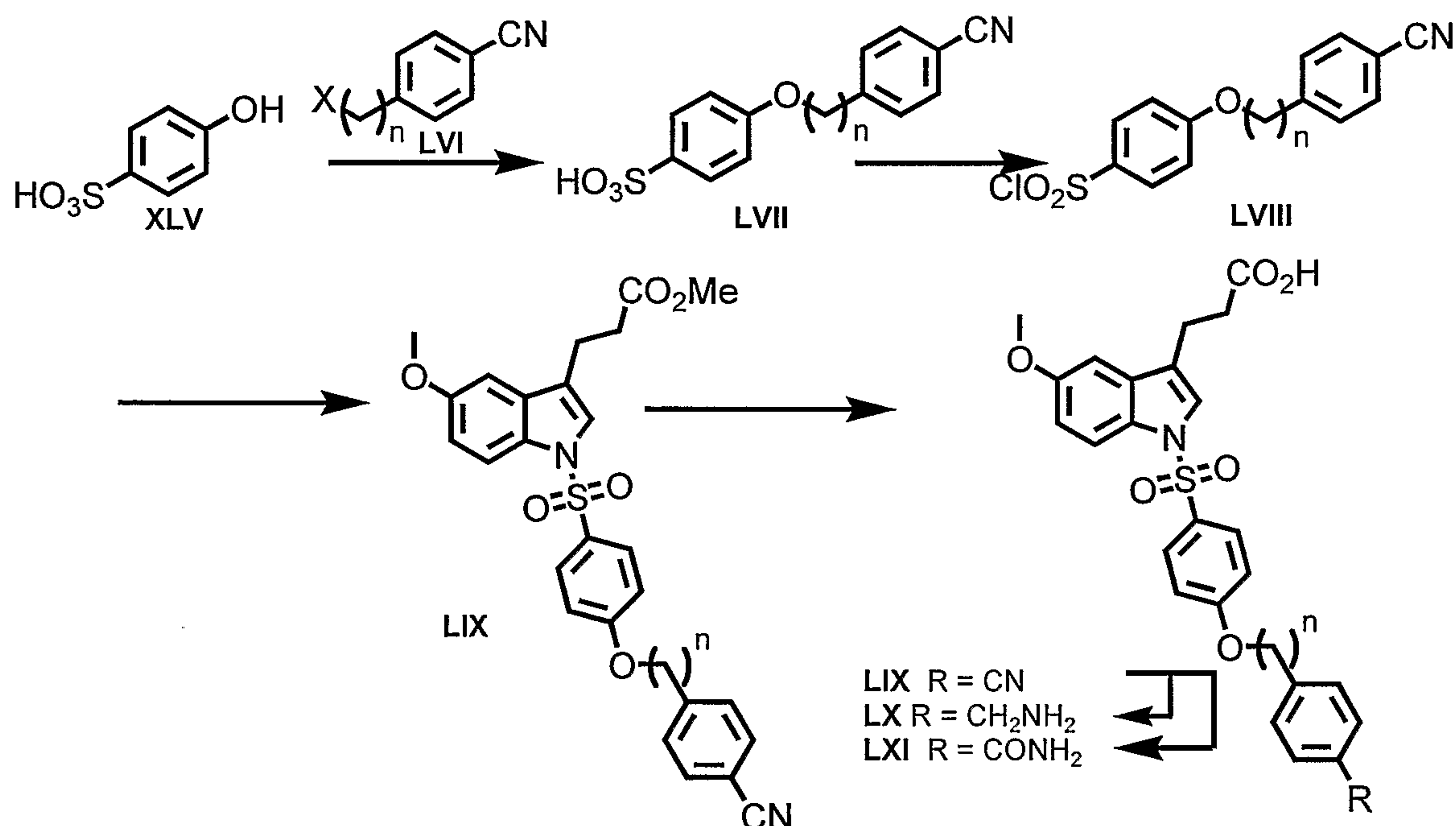
Scheme 25
