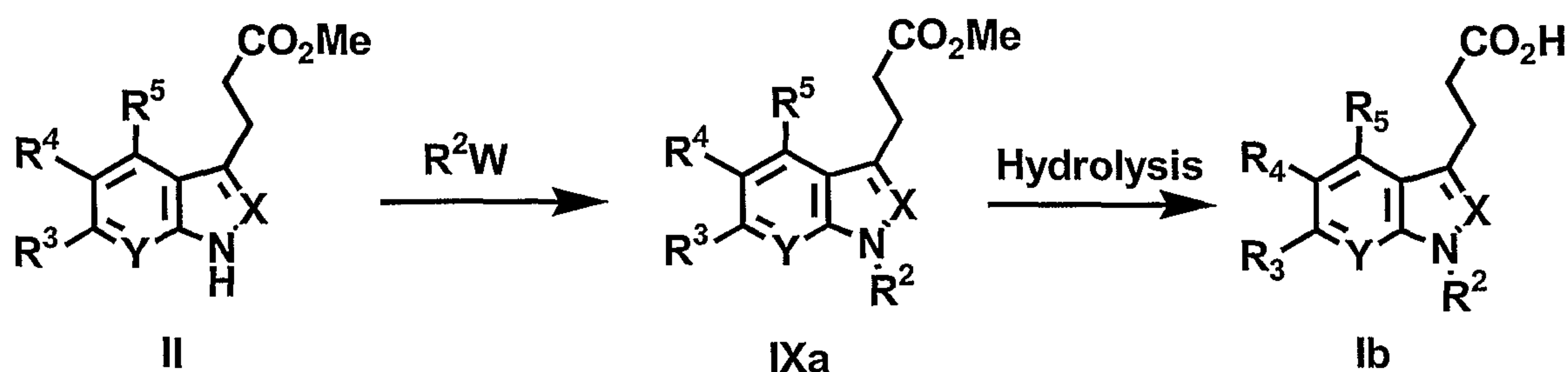
Scheme 3
