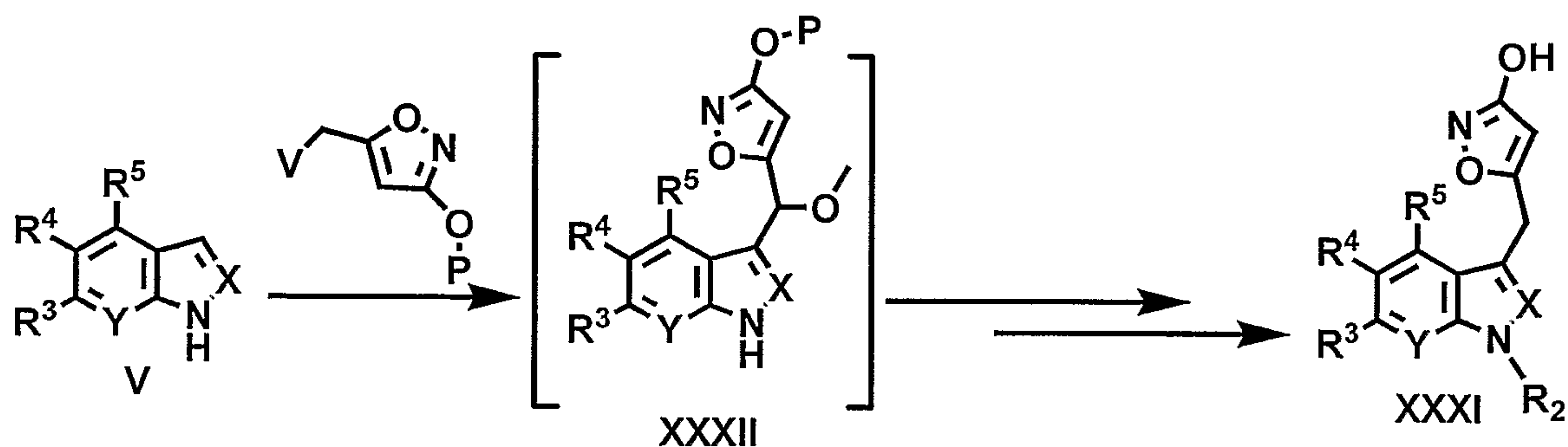
Scheme 18
