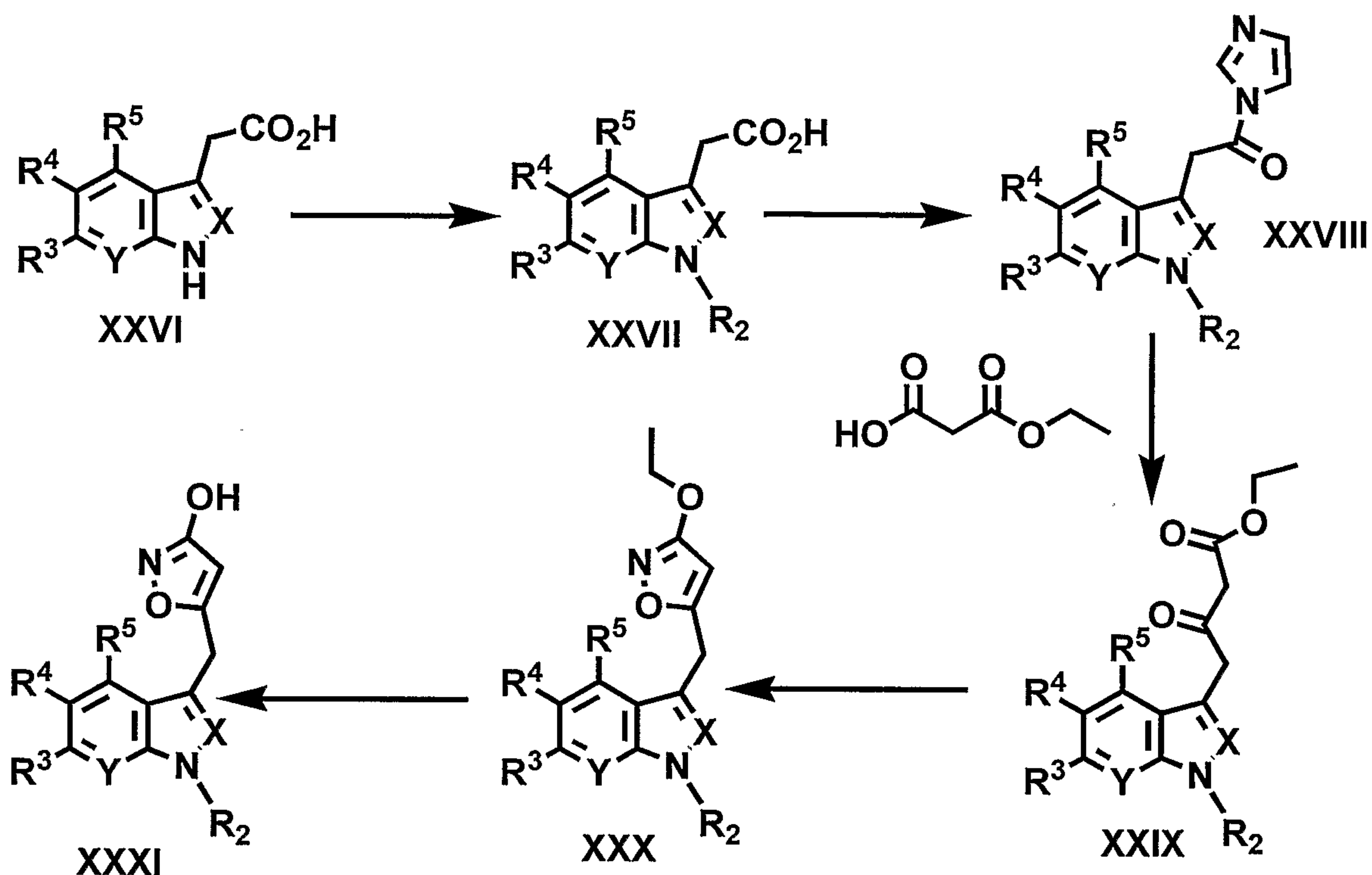
Scheme 17
