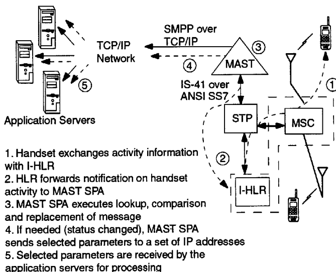
MAST - Architecture and Information Flow
