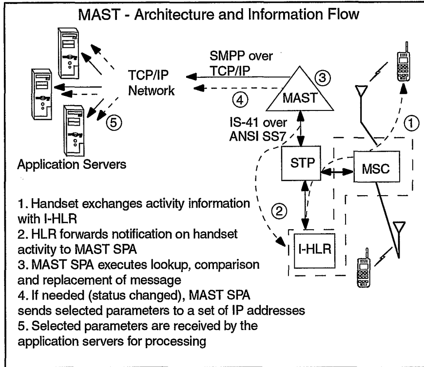
MAST Architecture and Information Flow
