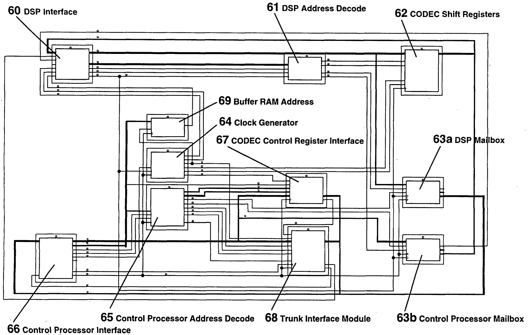
Fig. 6 Multi-Port PSTN Module Control Logic
