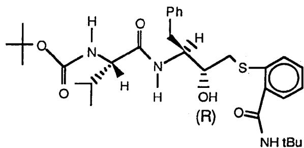
INTERMEDIATE NO. 4
