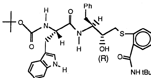
INTERMEDIATE NO. 6
