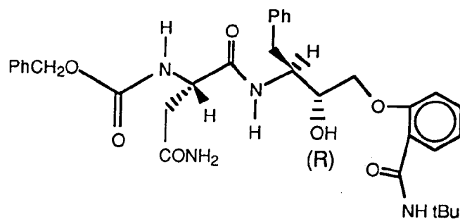
INTERMEDIATE NO. 1
