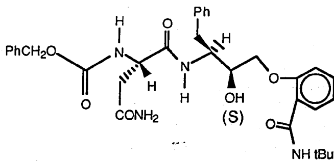
INTERMEDIATE NO. 8
