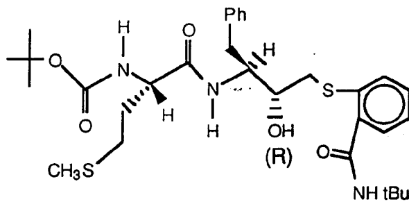
INTERMEDIATE NO. 5
