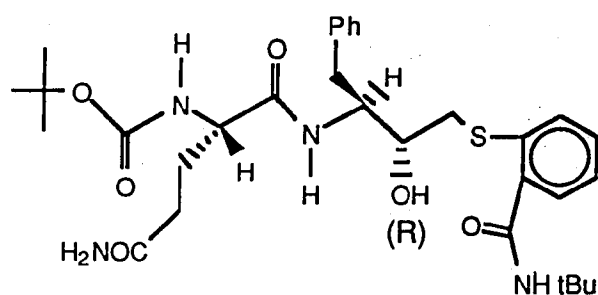
INTERMEDIATE NO. 3
