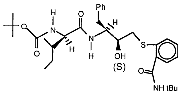
INTERMEDIATE NO. 7
