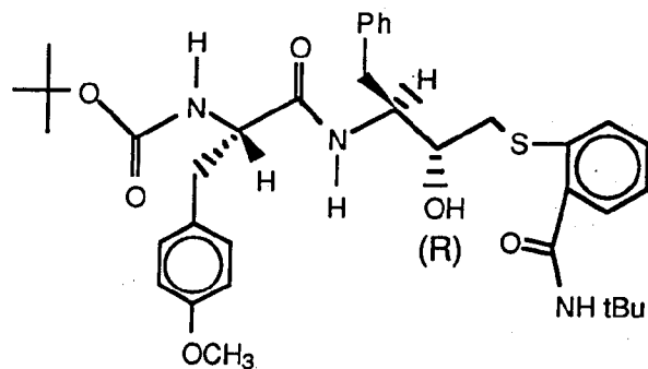
INTERMEDIATE NO. 2
