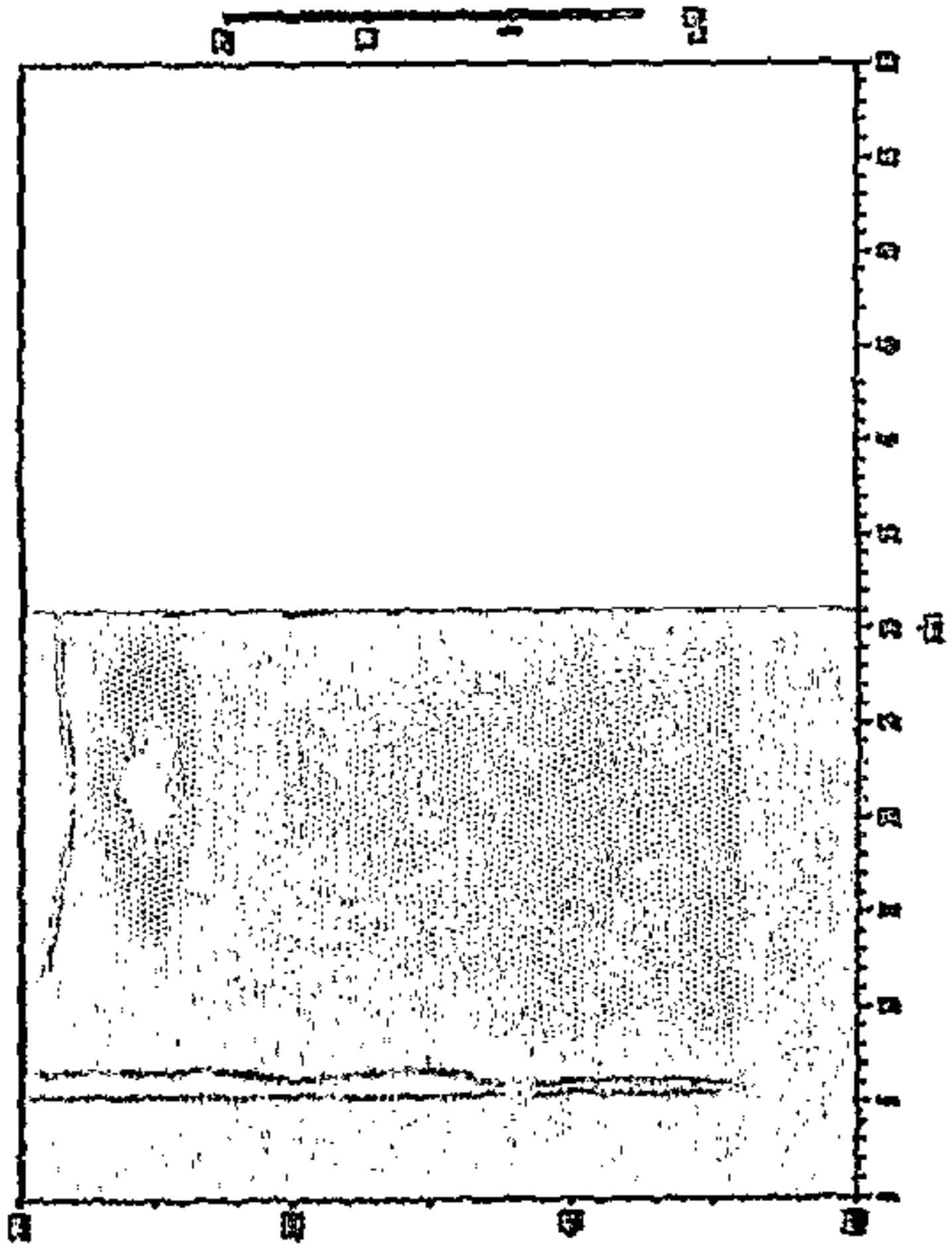
BERBERIN (FLUKA STANDARD)
