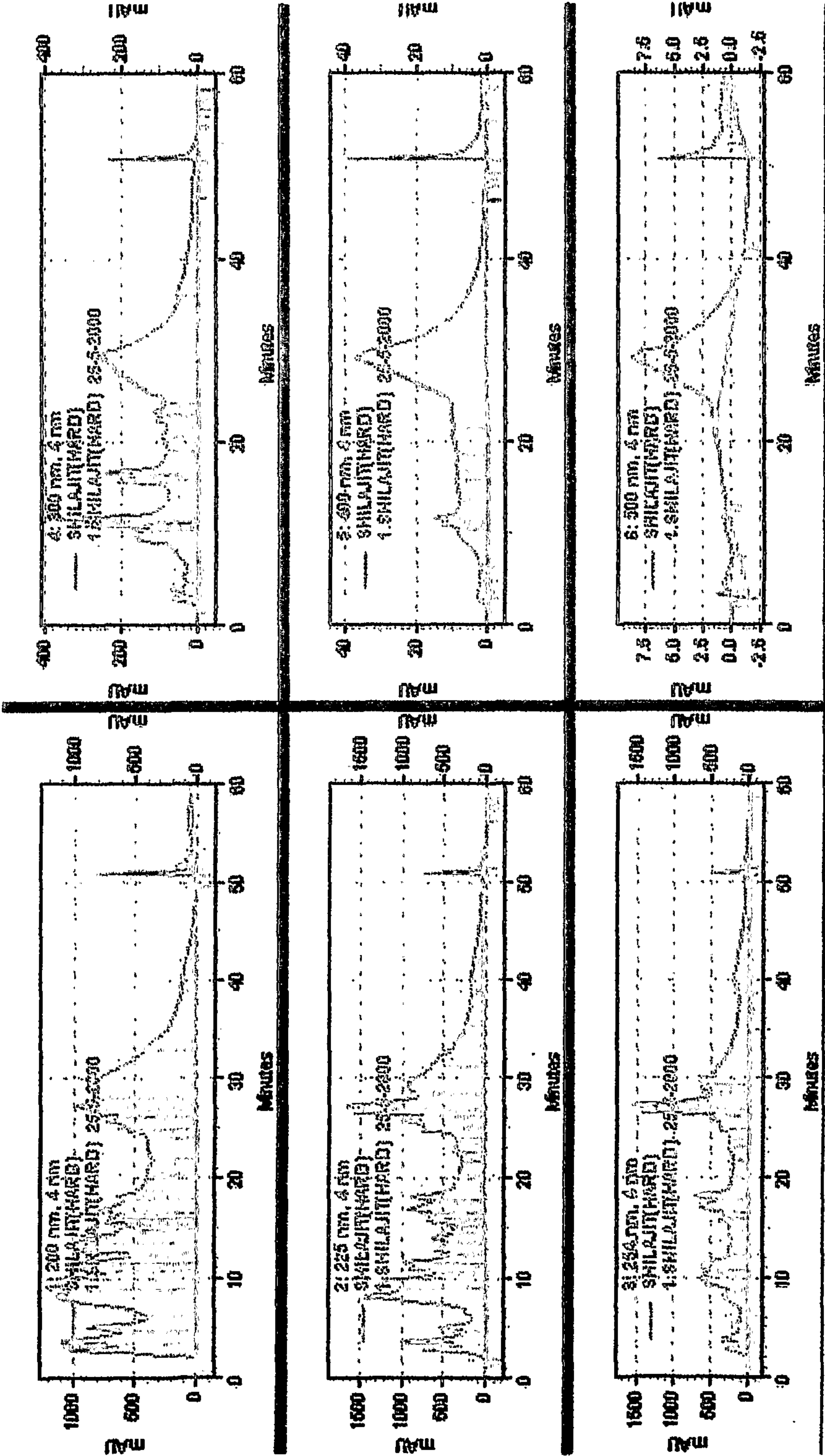
Figure 9 CHROMATOGRAMS OF A HERBOMINERAL MEDICINE SHILAJIT (POOR BY EFFICACY) AT DIFFERENT WAVELENGTHS (The existing method)
