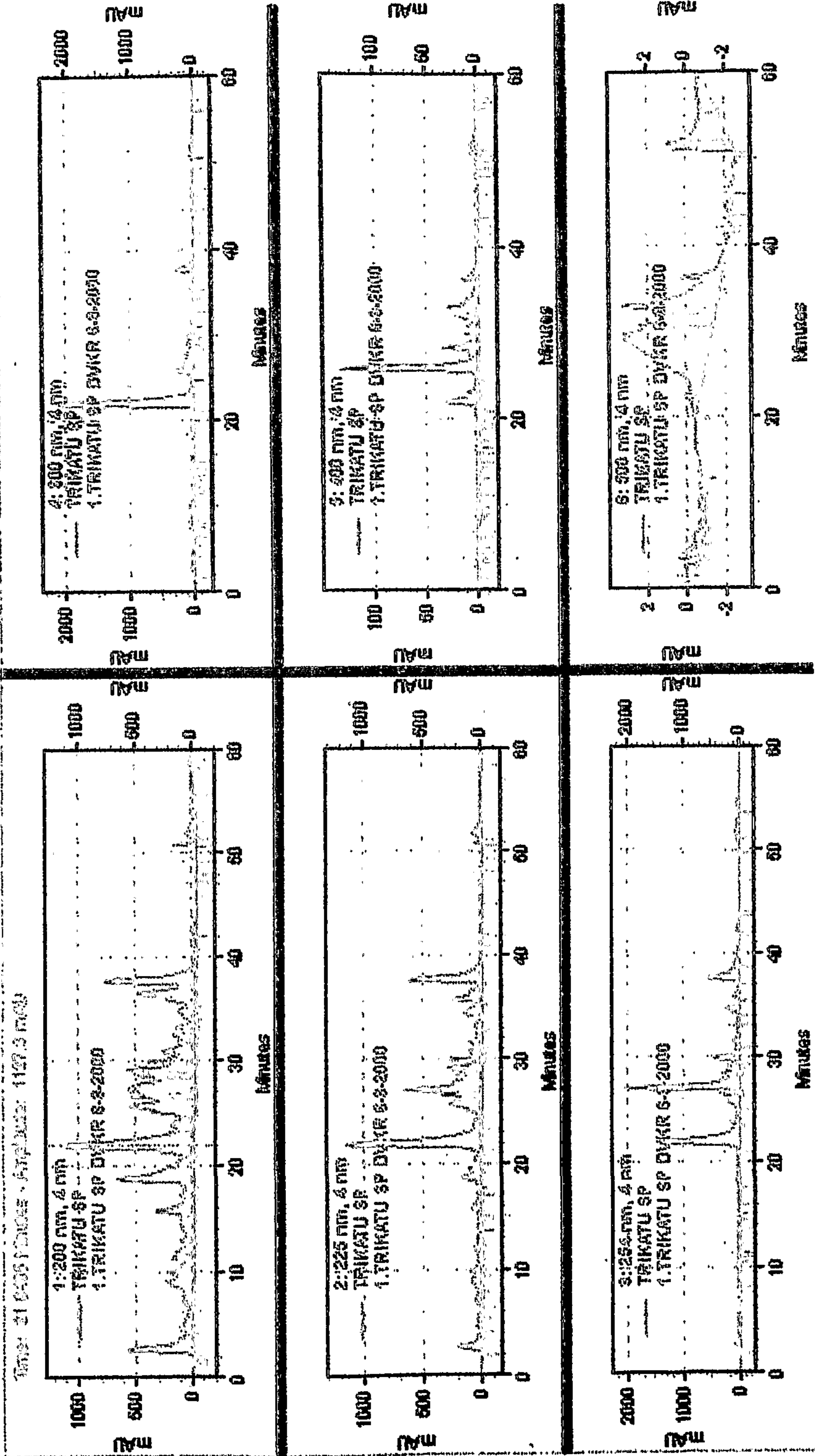
Figure 12 CHROMATOGRAMS OF A HERBAL FORMULATION TRIKTU (A FORMULATION OF PIPPALI, MARICHA AND SHUNTI) AT DIFFERENT WAVELENGTHS (The existing method)
