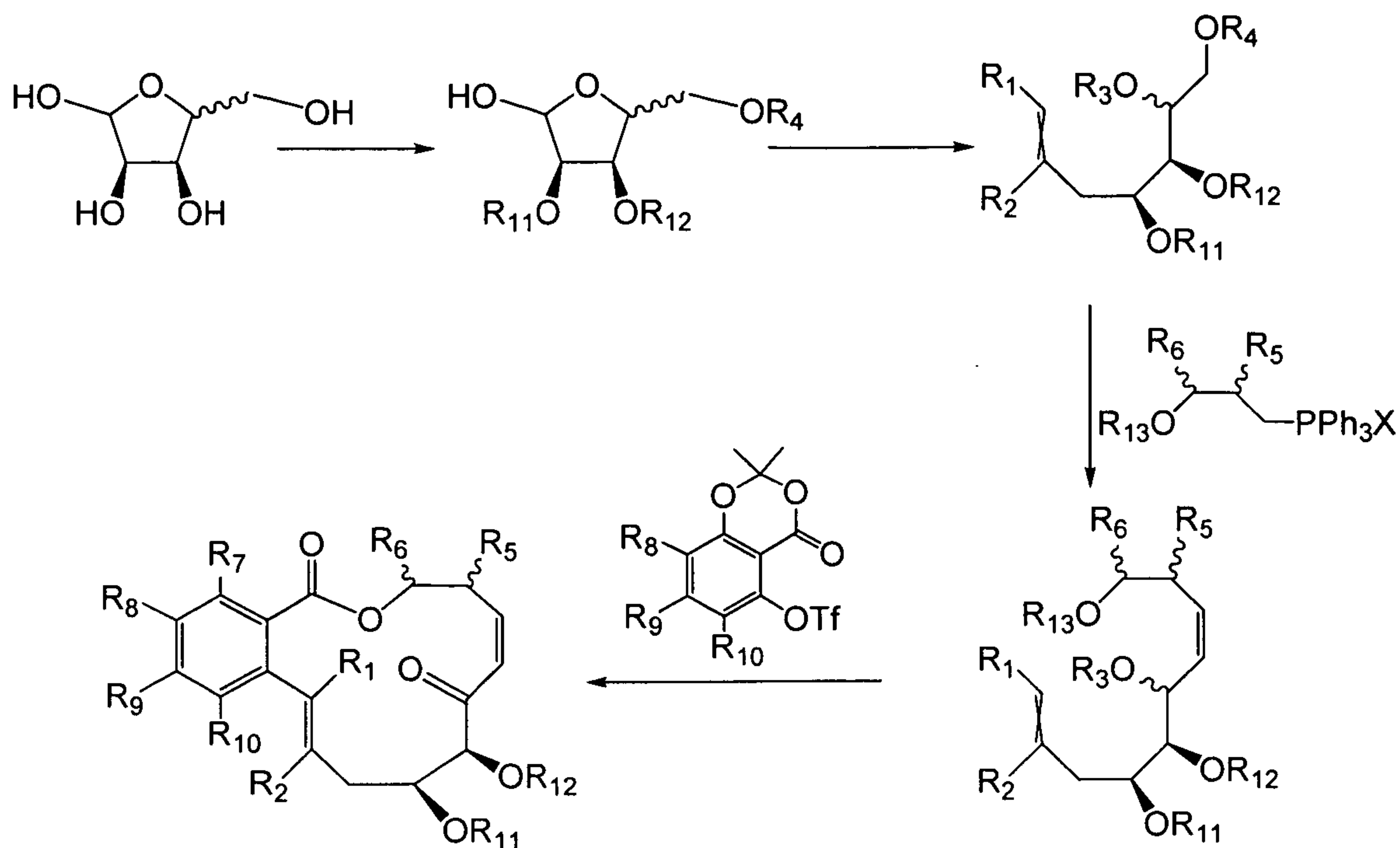
Scheme 1: Synthesis of formula (IV) from ribose – route 1
