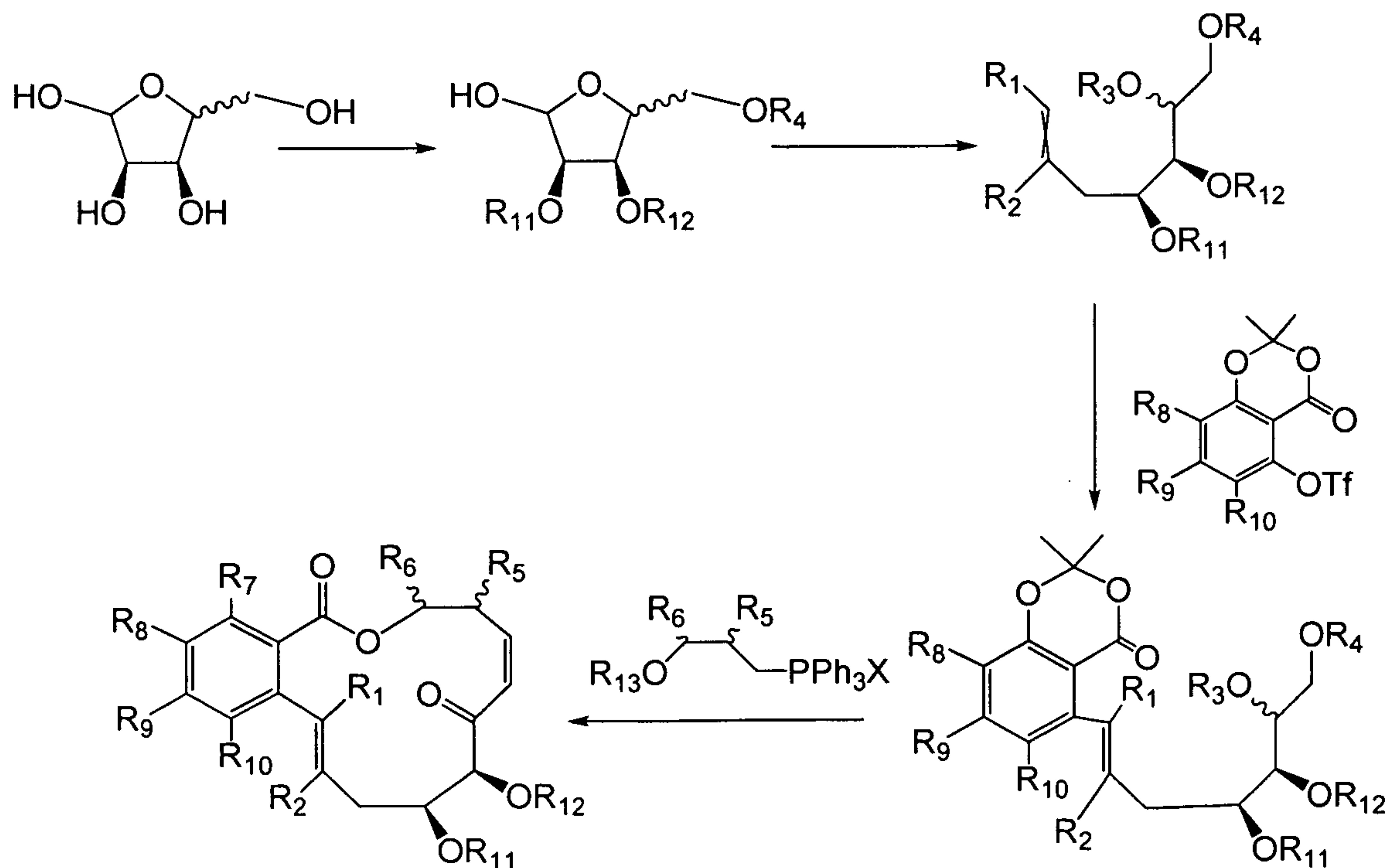
Scheme 2: Synthesis of formula (IV) from ribose – route 2
