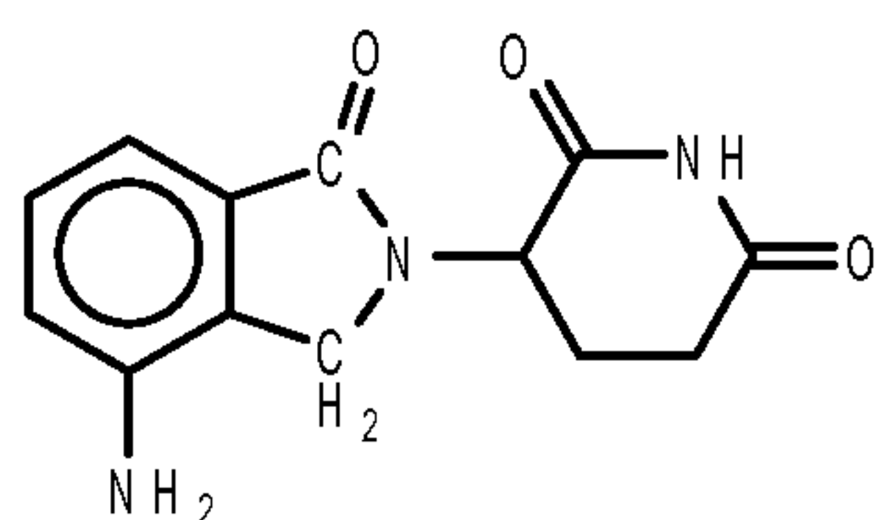
1-oxo-2-(2,6-dioxopiperidin-3-yl)-4-aminoisoindoline
