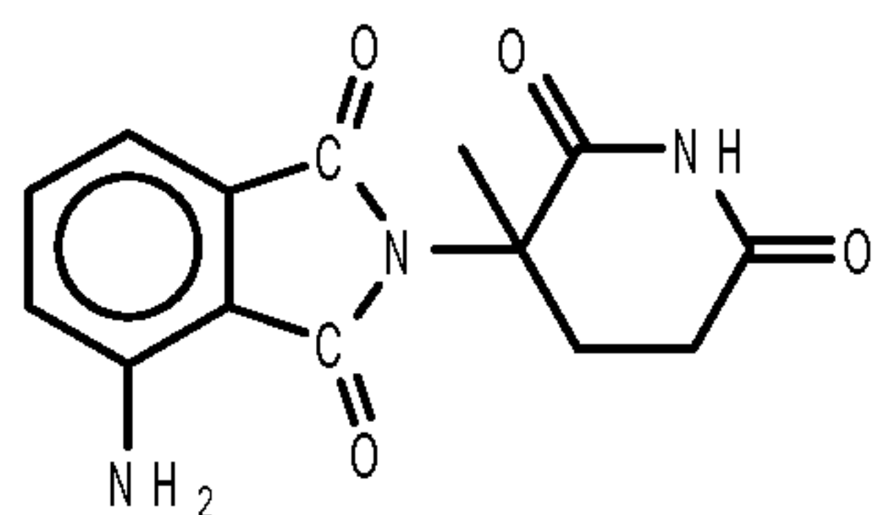
1,3-dioxo-2-(3-methyl-2,6-dioxopiperidin-3-yl)-4-
