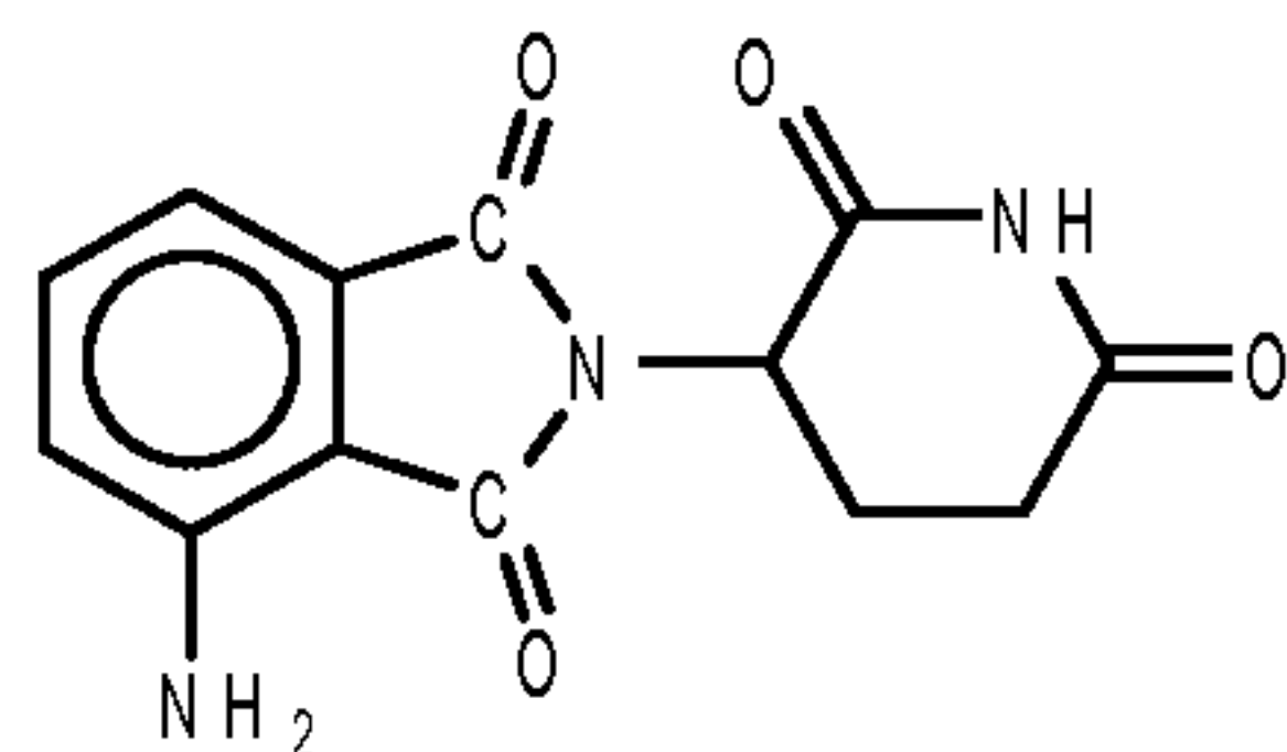
1,3-dioxo-2-(2,6-dioxopiperidin-3-yl)-4-aminoisoindoline
