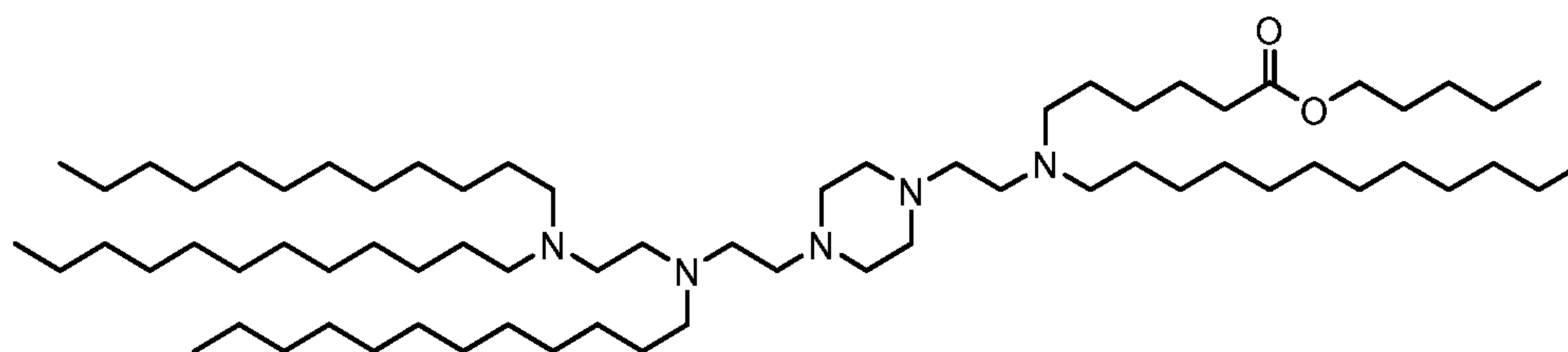
(Compound 244),
