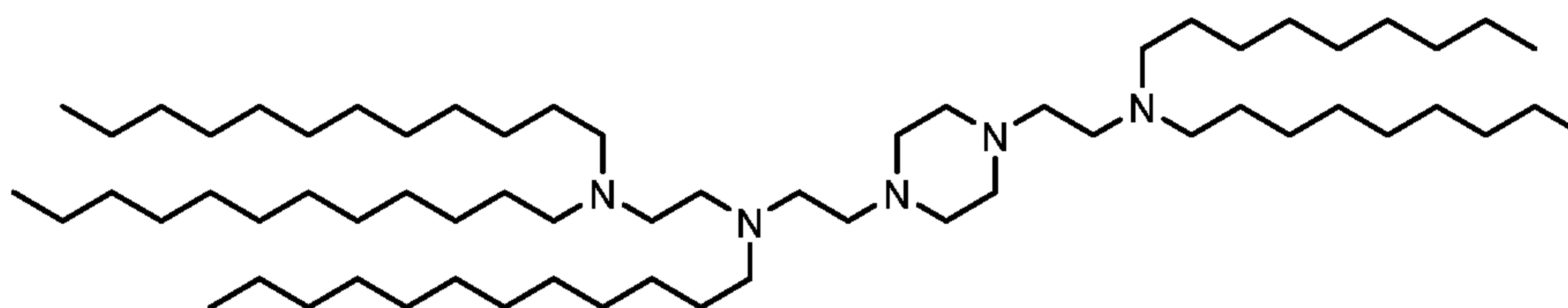
(Compound 255),
