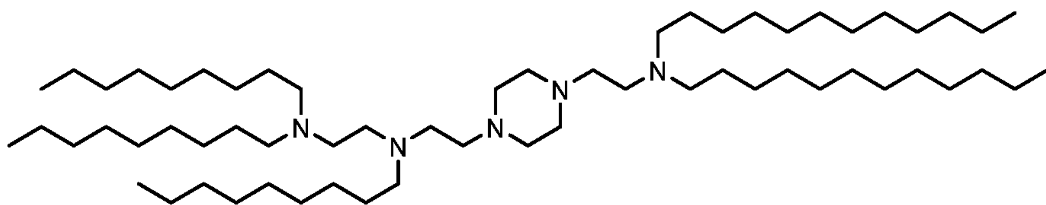
(Compound 251),
