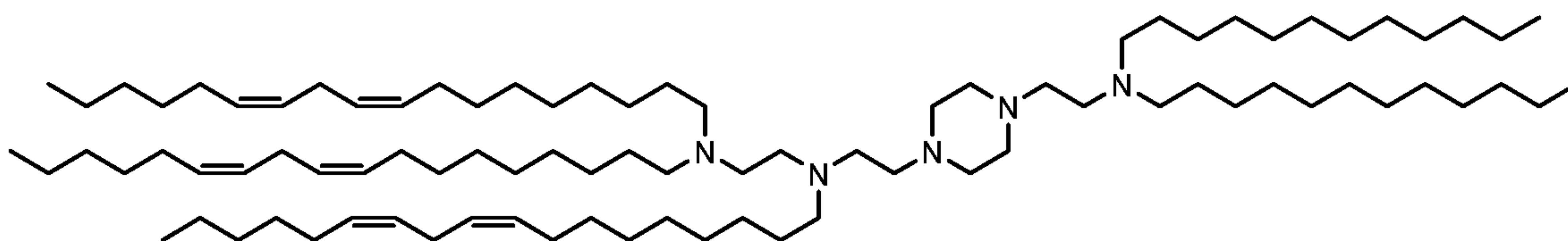
(Compound 266).
