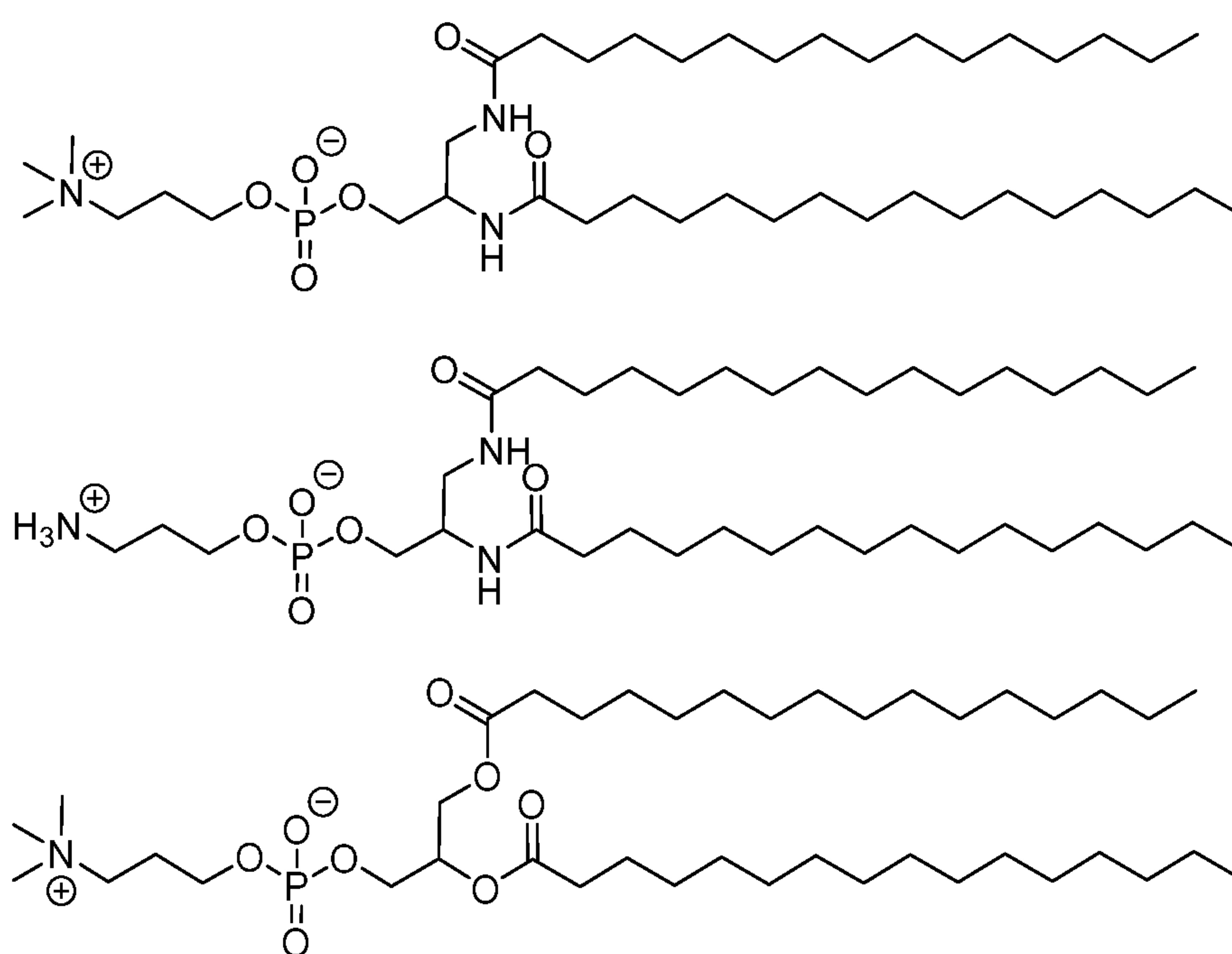
(Compound 412)
