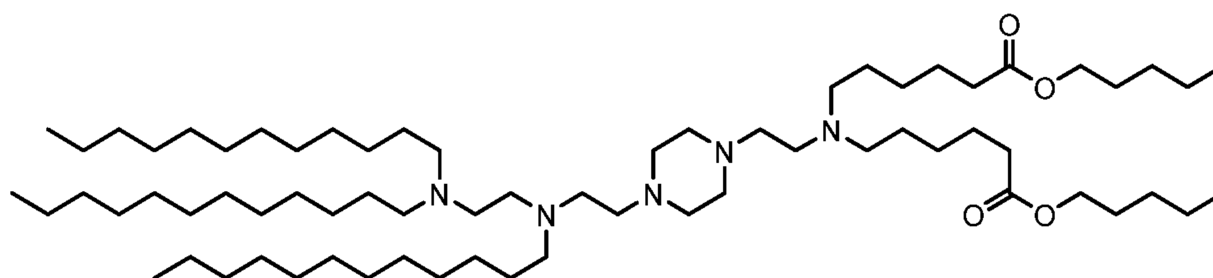
(Compound 246),
