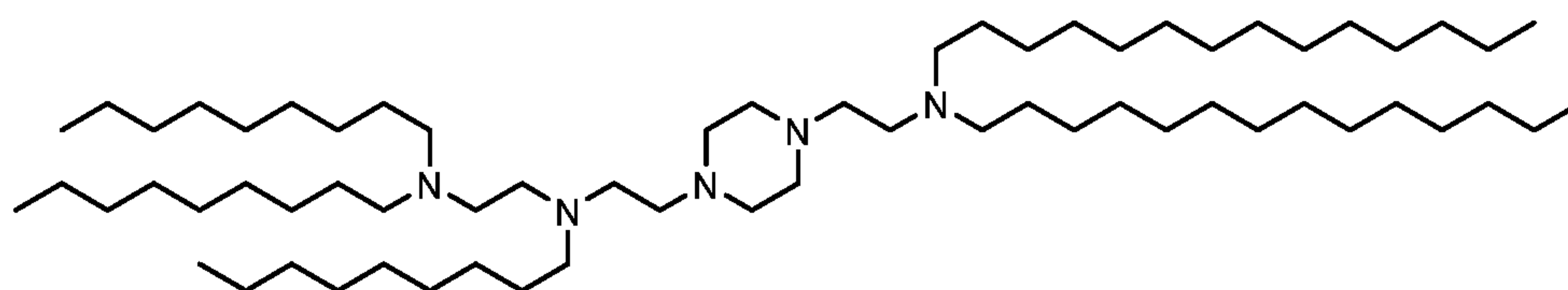
(Compound 252),
