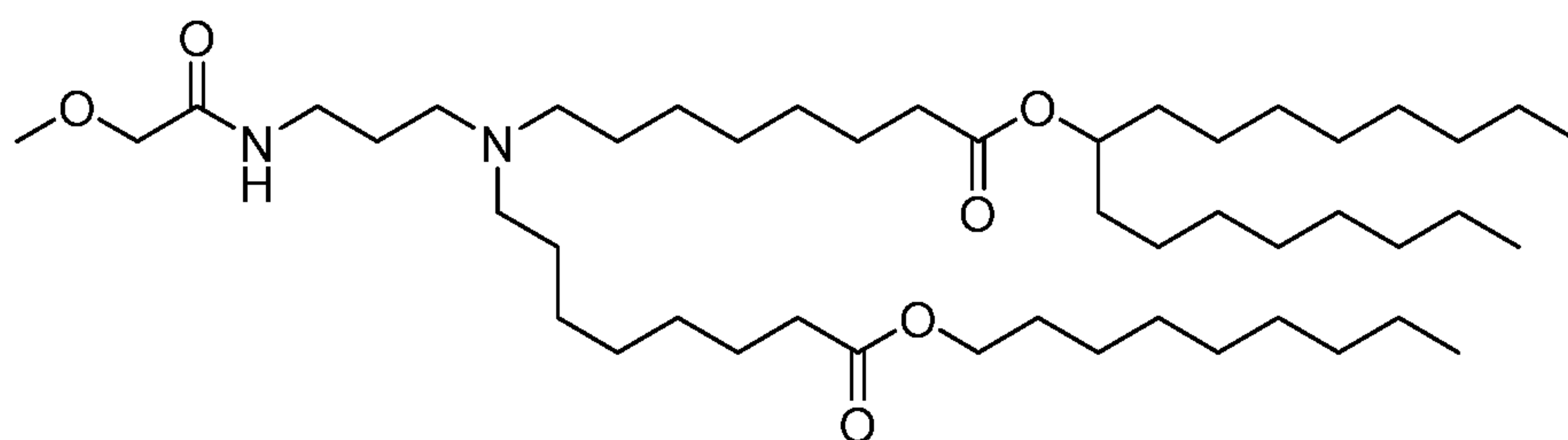
(Compound 178),
