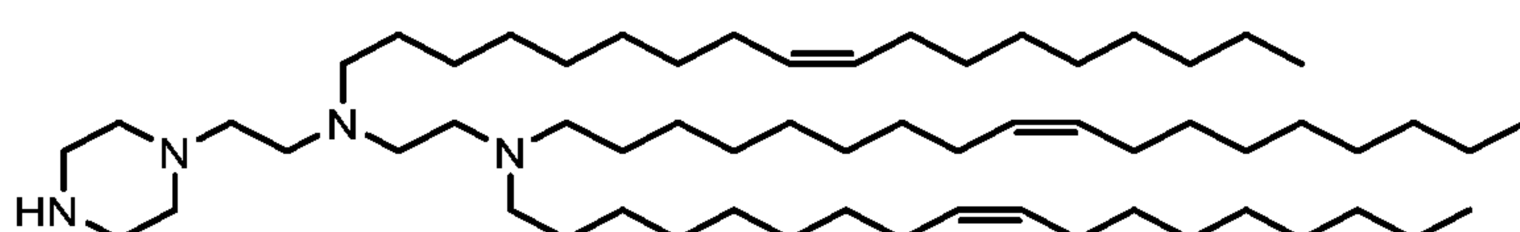
20 (Compound 271),
