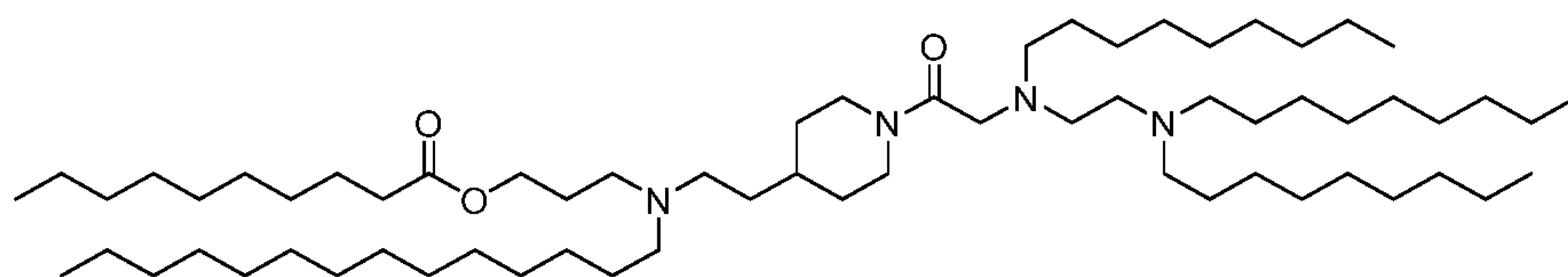
(Compound 324),
