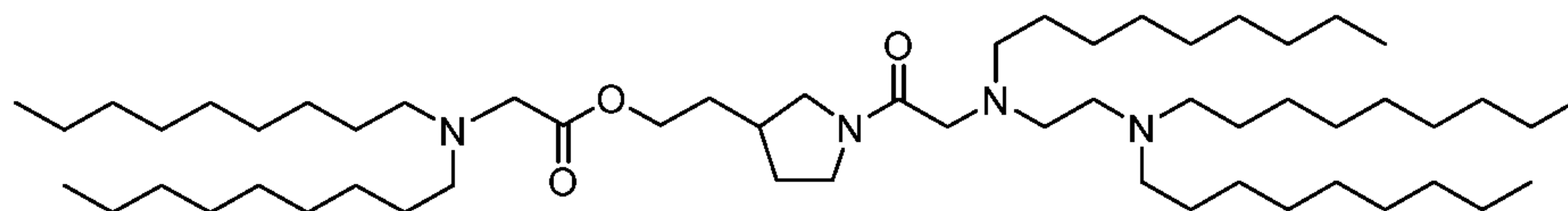
(Compound 335),
