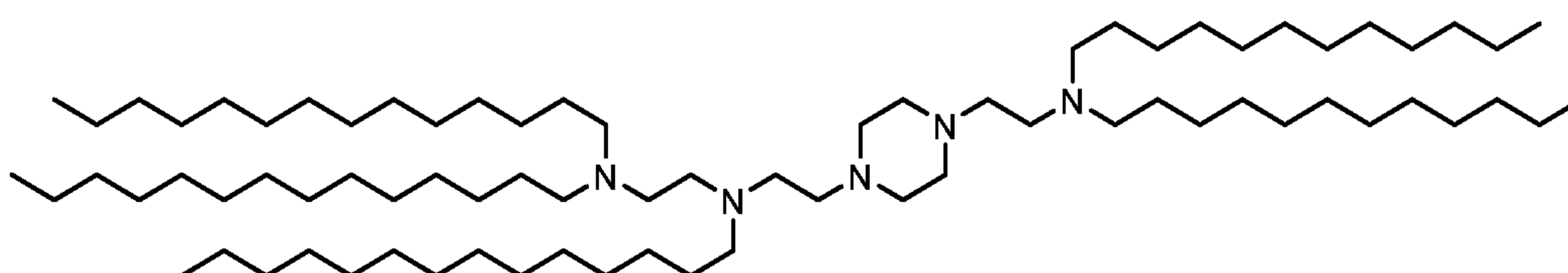
(Compound 263),
