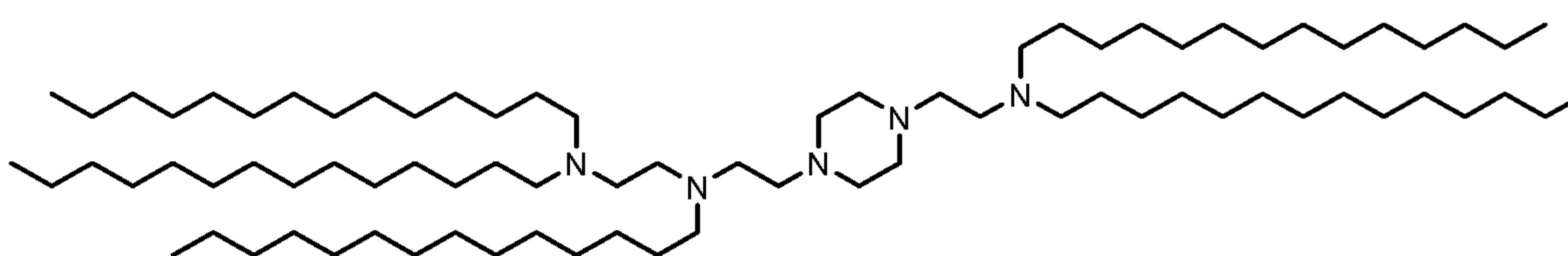
(Compound 264),
