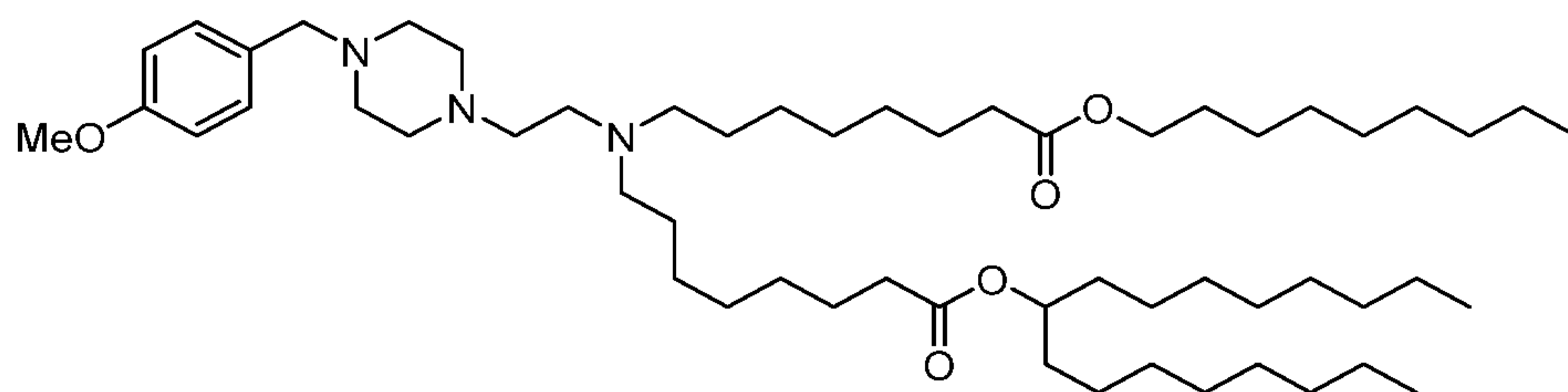
(Compound 102),
