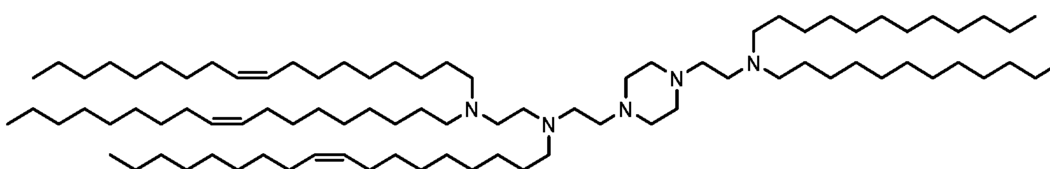
(Compound 265), and
