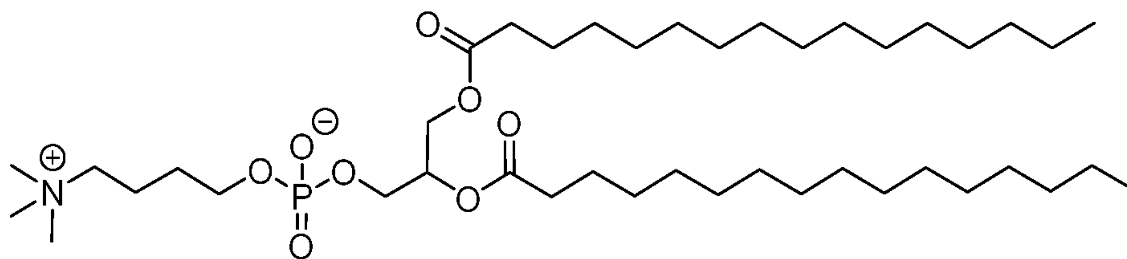
(Compound 413)
