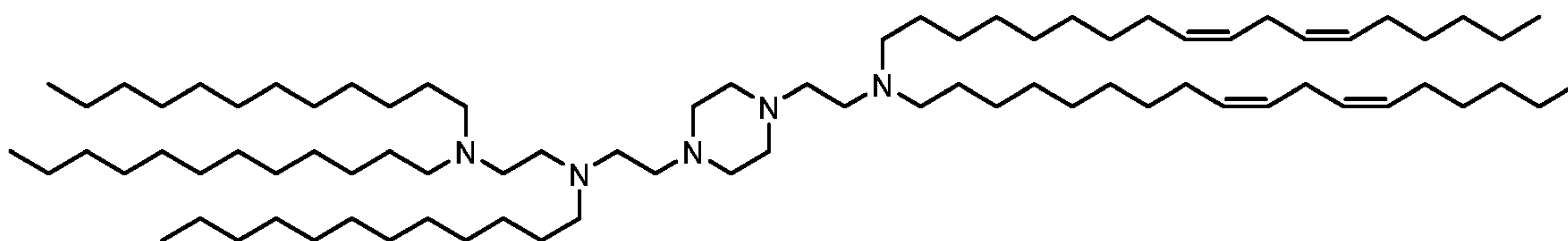
(Compound 261),
