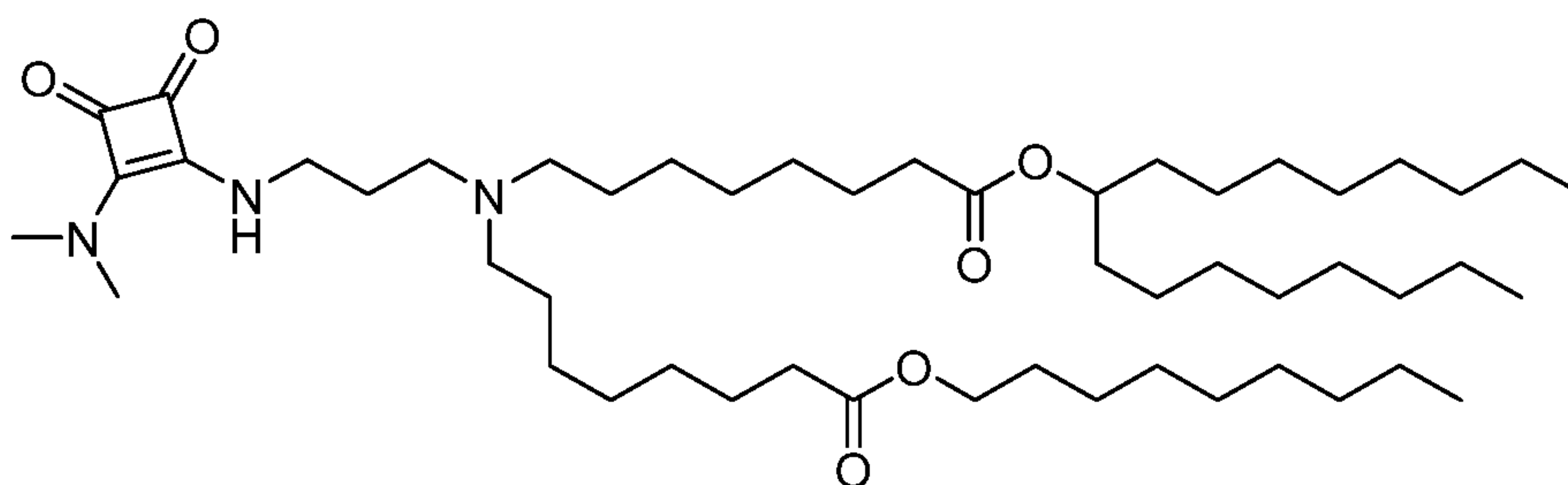
(Compound 169),
