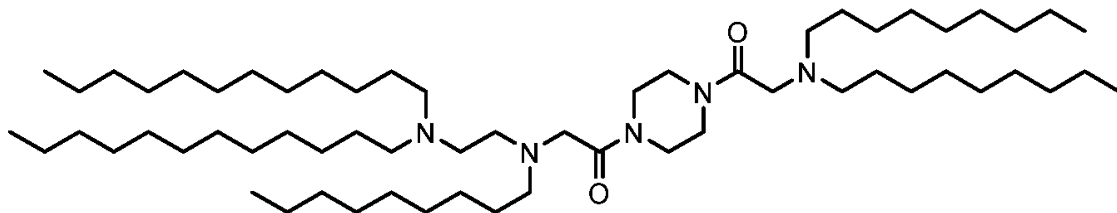
(Compound 238),
