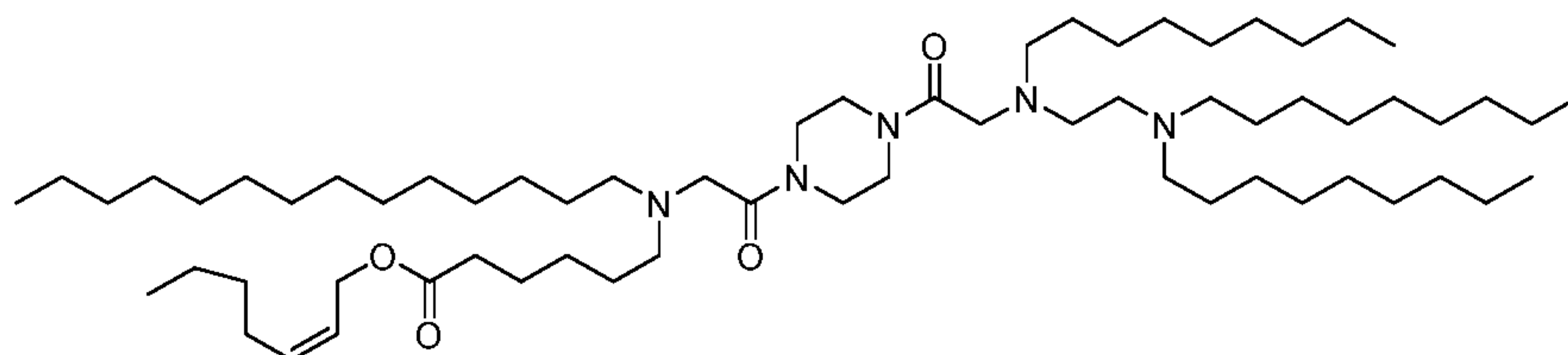
(Compound 340), and
