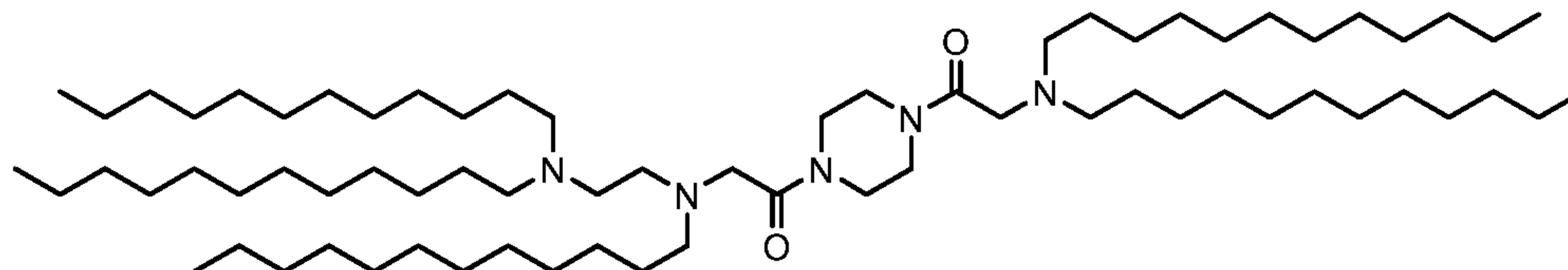
(Compound 243),
