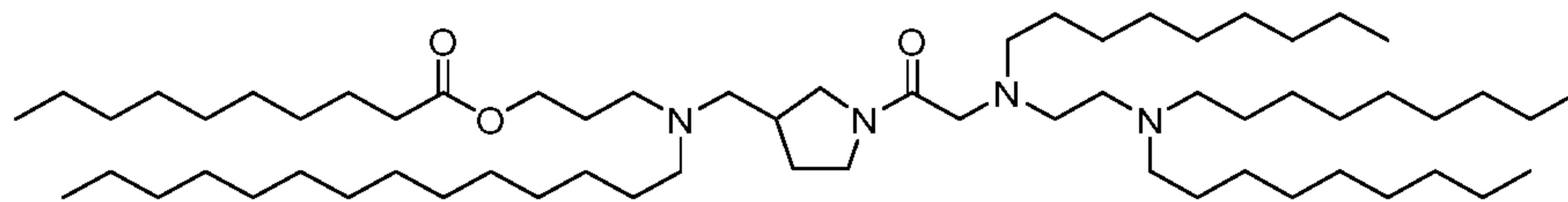
(Compound 330),
