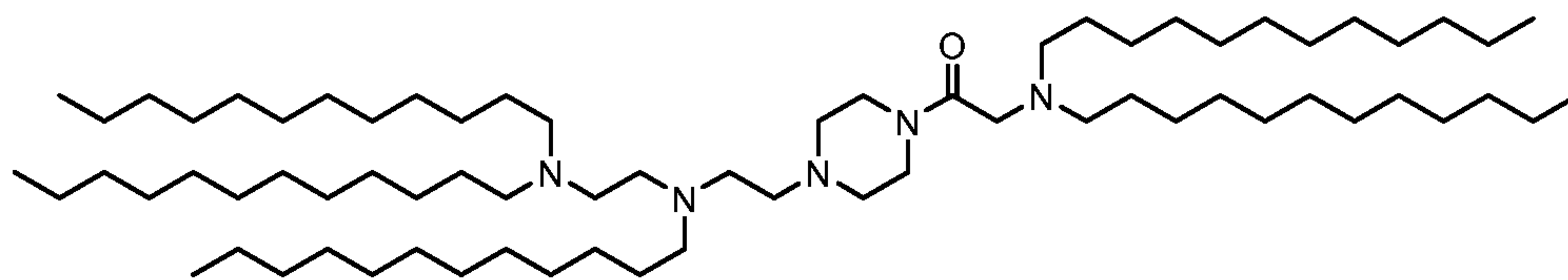
(Compound 235),
