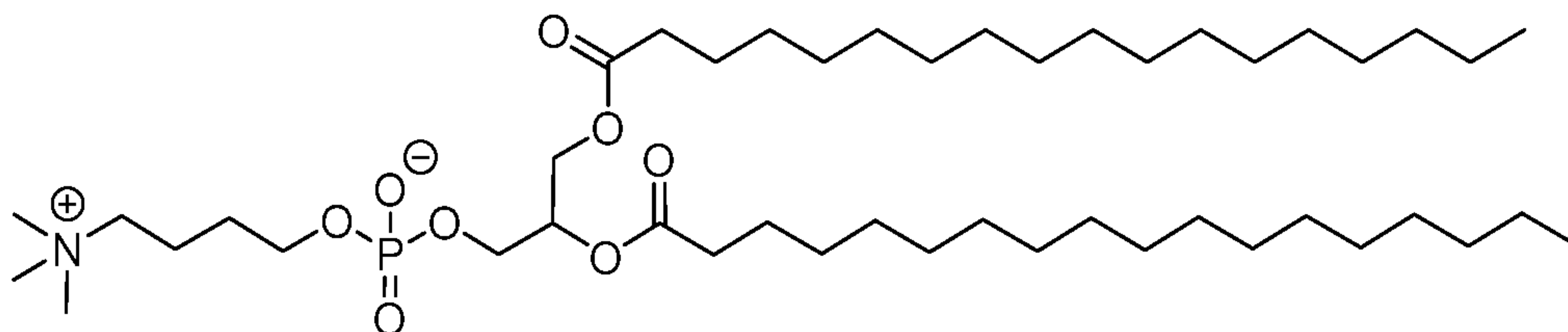
(Compound 414),
