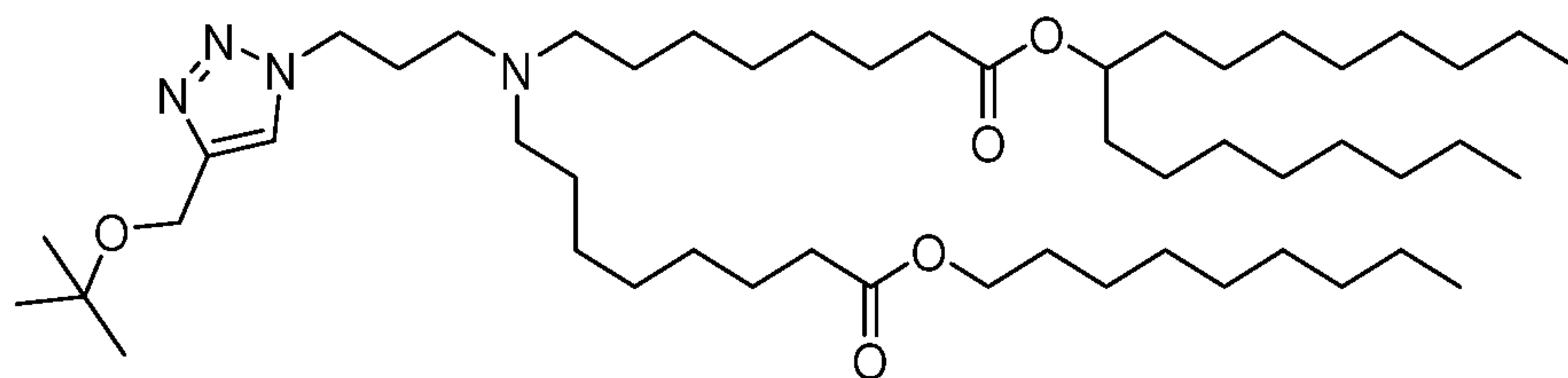
(Compound 177),
