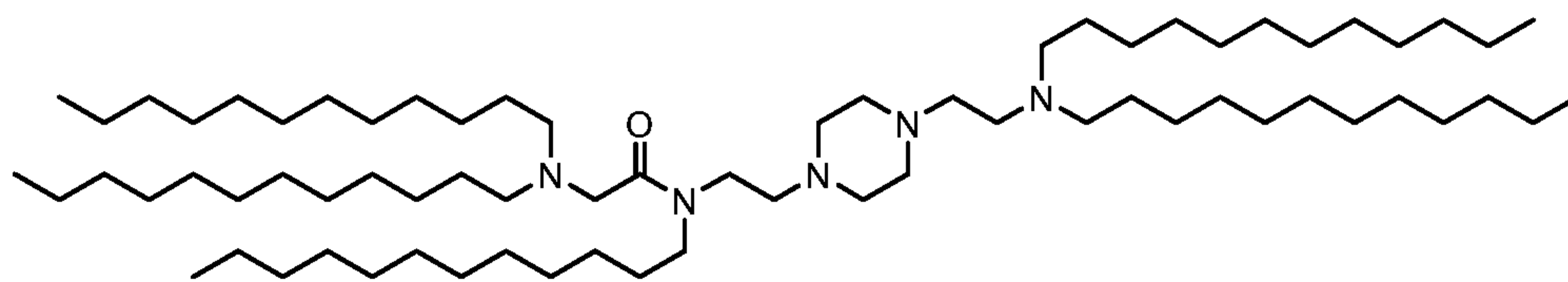
(Compound 233),
