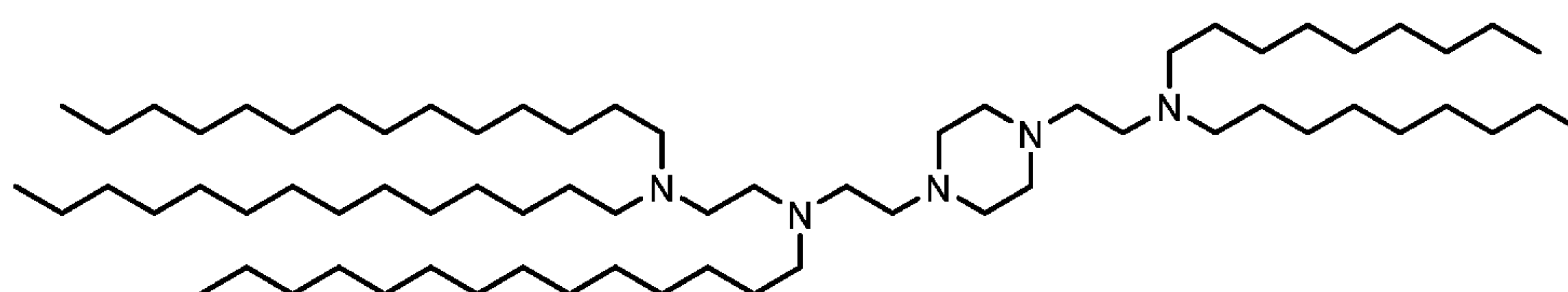
(Compound 262),
