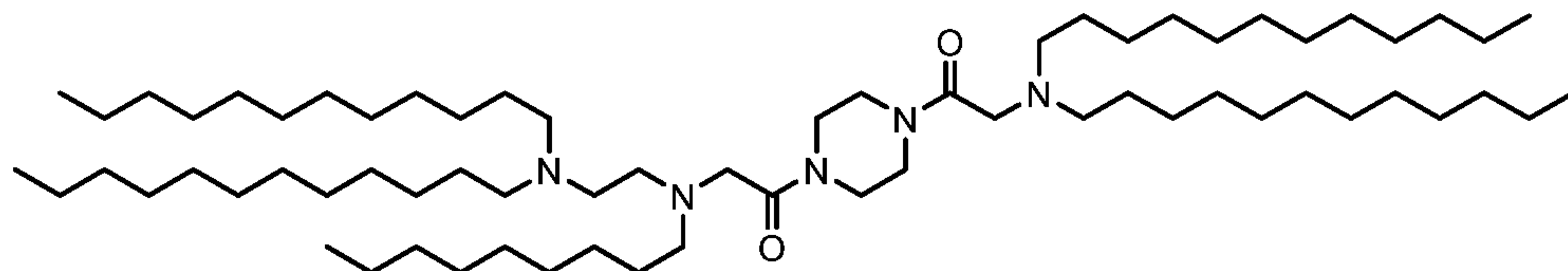
(Compound 242),
