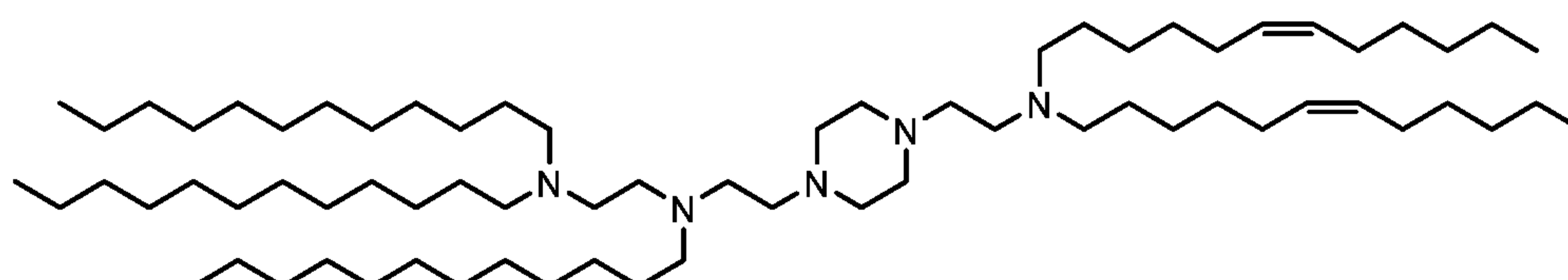
(Compound 257),
