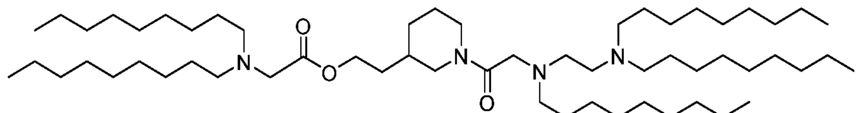
(Compound 333),
