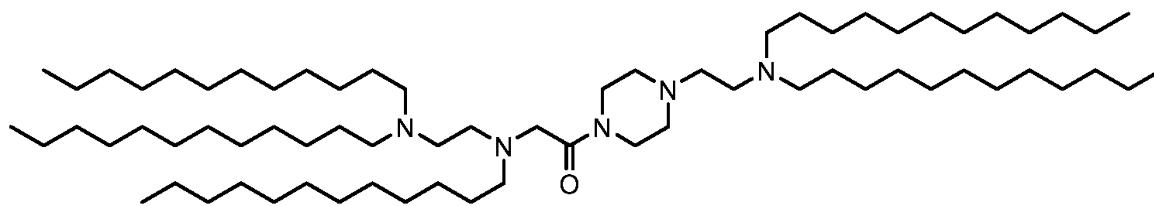
(Compound 234),
