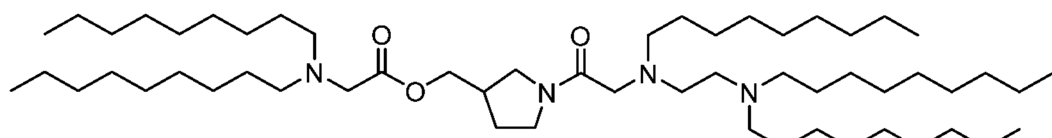
(Compound 334),
