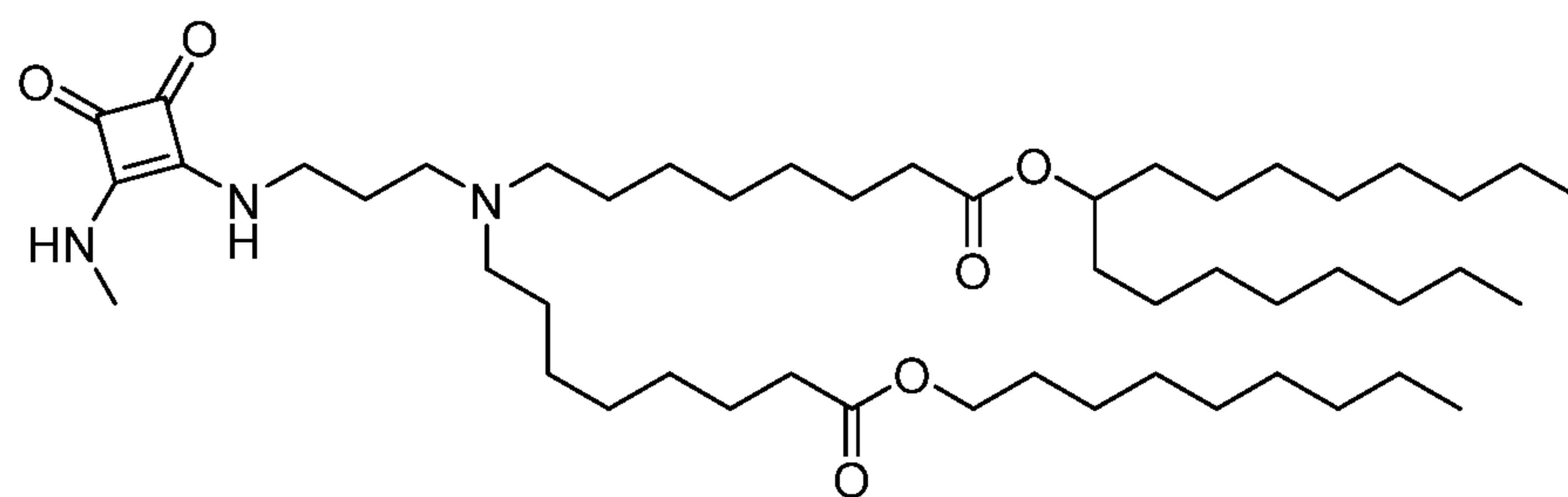
(Compound 182),
