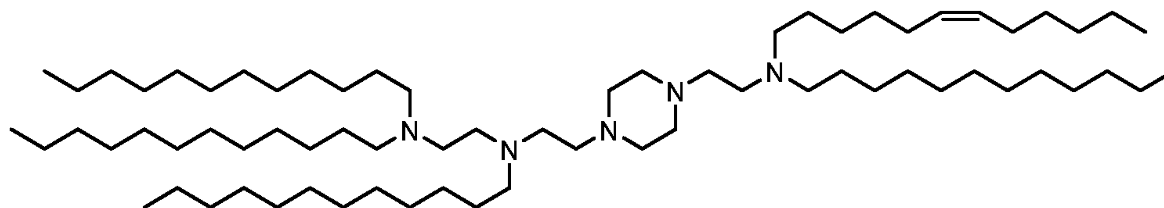
(Compound 256),
