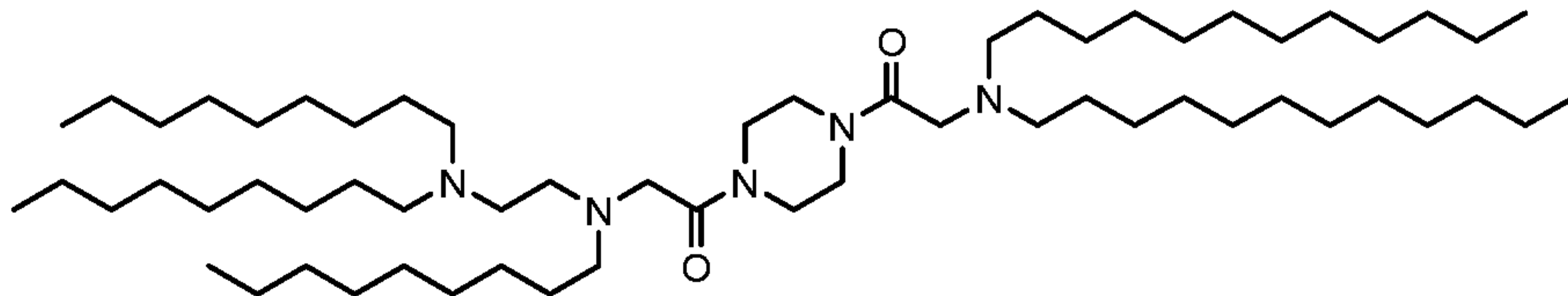
(Compound 240),
