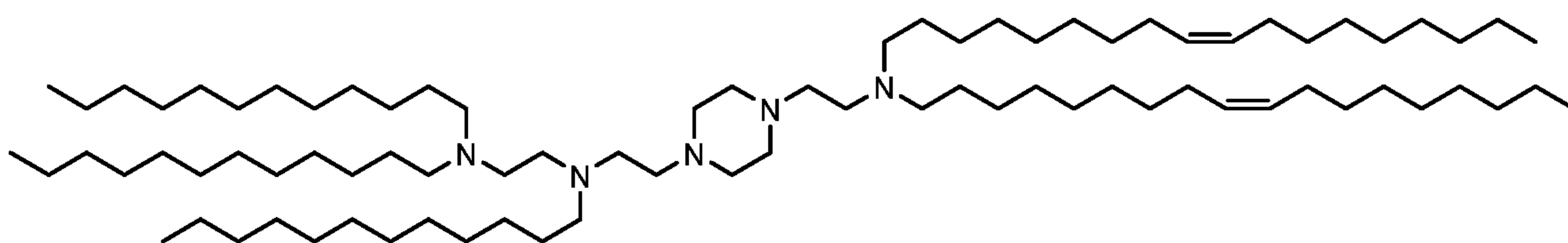
(Compound 260),
