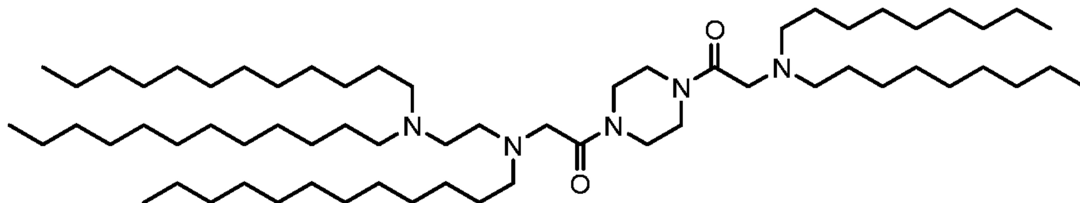
(Compound 239),
