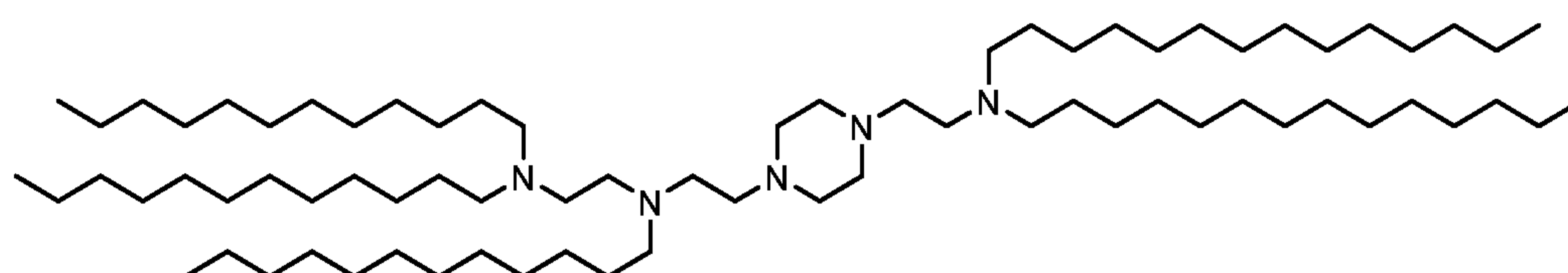
(Compound 258),
