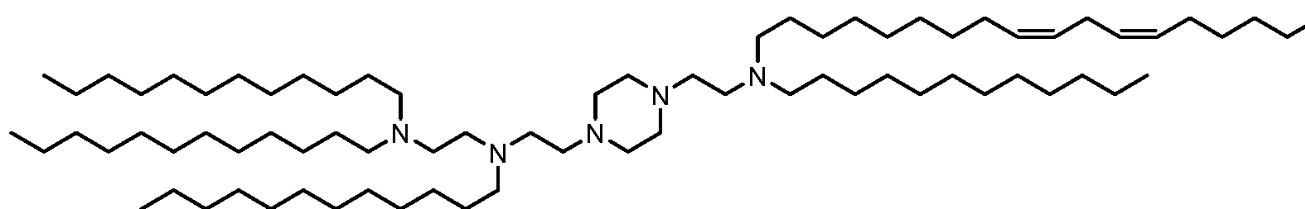
(Compound 259),
