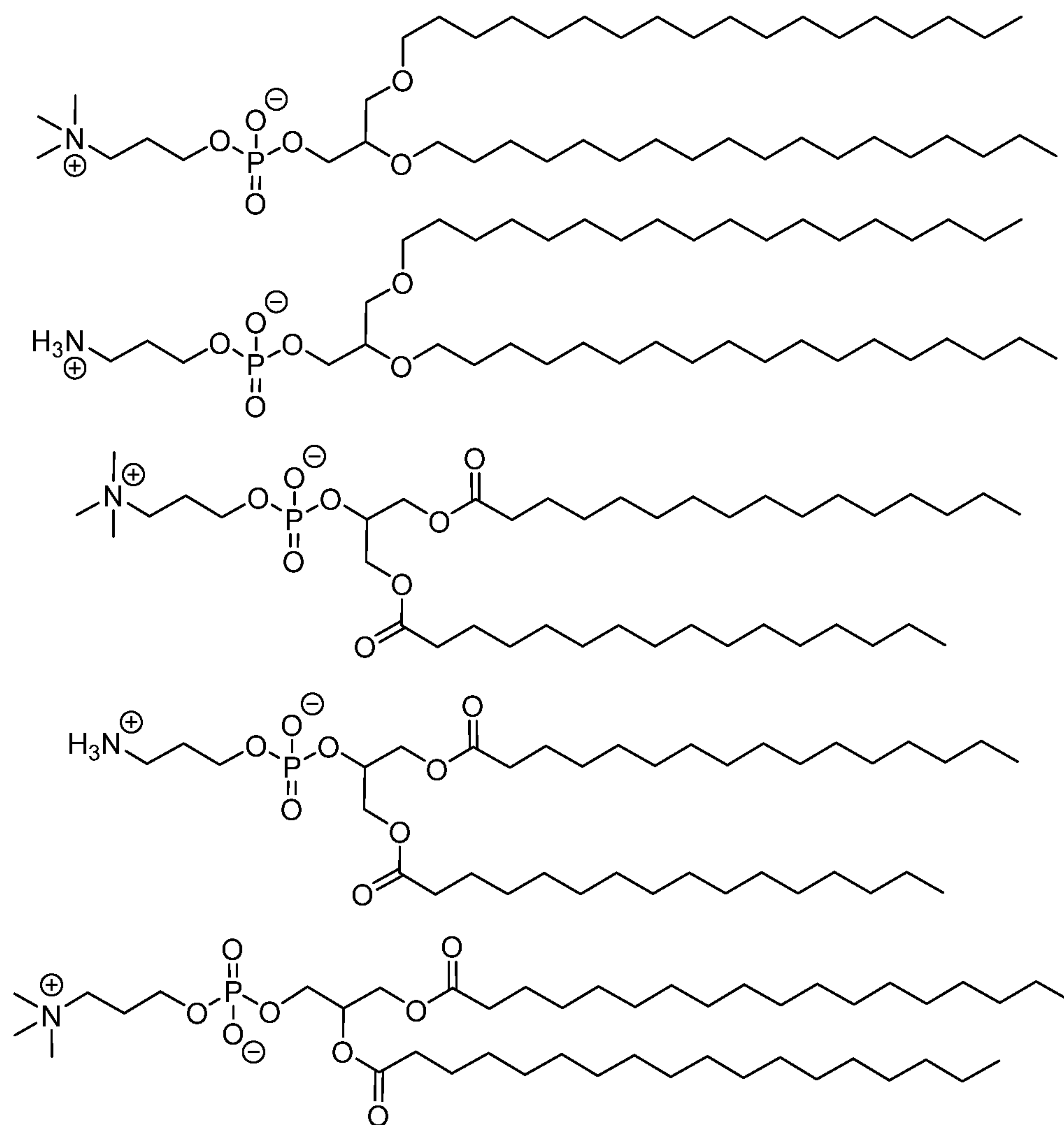
(Compound 411)
