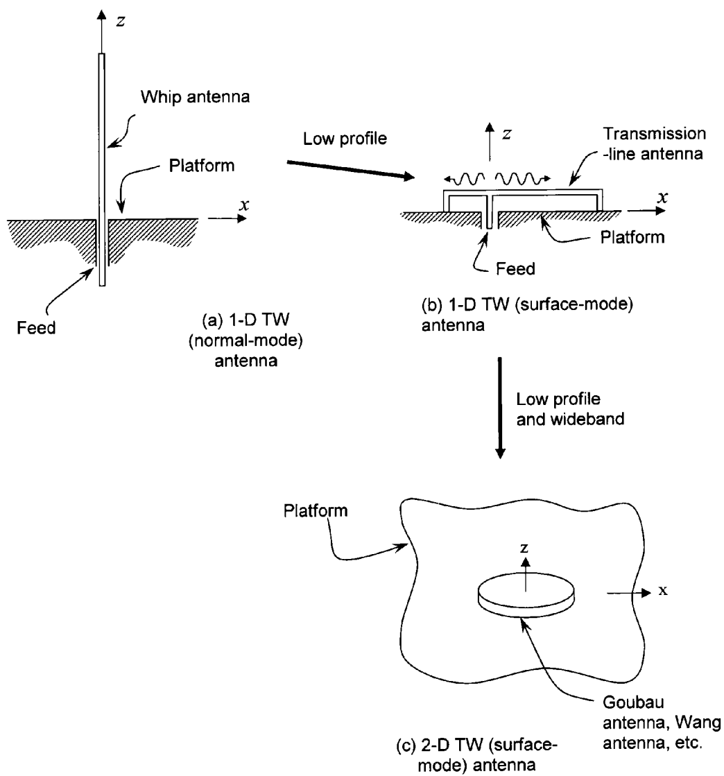
FIG. 1 (Prior Art)
