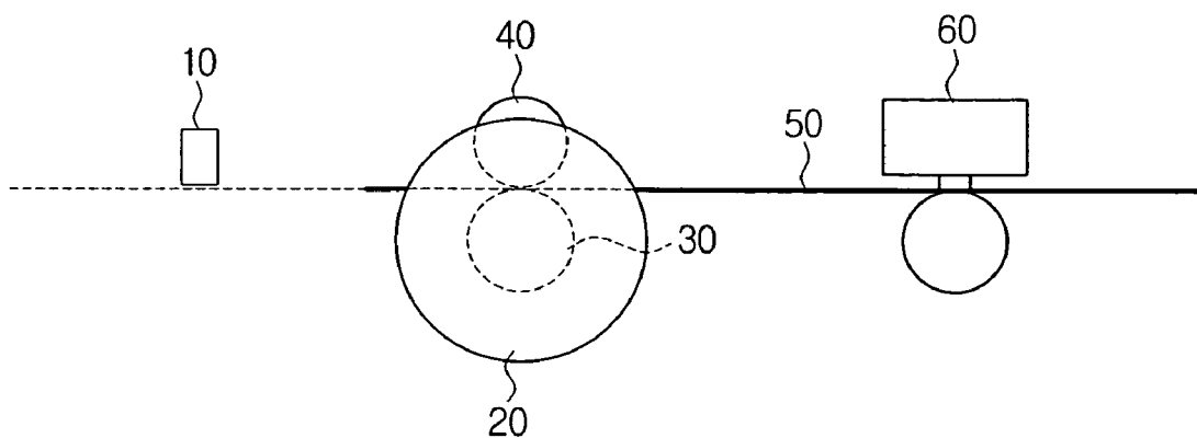
FIG. 1 (PRIOR ART)
