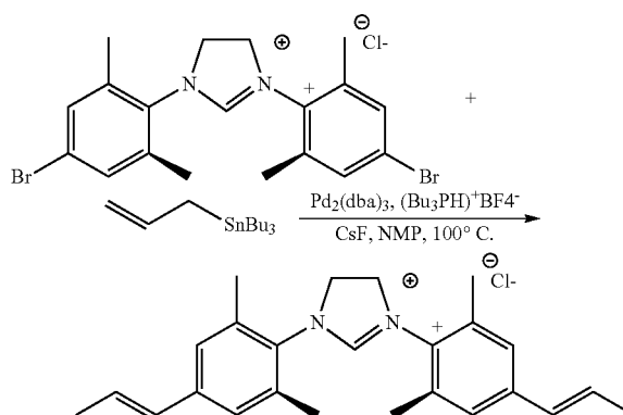
Reaction Scheme 3
