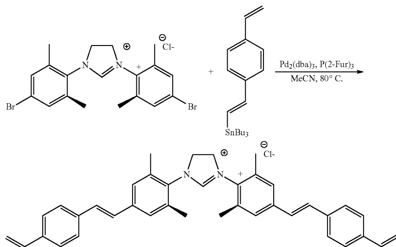
Reaction Scheme 6
