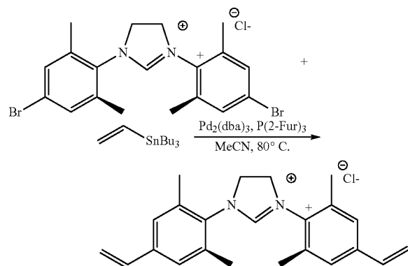
Reaction Scheme 2
