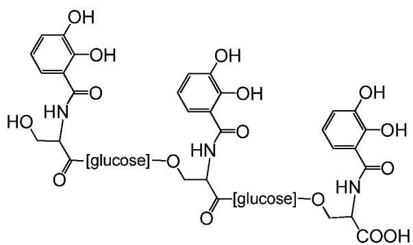
salmochelin 2
