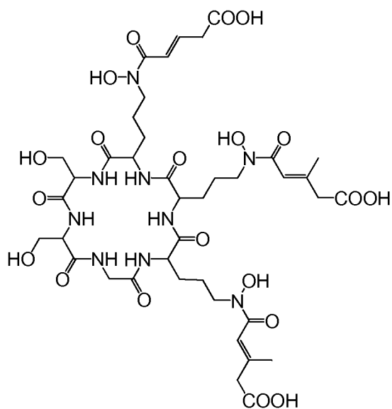
desferrichrome A
