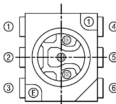
PIN CONNECTIONS
