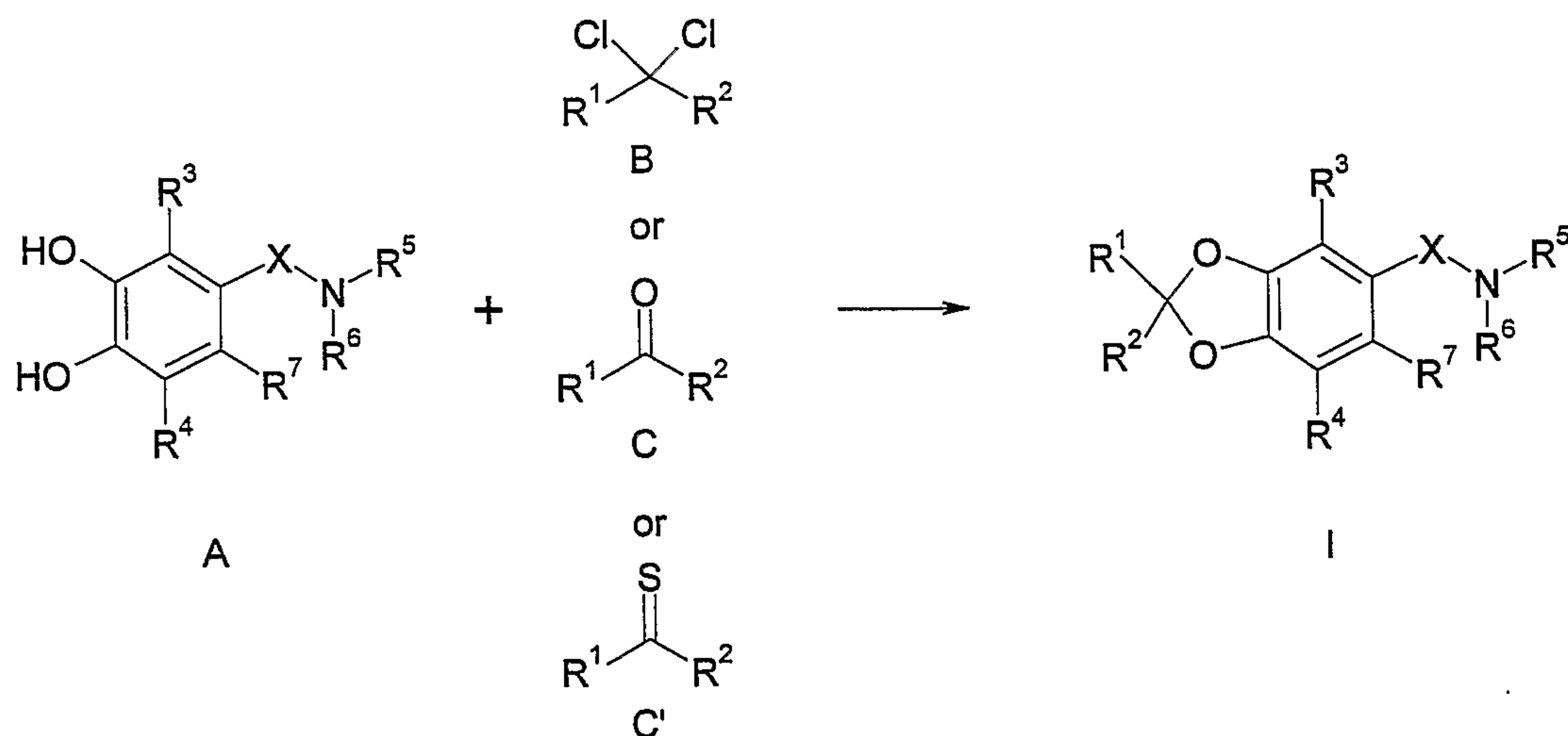
Scheme 1:
