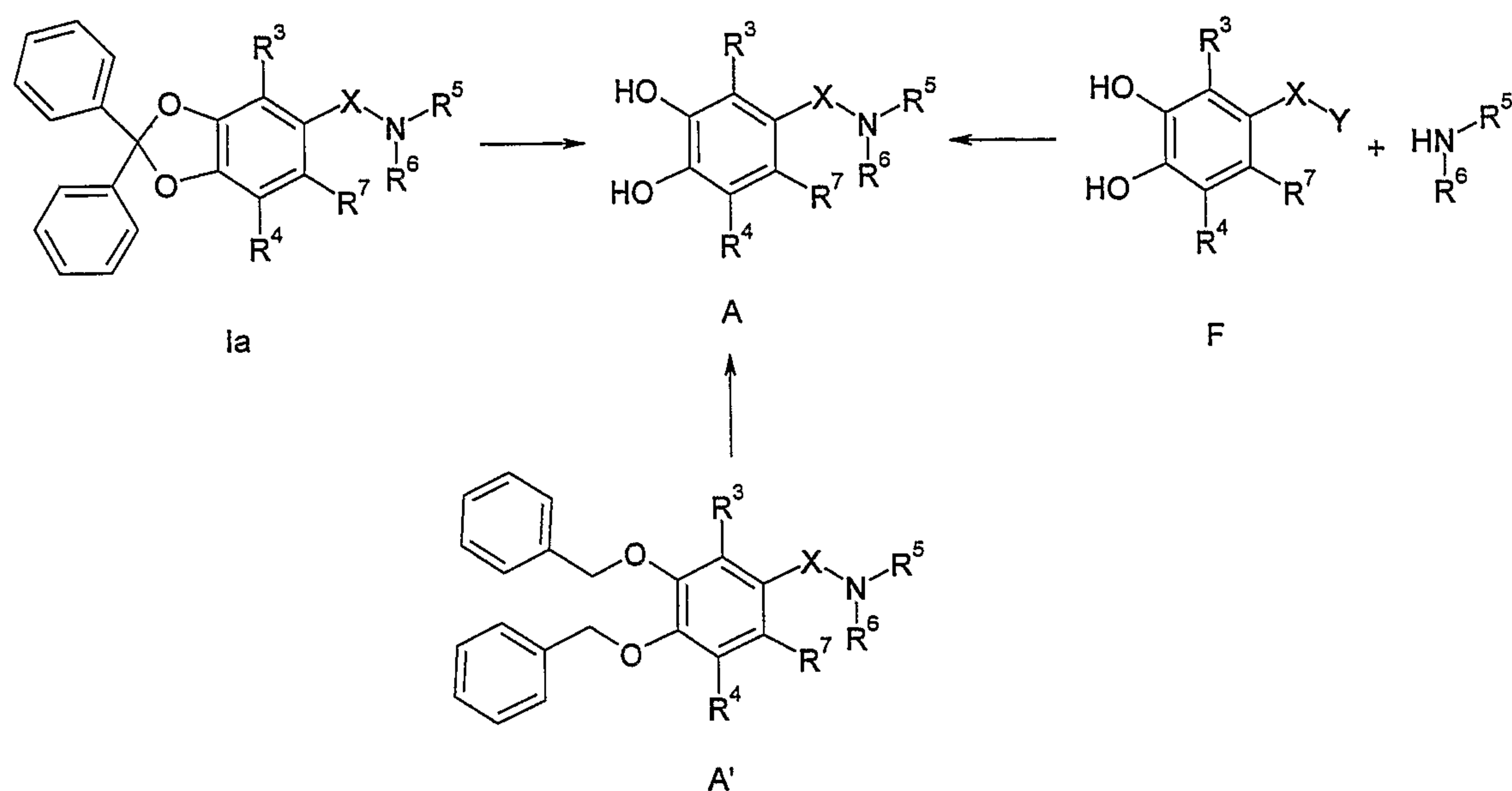
Scheme 3:
