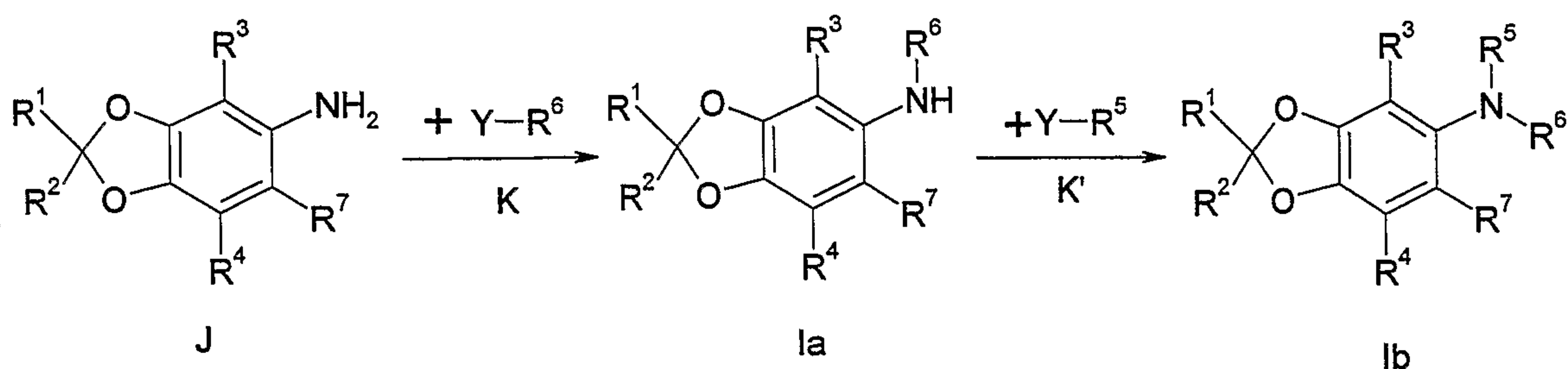
Scheme 5:
