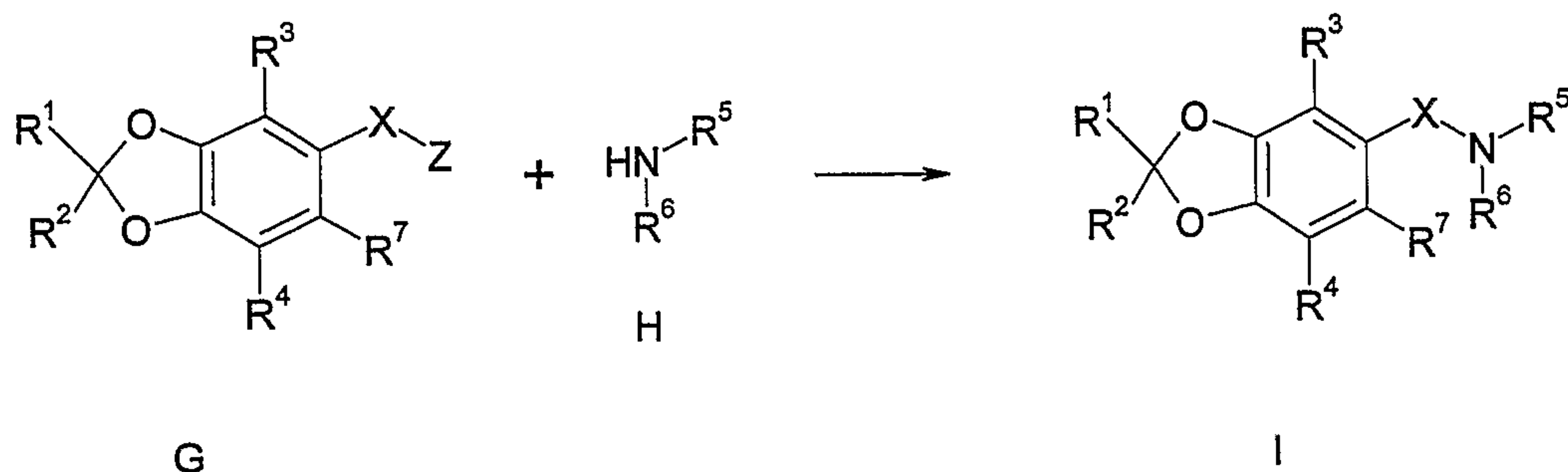
Scheme 4:
