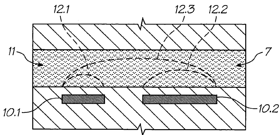
FIG. 52 (PRIOR ART)
