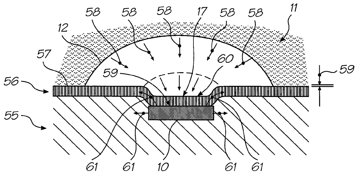
FIG. 47 (PRIOR ART)
