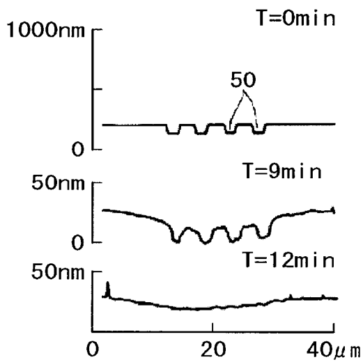
POLISHING ON SURFACE HAVING DEPRESSIONS
