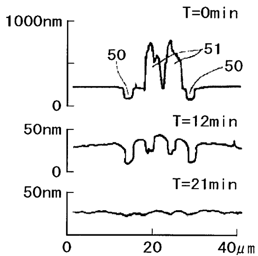
POLISHING ON FILLED-UP SURFACE
