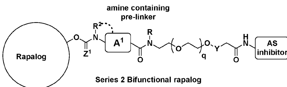
Scheme 2. Series 2 bifunctional rapalogs.
