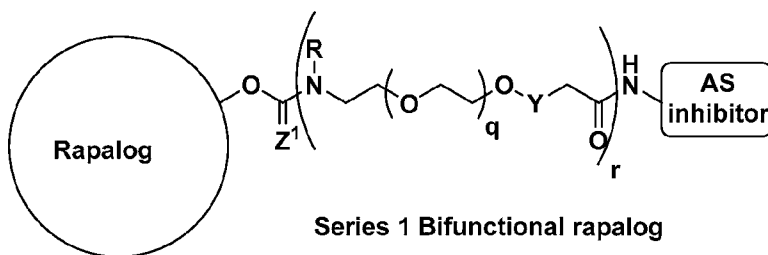
Scheme 1. Series 1 bifunctional rapalogs.
