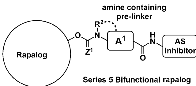
Scheme 5. Series 5 bifunctional rapalogs
