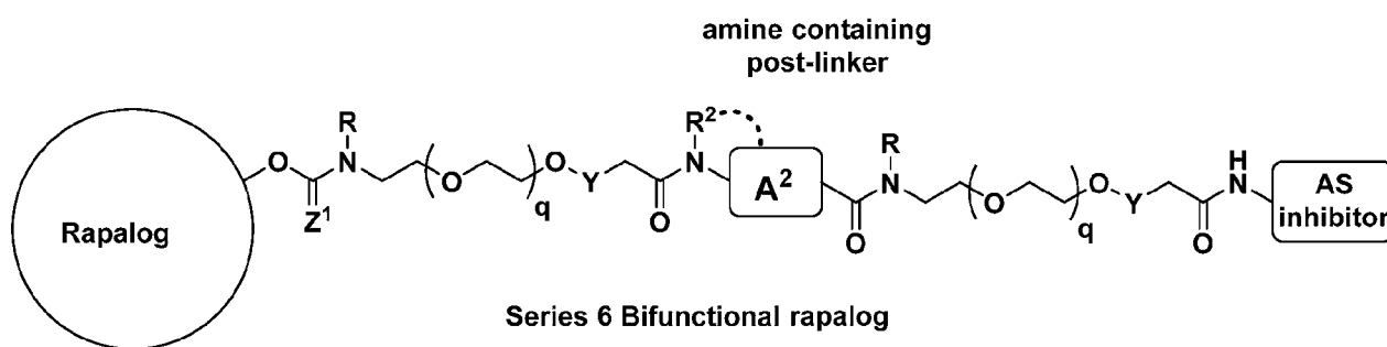
Scheme 6. Series 6 bifunctional rapalogs.
