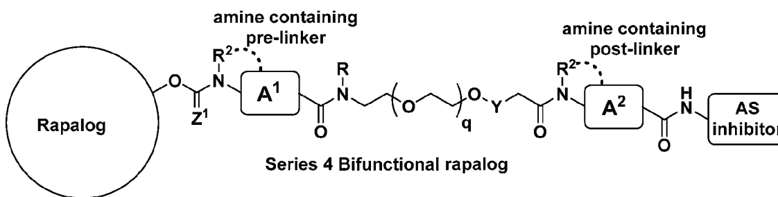
Scheme 4. Series 4 bifunctional rapalogs
