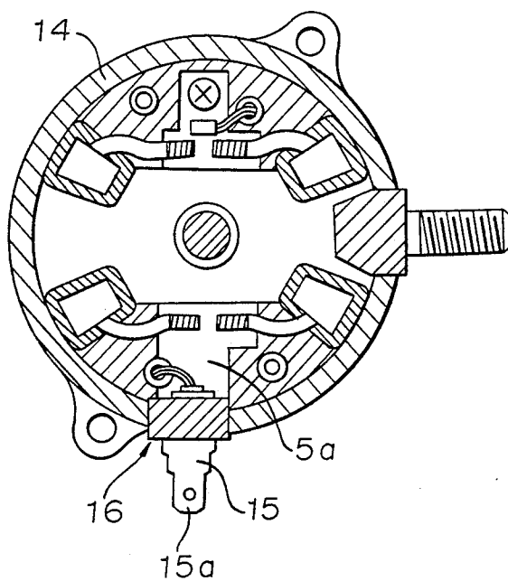
FIGURE 7 PRIOR ART
