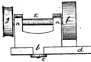
Fig. 1. Rear Elevation.
