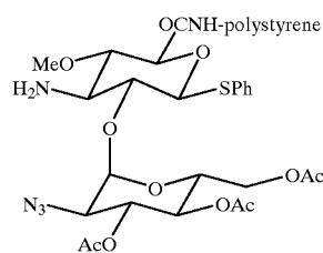
Phenyl 2-O-(2-azido-2-deoxy-3,4,6-tri-O-acetyl- \alpha -D-glucopyranosyl)-(1 \rightarrow 2)- 3-amino-3-deoxy-4-methoxy-1-thio- \beta -D-glucopyranosiduronic acid
