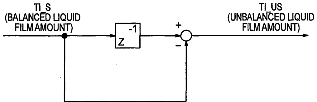
<EMBODIMENTS 5, 6> FIG. 47 <UNBALANCED LIQUID FILM AMOUNT CALCULATION UNIT>
