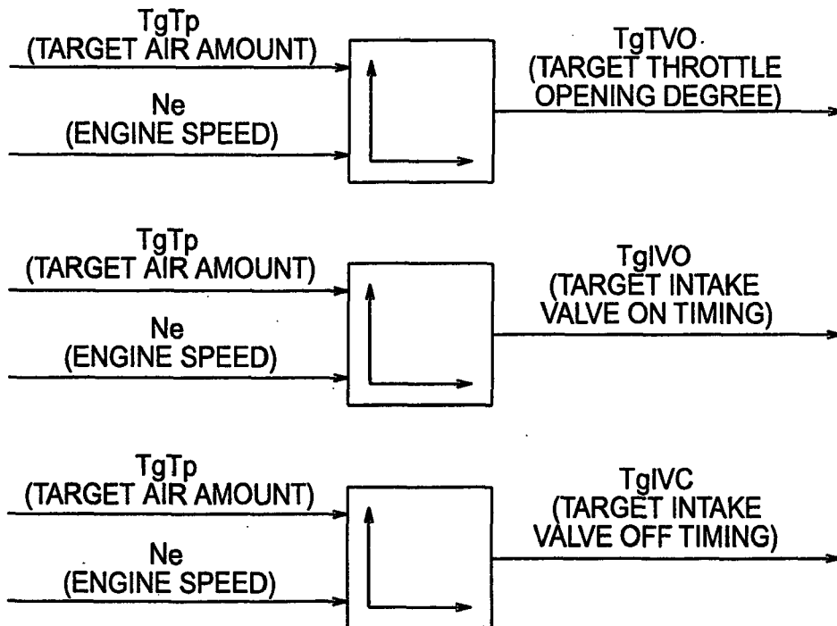
FIG. 36 < EMBODIMENTS 1 TO 4 > < TARGET THROTTLE OPENING DEGREE/INTAKE VALVE ON/OFF TIMING CALCULATION UNIT >
