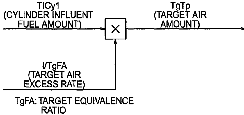
FIG. 35 < EMBODIMENT 1 > < TARGET AIR AMOUNT CALCULATION UNIT >
