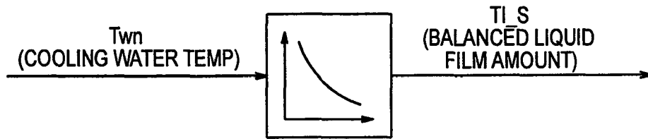
<EMBODIMENT 5> FIG. 46 <BALANCED LIQUID FILM AMOUNT CALCULATION UNIT>
