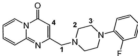
2-((4-(2-fluorophenyl)piperazin-1-yl)methyl)-4H-pyrido[1,2-a]pyrimidin-4-one
