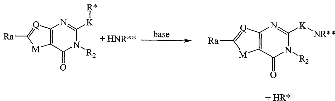
Scheme I
