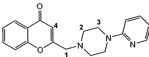
2-((4-(pyridin-2-yl)piperazin-1-yl)methyl)-4H-chromen-4-one
