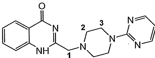
2-((4-(pyrimidin-2-yl)piperazin-1-yl)methyl)quinazolin-4(1H)-one
