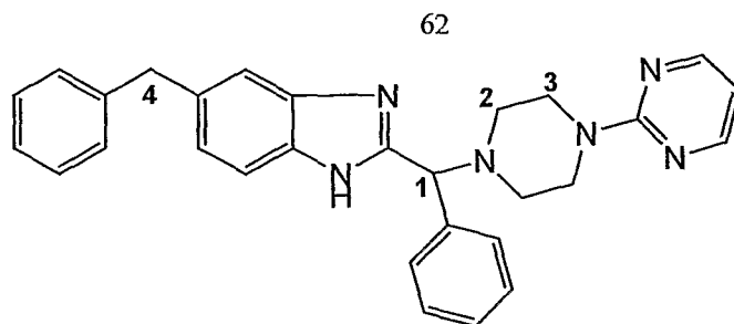
5-benzyl-2-(phenyl(4-(pyrimidin-2-yl)piperazin-1-yl)methyl)-1H-benzo[d]imidazole
