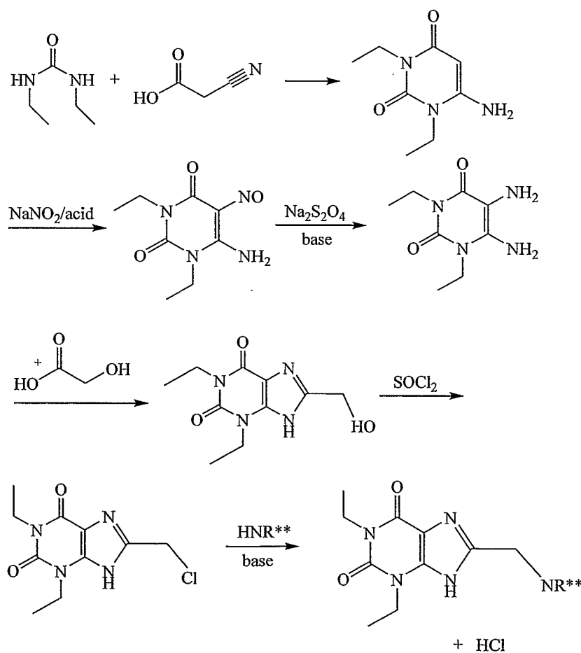
Scheme VIb
