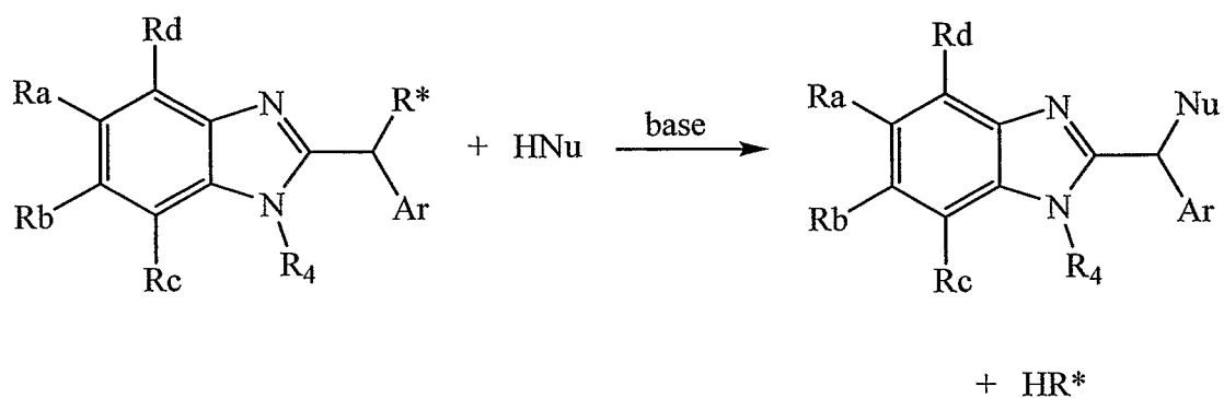
Scheme IV
