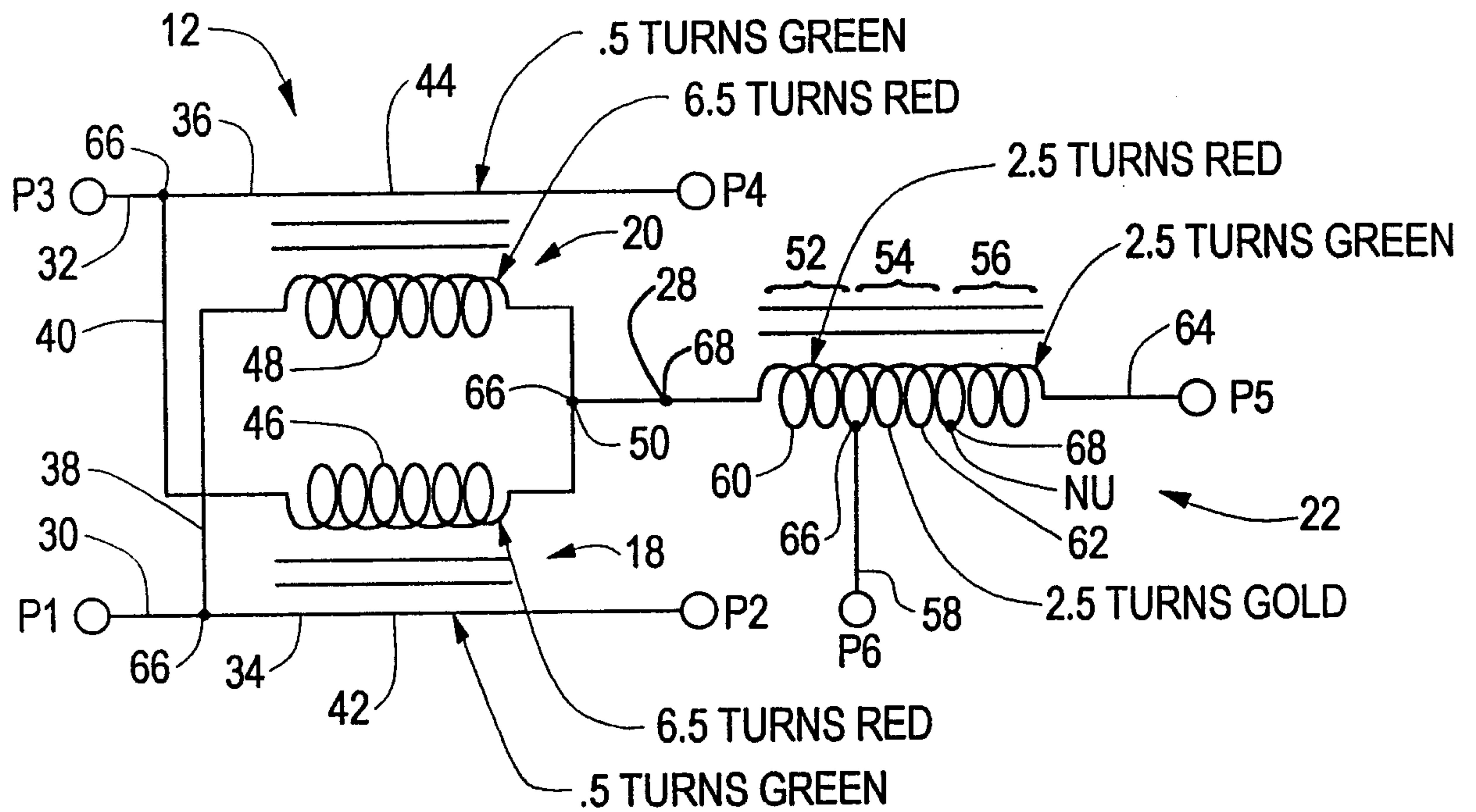
SCHEMATIC
