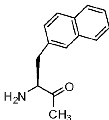
2-(2-naphthyl)-L-alanine (Nal(2))
