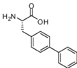
2-L-biphenyl-alanine (Bip)
