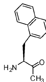
2-(1-naphthyl)-L-alanine (Nal(1))
