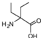
2,2-diethylglycine (Deg)
