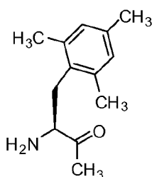
2,4,6-trimethyl-L-phenylalanine (Tmp)
