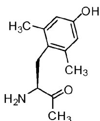
2,6-dimethyl-L-tyrosine (Dmt)
