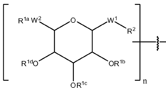
Formula 3-I
