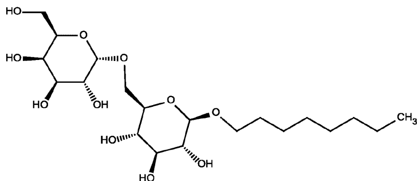
1-Octyl beta-D-melibioside
