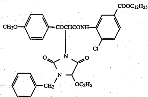
Coupler EX-1
