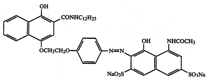
Coupler EX-2
