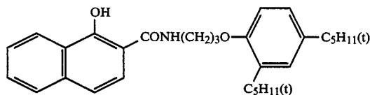
Coupler D-3
