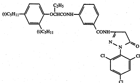
Coupler Y-1
