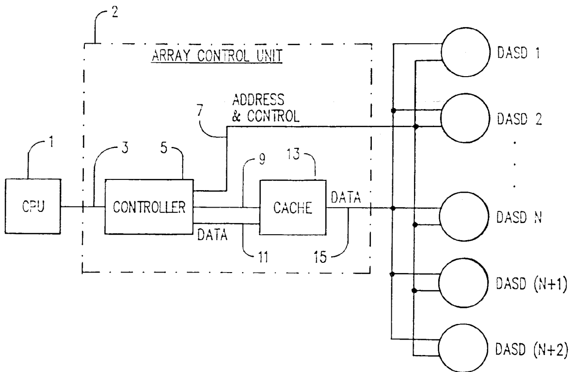
SYNCHRONOUS DASD ARRAY Figure 8
