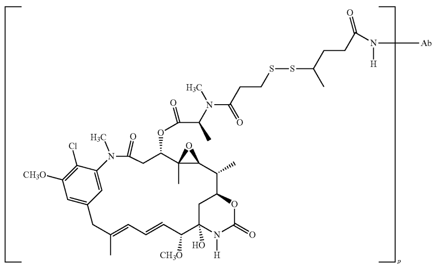
Ab-SPP-DM1
