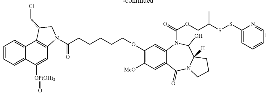
CBI-PBD-(phosphate)-2-propyl pyridyl disulfide 82
