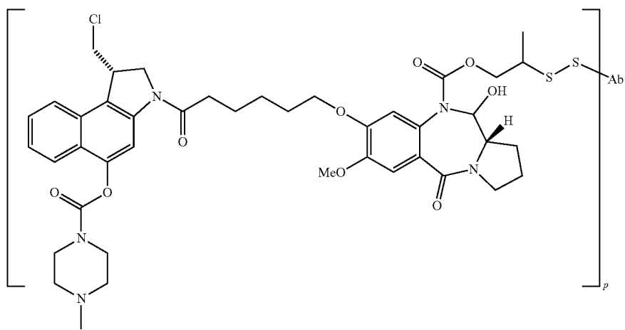
CBI-PBD (piperazine-carbamate prodrug)-disulfide-Ab
