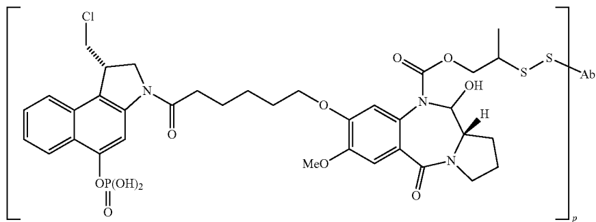
CBI-PBD (phosphate)-disulfide-Ab
