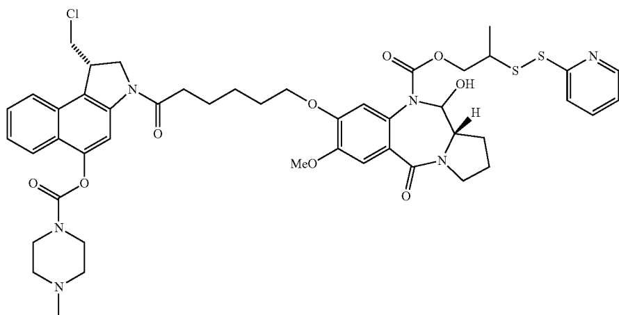
CBI-PBD (piperazine-carbamate prodrug)- 2-propyl pyridyl disulfide 81
