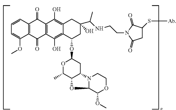
PNU-159682-maleimide-Ac
