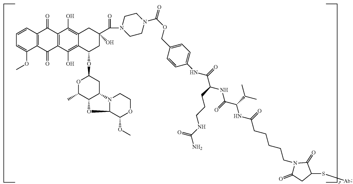
PNU-159682-val-cit-PAB-Ab
