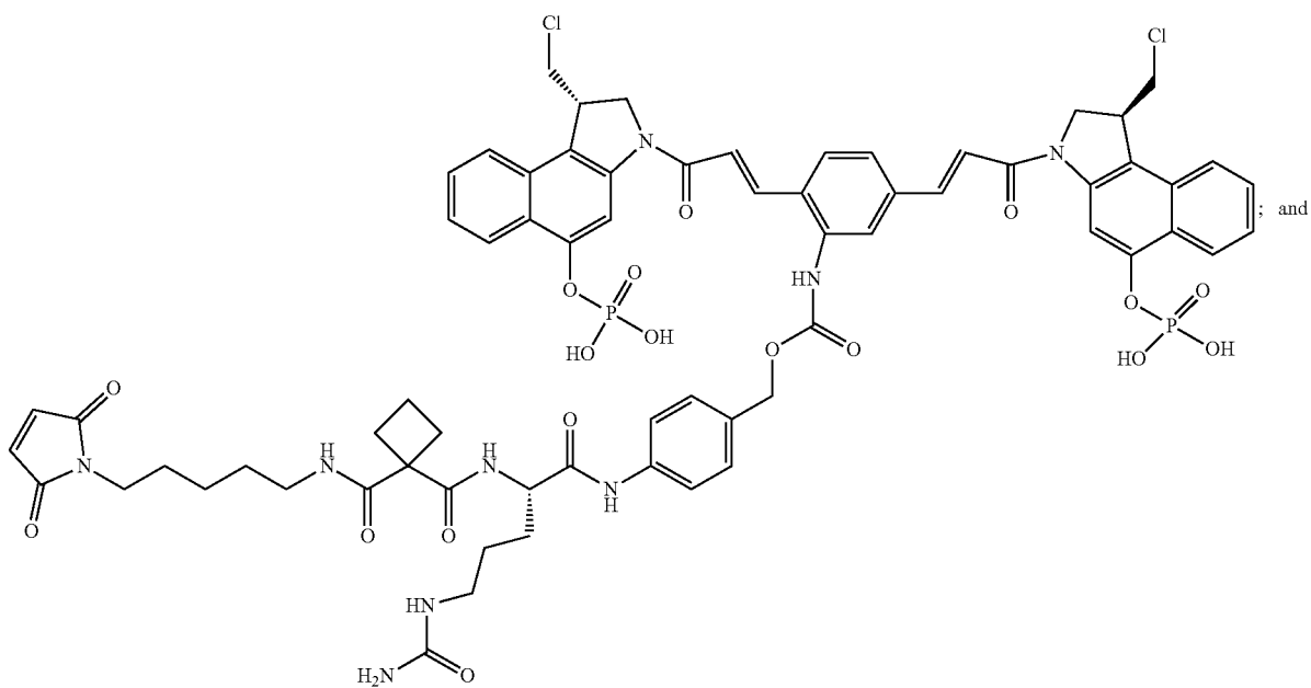
CBI-CBI (phosphate)-peptidomimetic PAB linker 89
