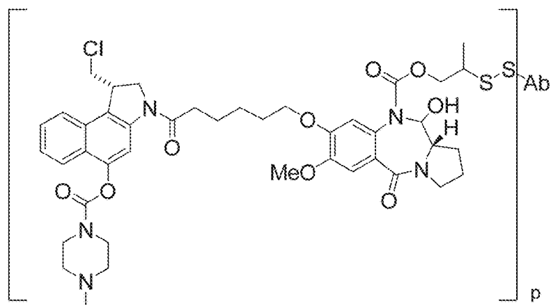
FIG. 12C: thio-hu7C2-LC-K149C-disulfide-CBI-PBD
