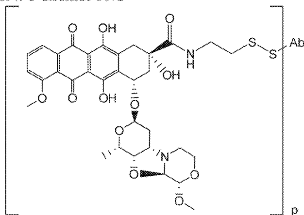
FIG. 12D: thio-hu7C2-LC-K149C-disulfide-PNU
