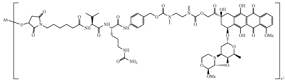
PNU-159682-val-cit-PAB-spacer-Ab
