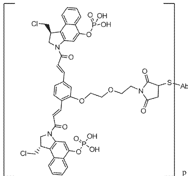
FIG. 12B: thio-hu7C2-LC-K149C-CBI dimer
