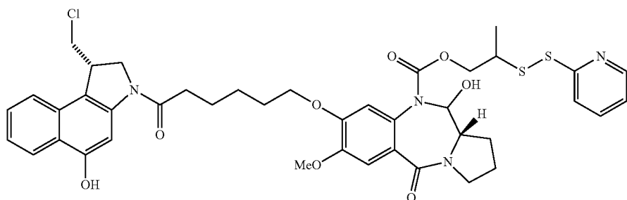
CBI-PBD-2-propyl pyridyl disulfide 83
