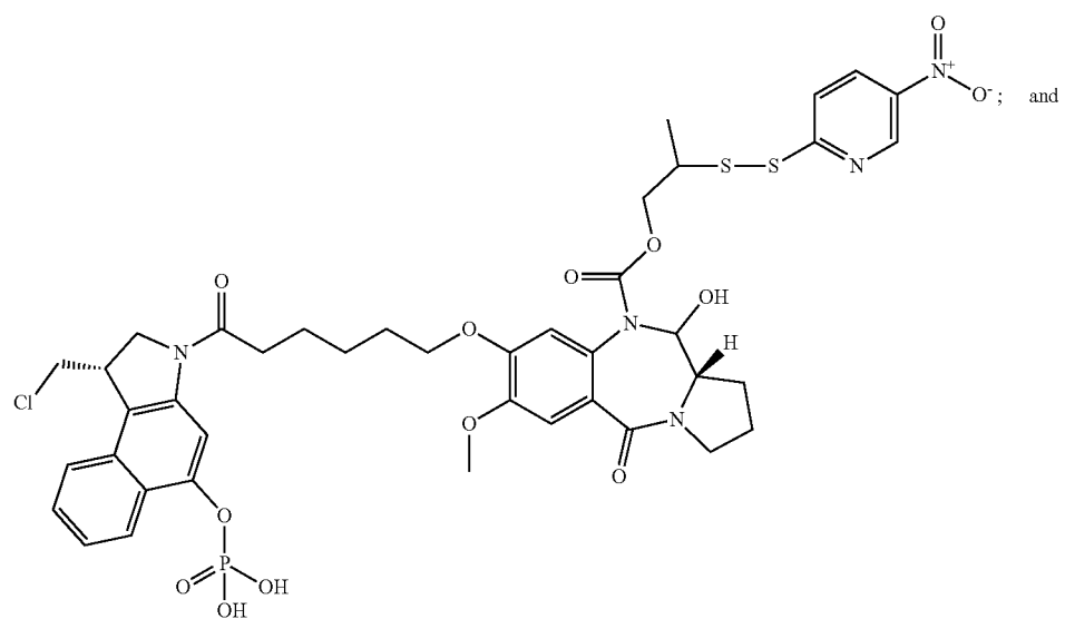
CBI-PBD-(phosphate)-2-propyl, nitropyridyl disulfide 85
