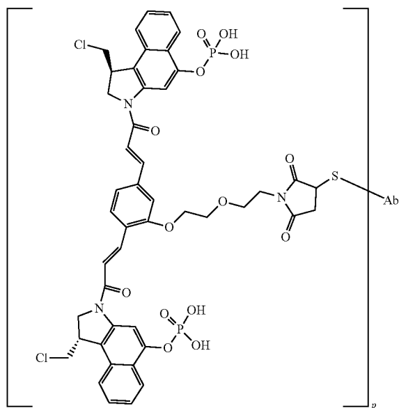
CBI-CBI (phosphate)-acetal-maleimide-Ab
