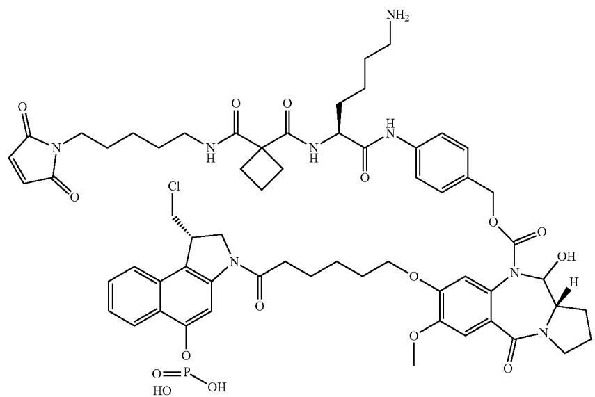
CBI-PBD-(phosphate)-peptidomimetic linker 86
