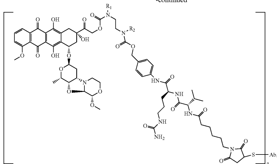
PNU-159682-val-cit-PAB-spacer(R¹R²)-Ab
