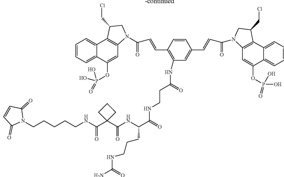
CBI-CBI (phosphate)-peptidomimetic EDA linker 90
