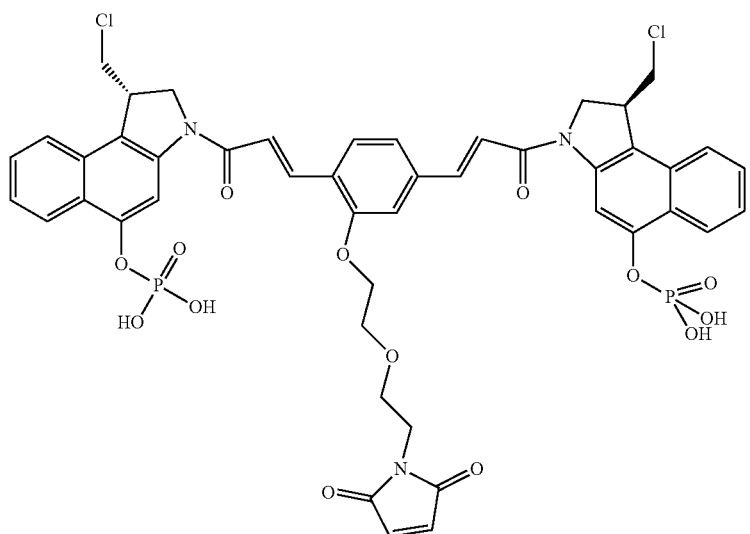
CBI-CBI (phosphate)-acetal-maleimide 78
