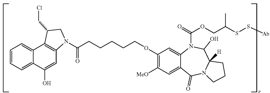
CBI-PBD-disulfide-Ab
