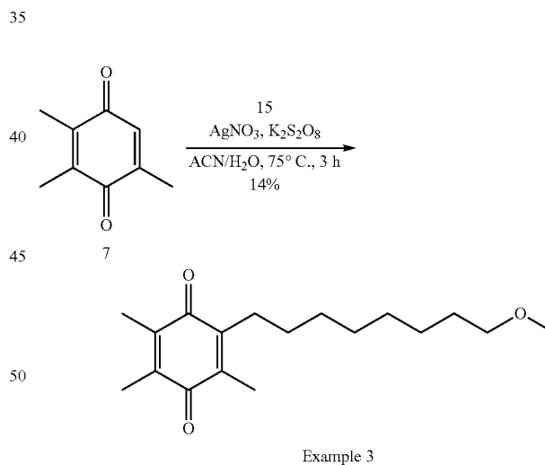
Step 3. 2-(8-methoxyoctyl)-3,5,6-trimethylcyclohexa-2,5-diene-1,4-dione (Example 3)
