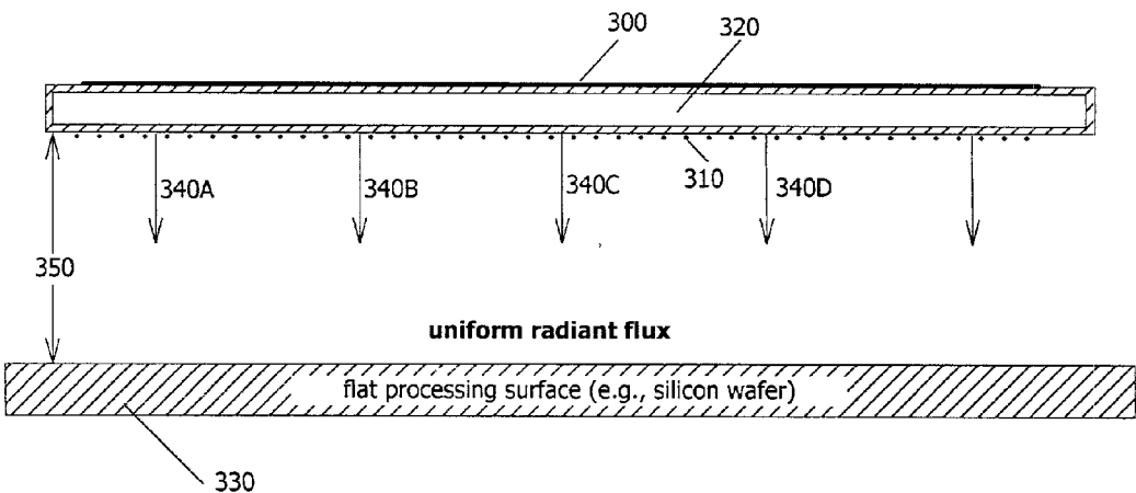
Figure 3 Flat Panel DBD (V)UV light source
