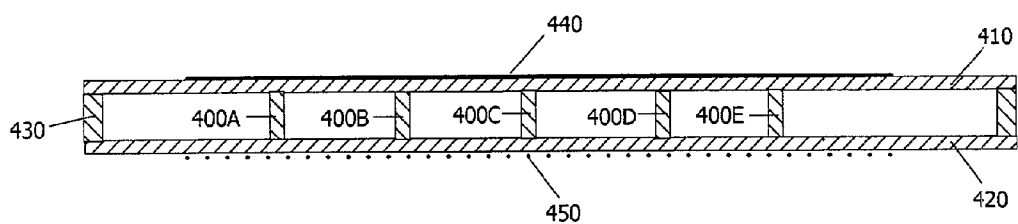
Figure 4a side-on view of stem-stabilized flat panel, large area DBD excimer (V)UV light source
