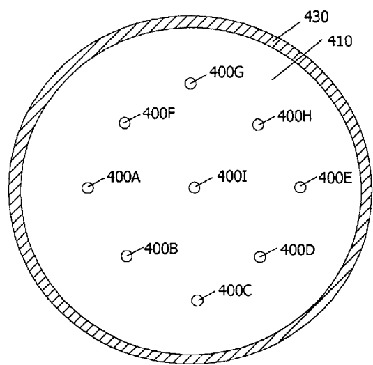
Figure 4b head-on view of stem-stabilized flat panel, large area DBD excimer (V)UV light source
