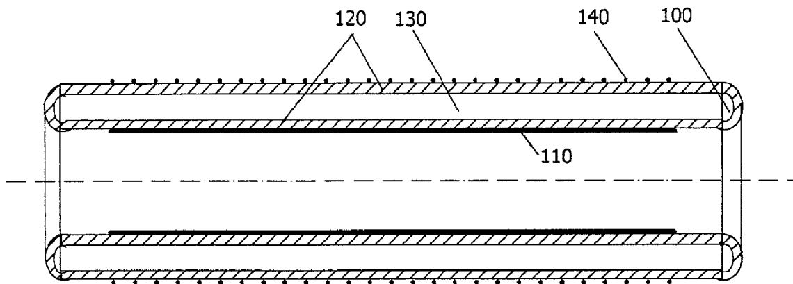
side-on view of typical co-axial DBD lamp
