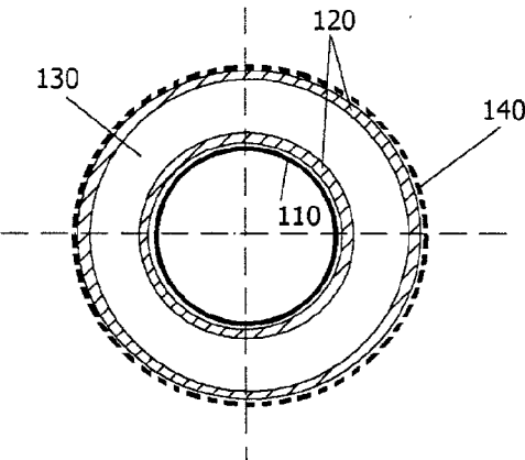
end-on view of typical co-axial DBD lamp
