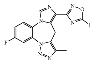
R = Me: Compound 145
