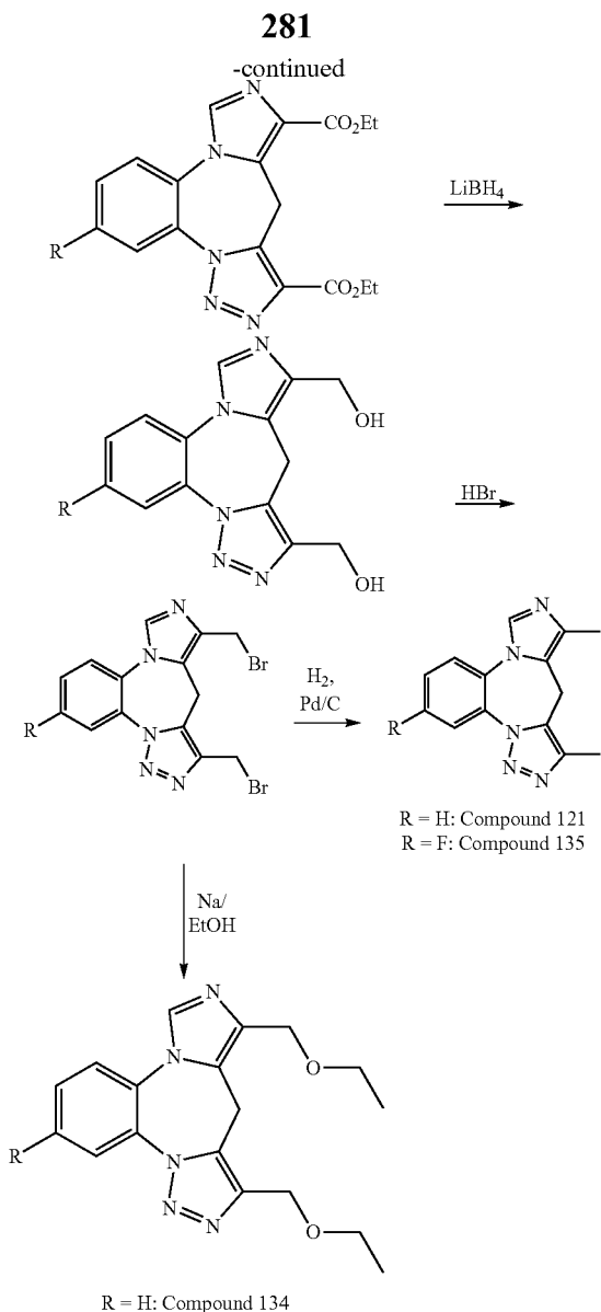
Example 77: Synthesis of Compound 121
