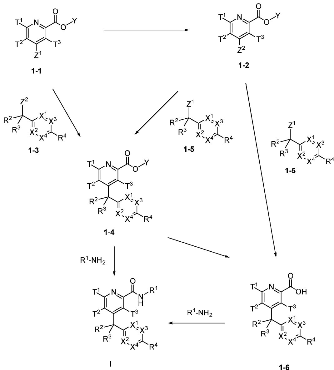
Scheme 1
