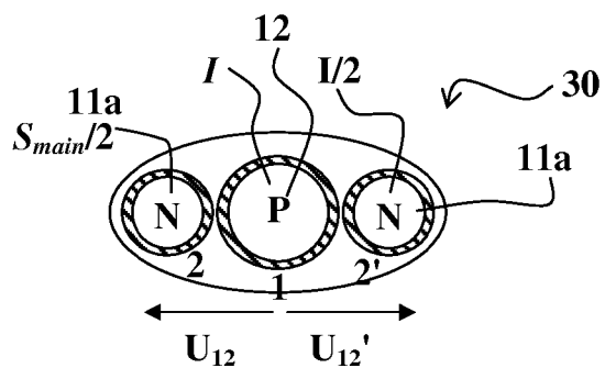
Fig. 2 Single-phase cable type A
