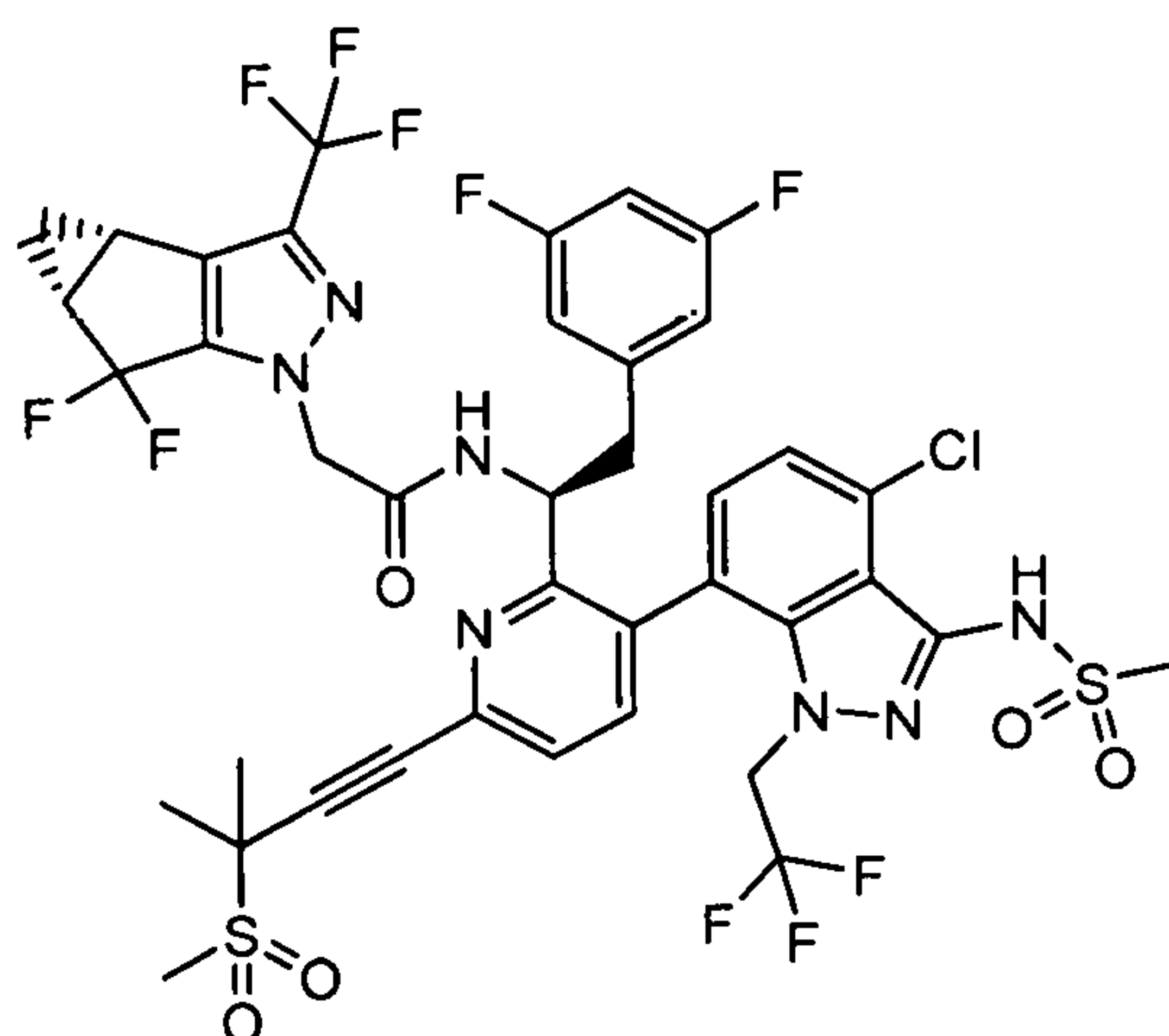
Compound 1
