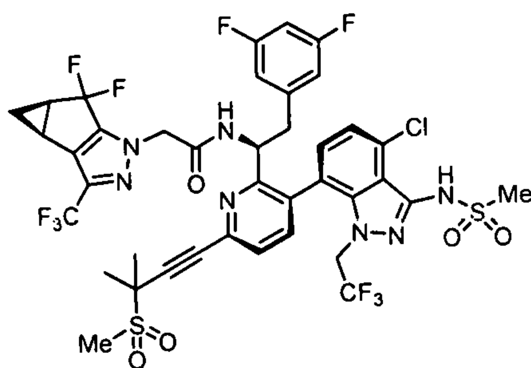
Isomer B
