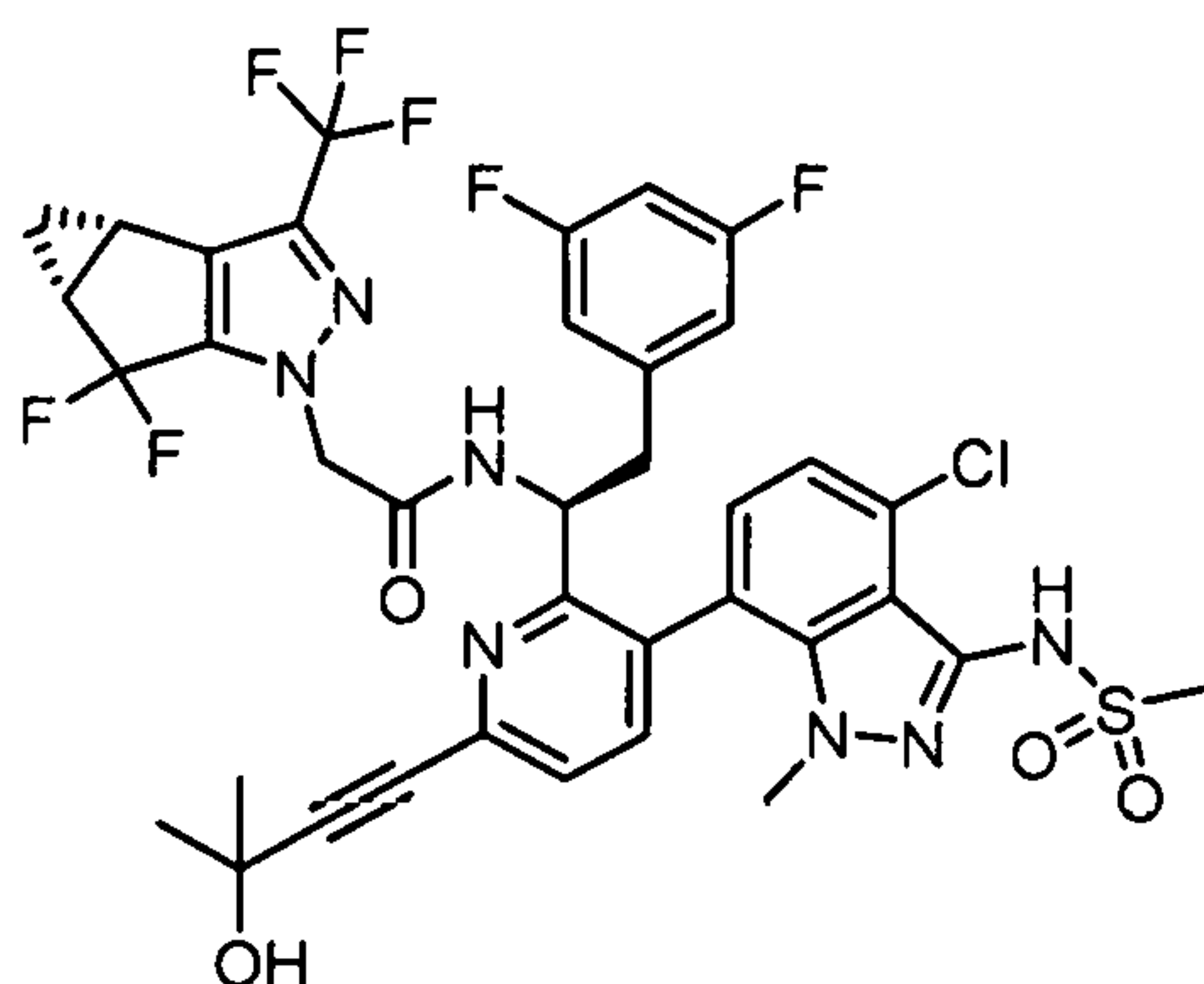
Compound B
