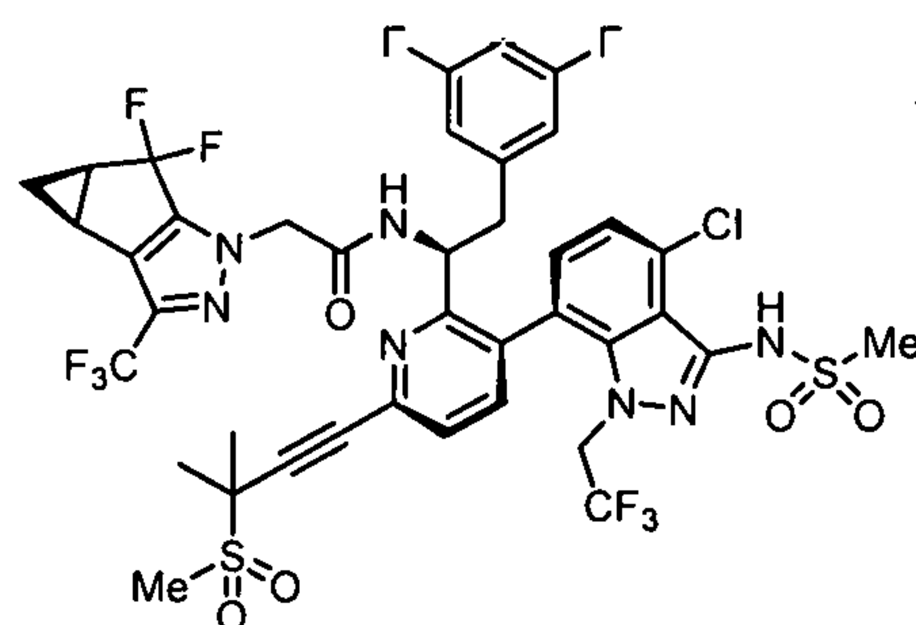
Isomer B
