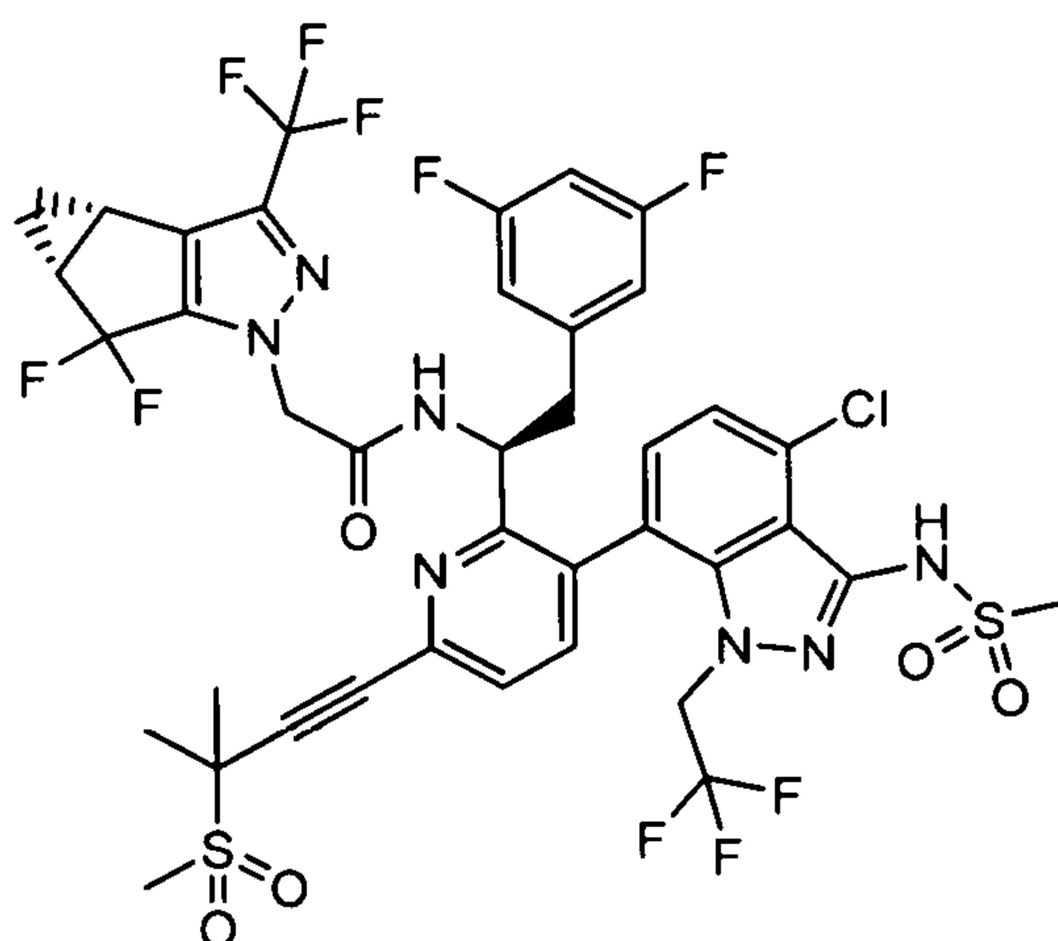
Compound 1
