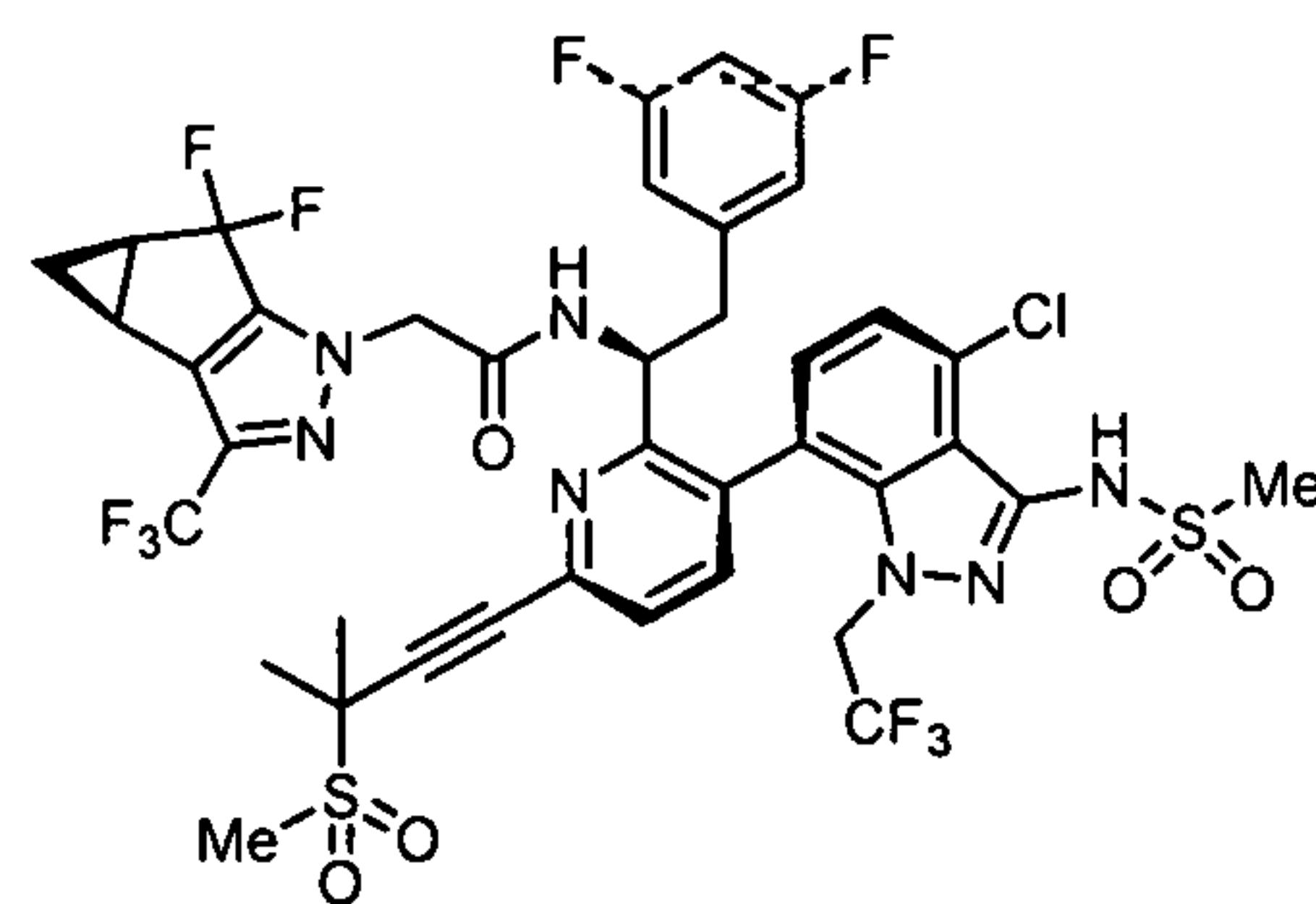
Isomer B
