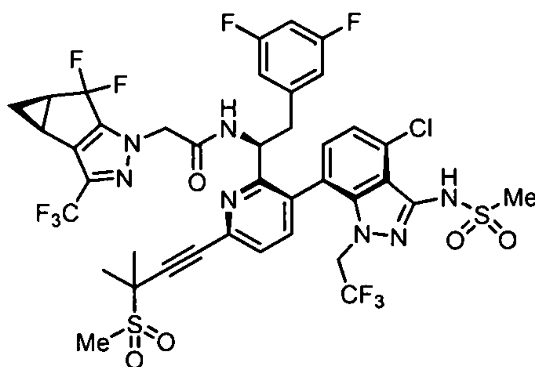
Isomer A
