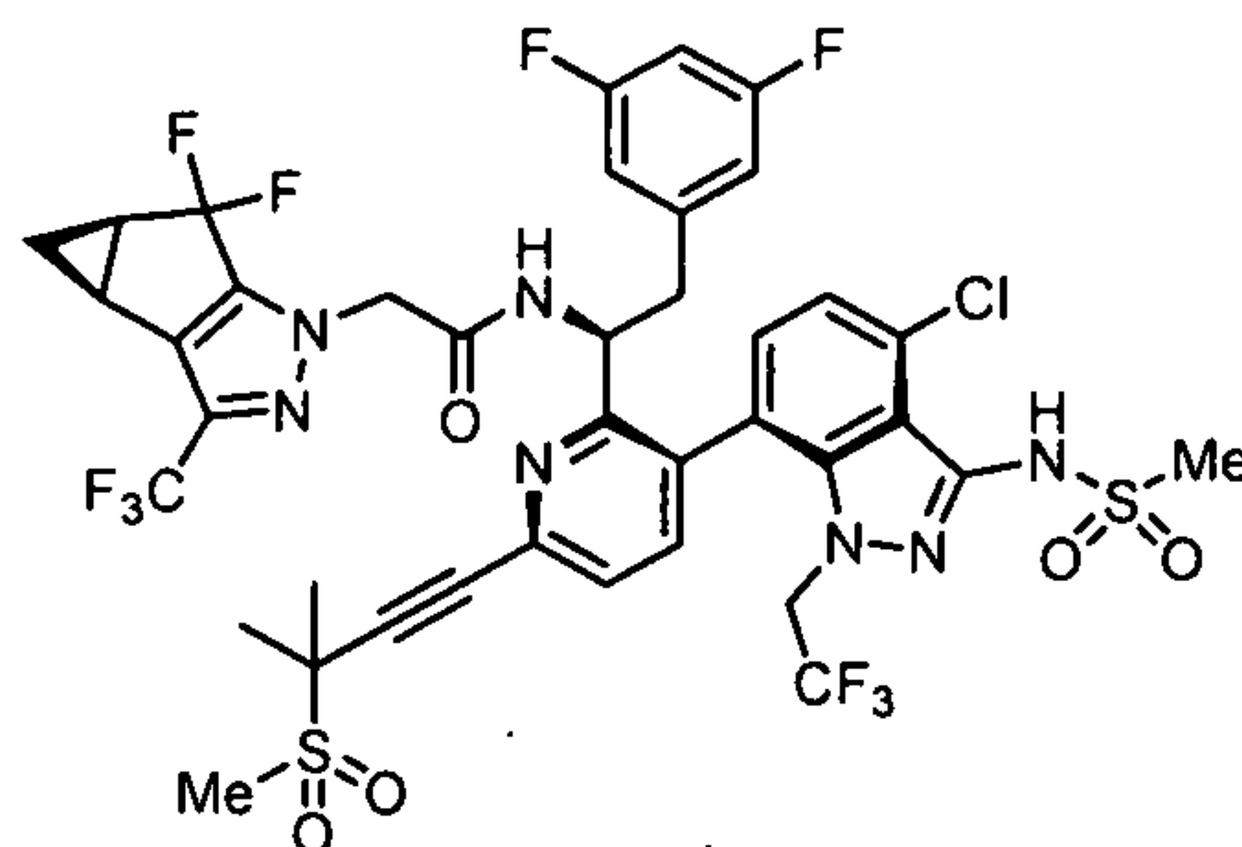
Isomer A
