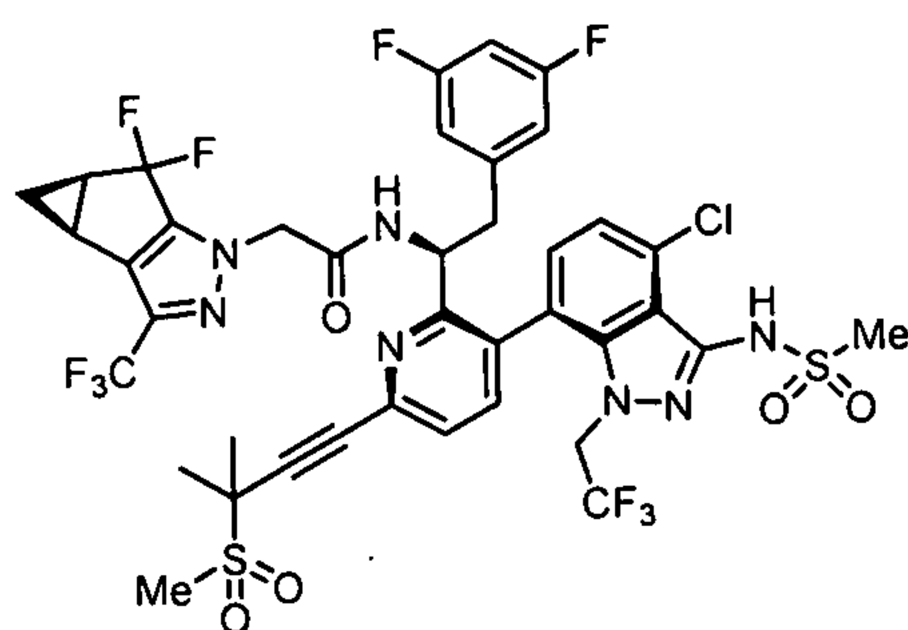
Isomer A
