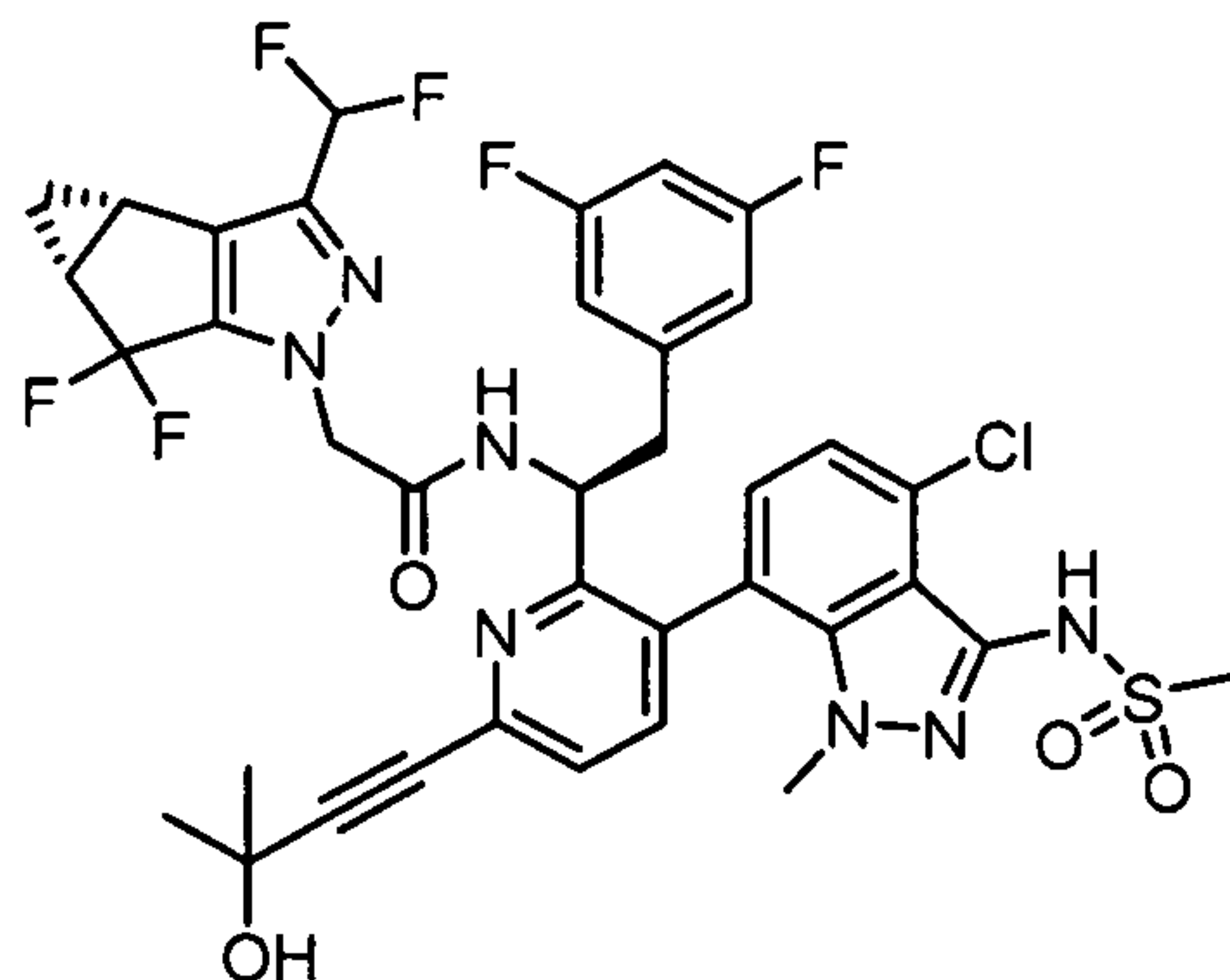
Compound A
