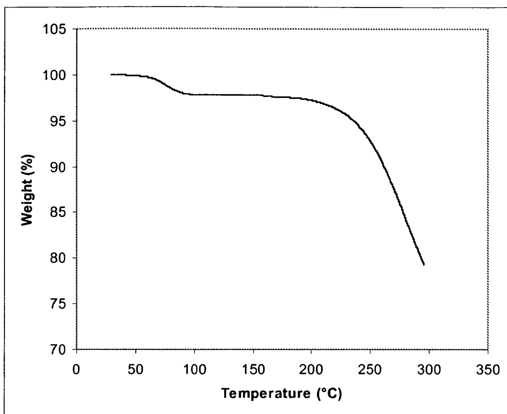
Figure 14: TGA of FORM 2
