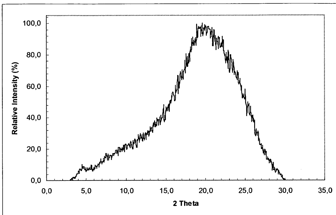
Figure 6: Amorphous modification of FORM 6
