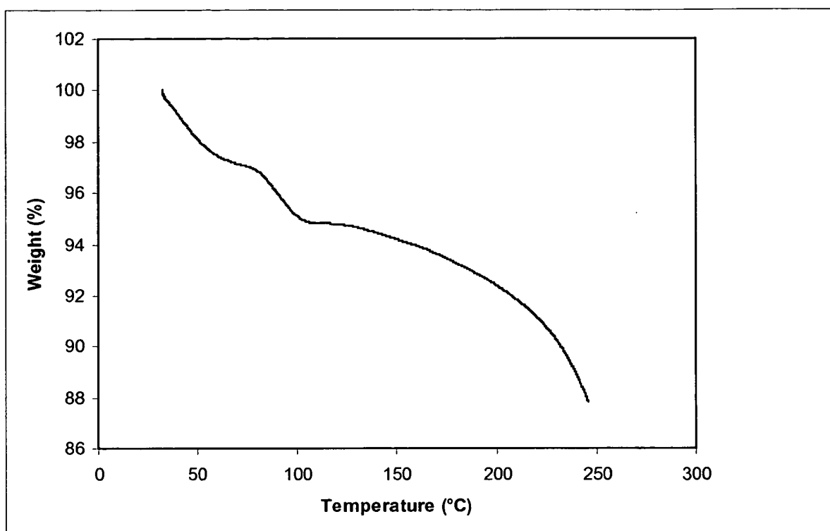
Figure 17: TGA of FORM 6
