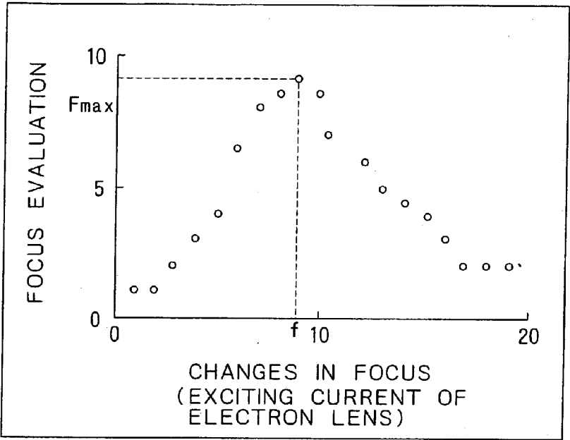
FIG. 2 (PRIOR ART)
