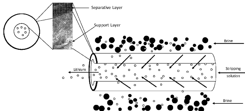
Tubular Membrane Operating in a Cross-Flow Configuration
