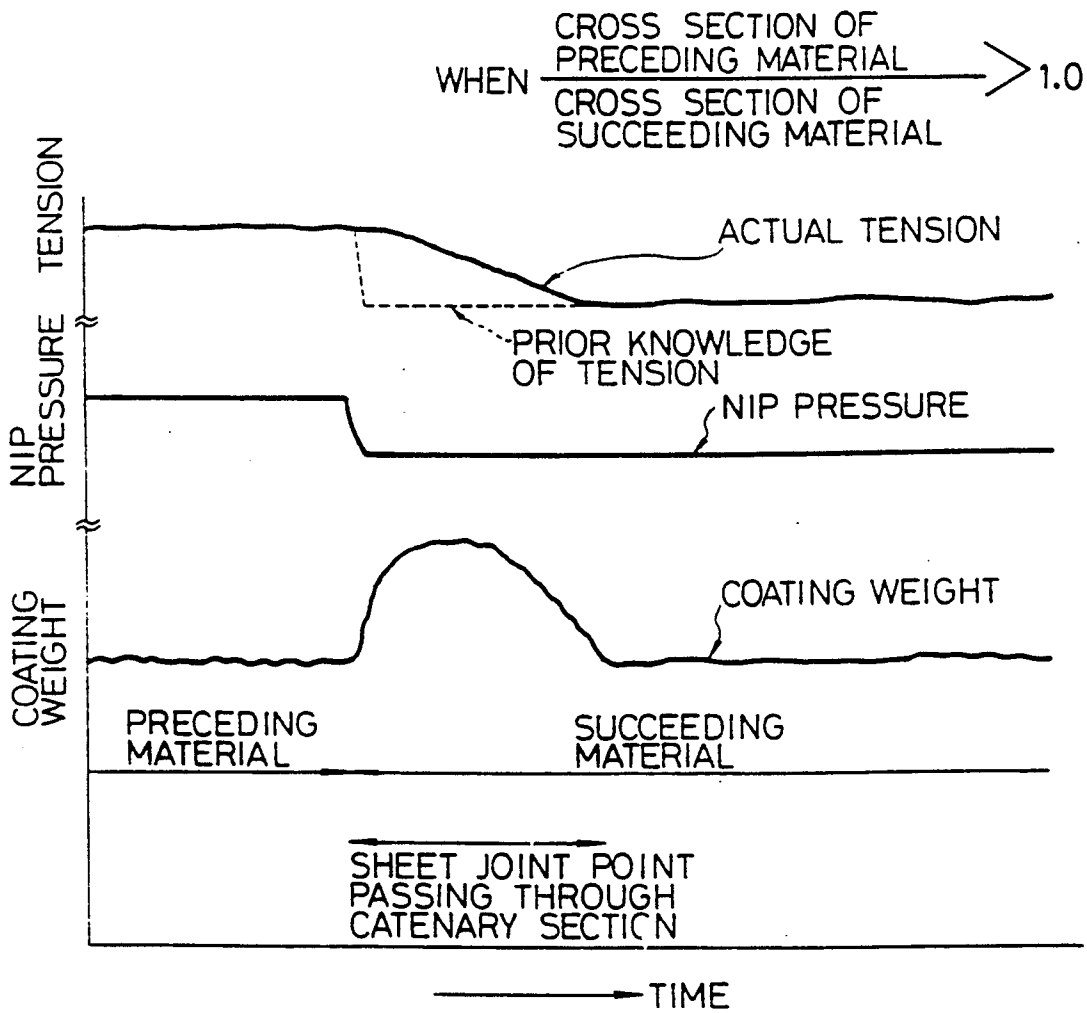
FIG. 45 PRIOR ART
