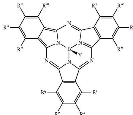
[Chemical Formula 2]
