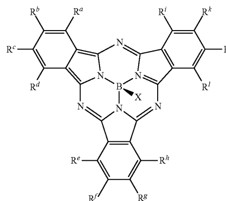
[Chemical Formula 1]
