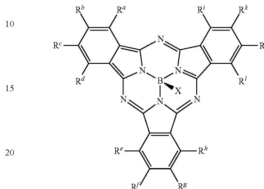
[Chemical Formula 1]
