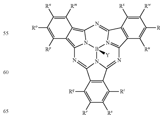
[Chemical Formula 2]
