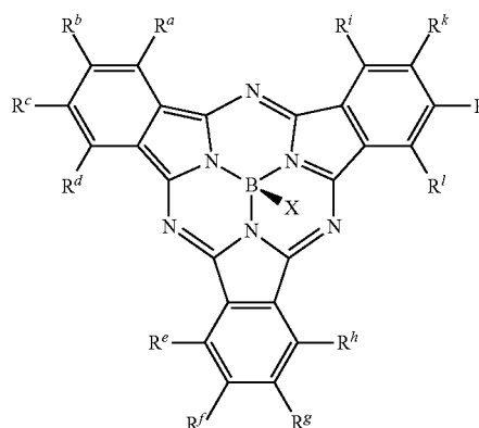
[Chemical Formula 1]
