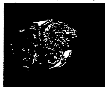
Nanocomplex-Mag
