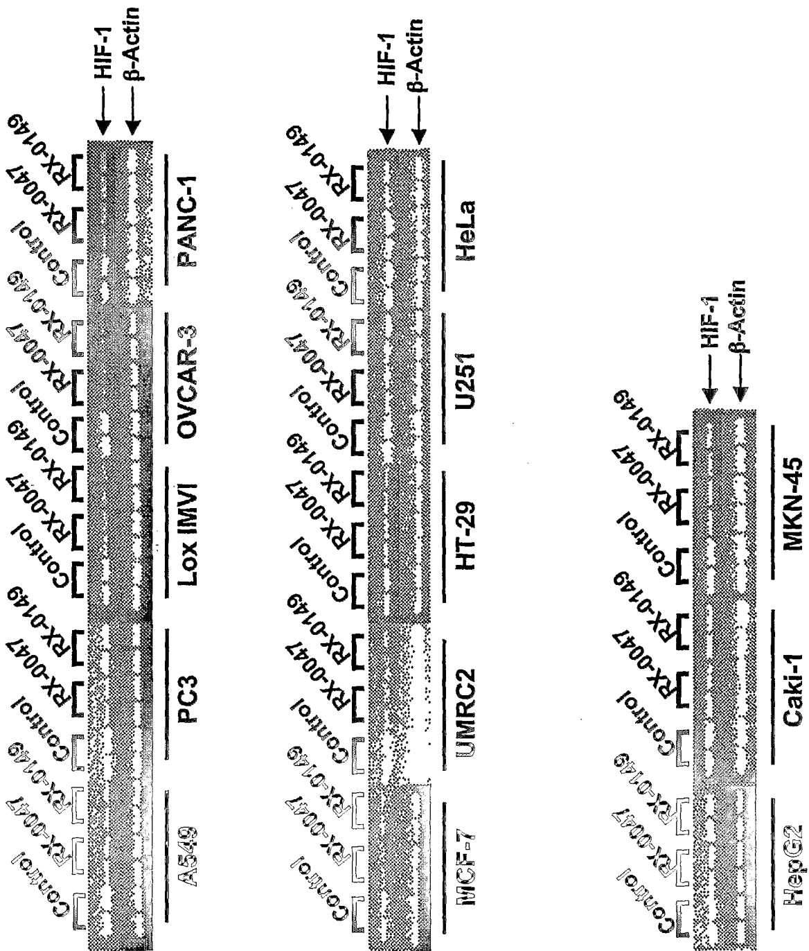
Fig. 1. RX-0047 and RX-0149 inhibit HIF-1 mRNA expression in various cancer cell lines
