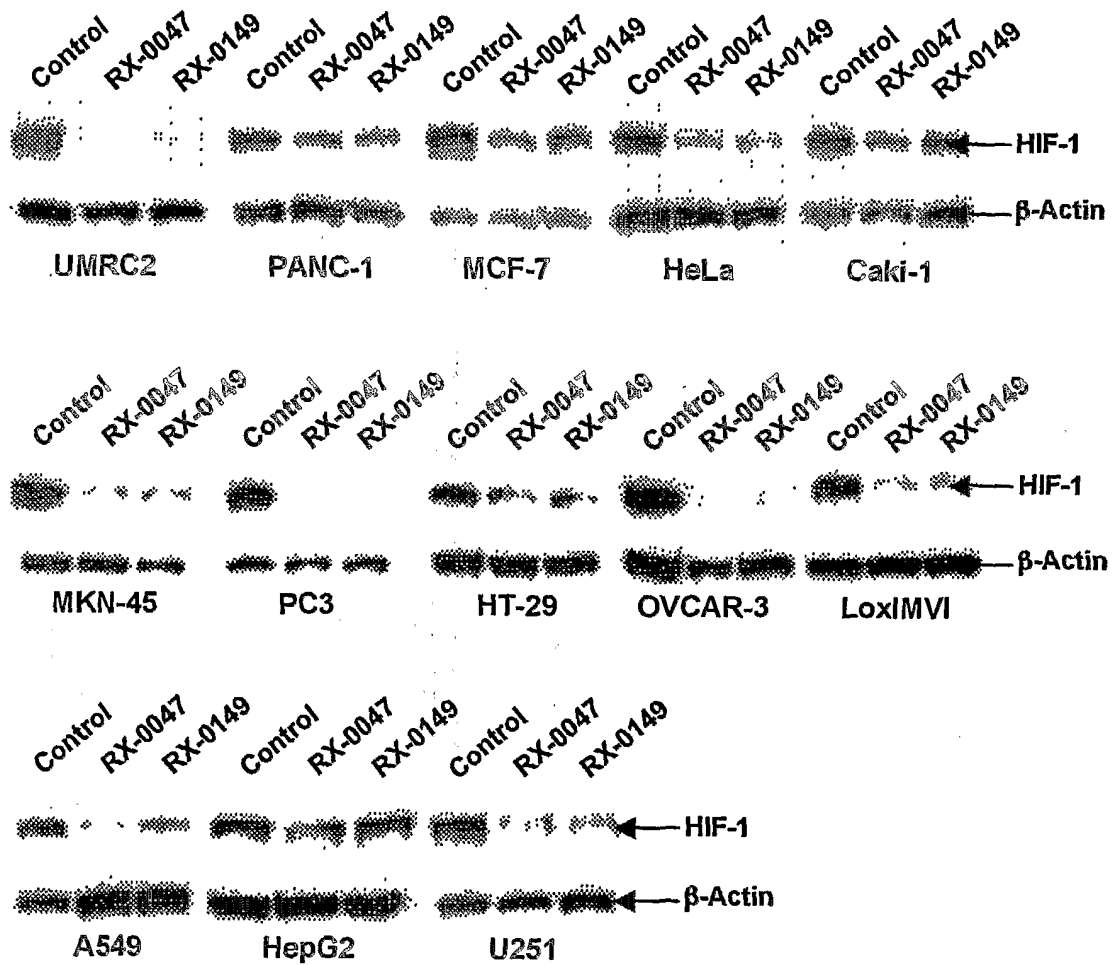
Fig. 2. Western blot analysis of inhibition of HIF-1 protein expression by RX-0047 and RX-0149
