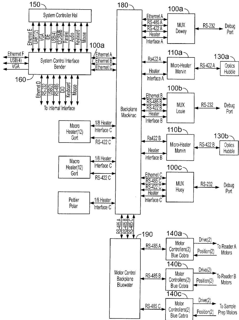
FIG. 86 Electronics Block Diagram
