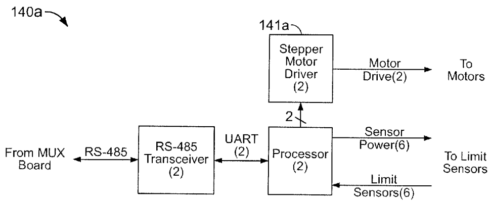
FIG. 91 Motor Control Board Block Diagram
