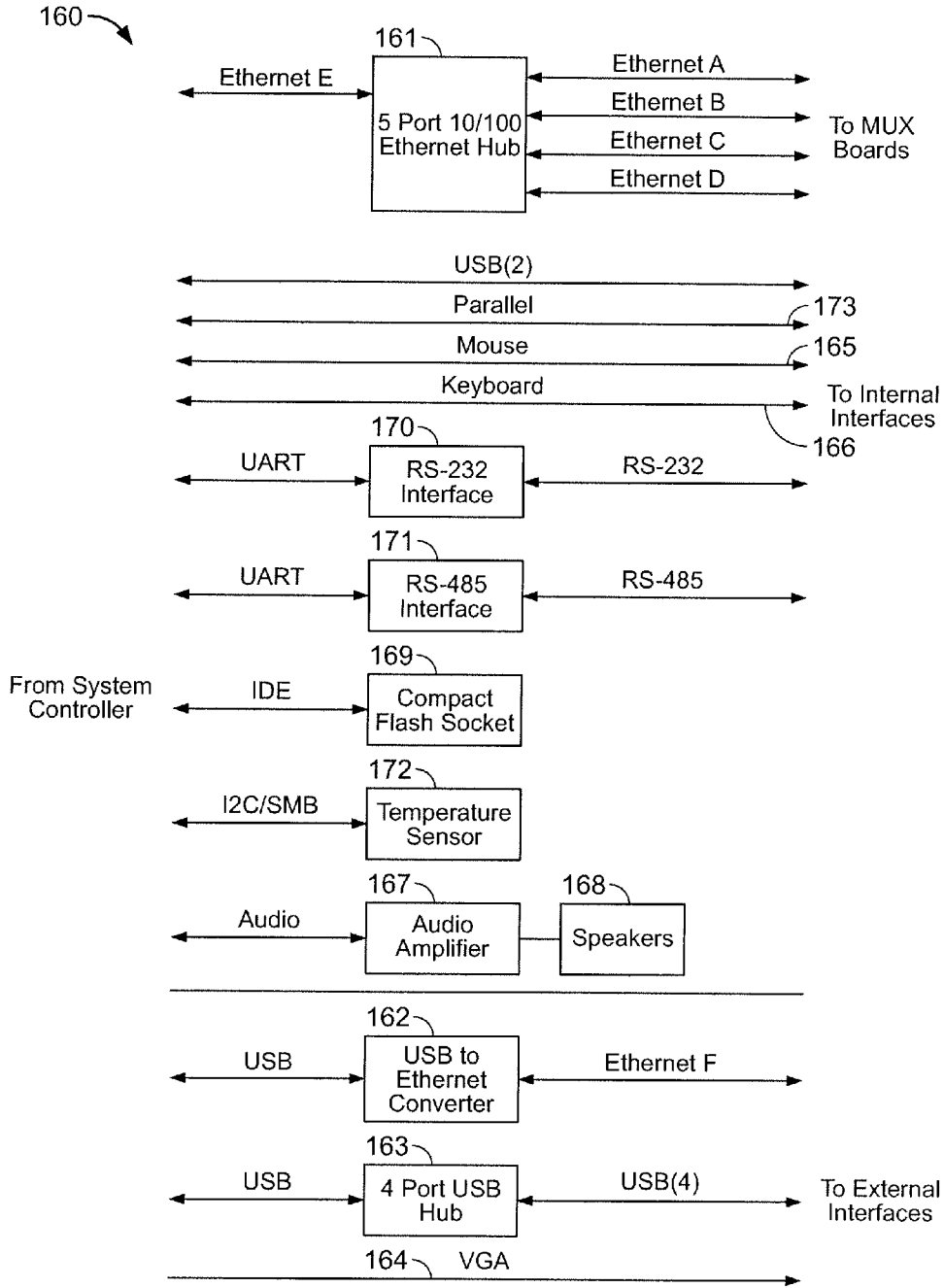
FIG. 87 Processor Base Board Block Diagram
