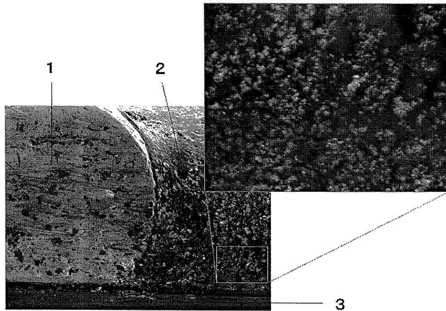
FIG 1 State with curing agent dispersed (before curing)
