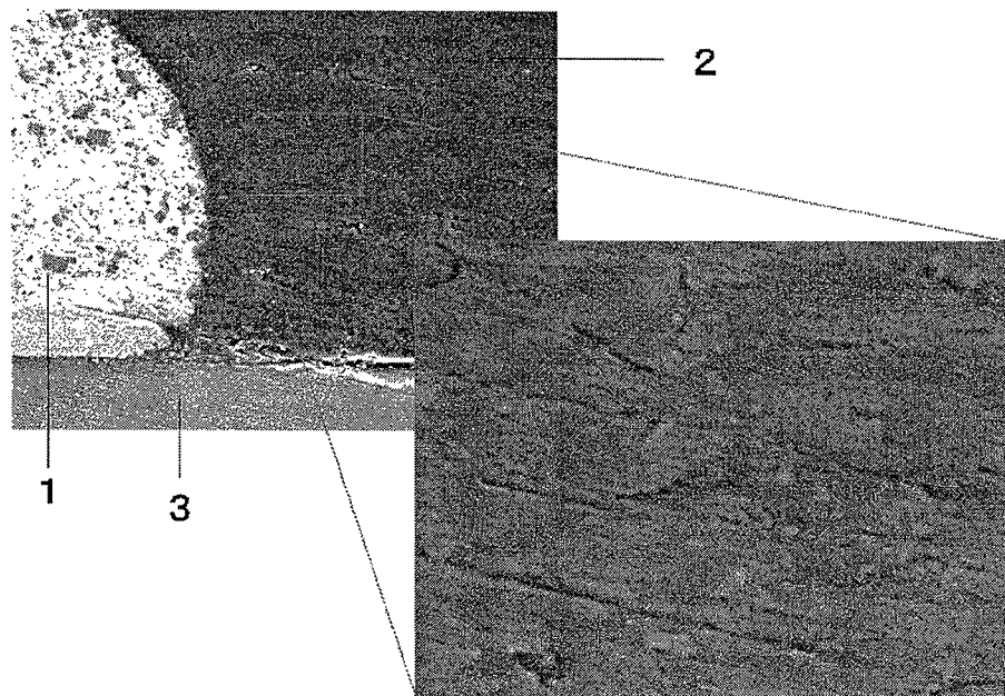
FIG 2 State with particles melted (after curing)
