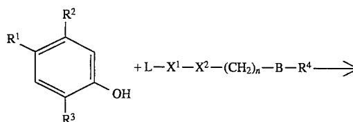
Scheme I
