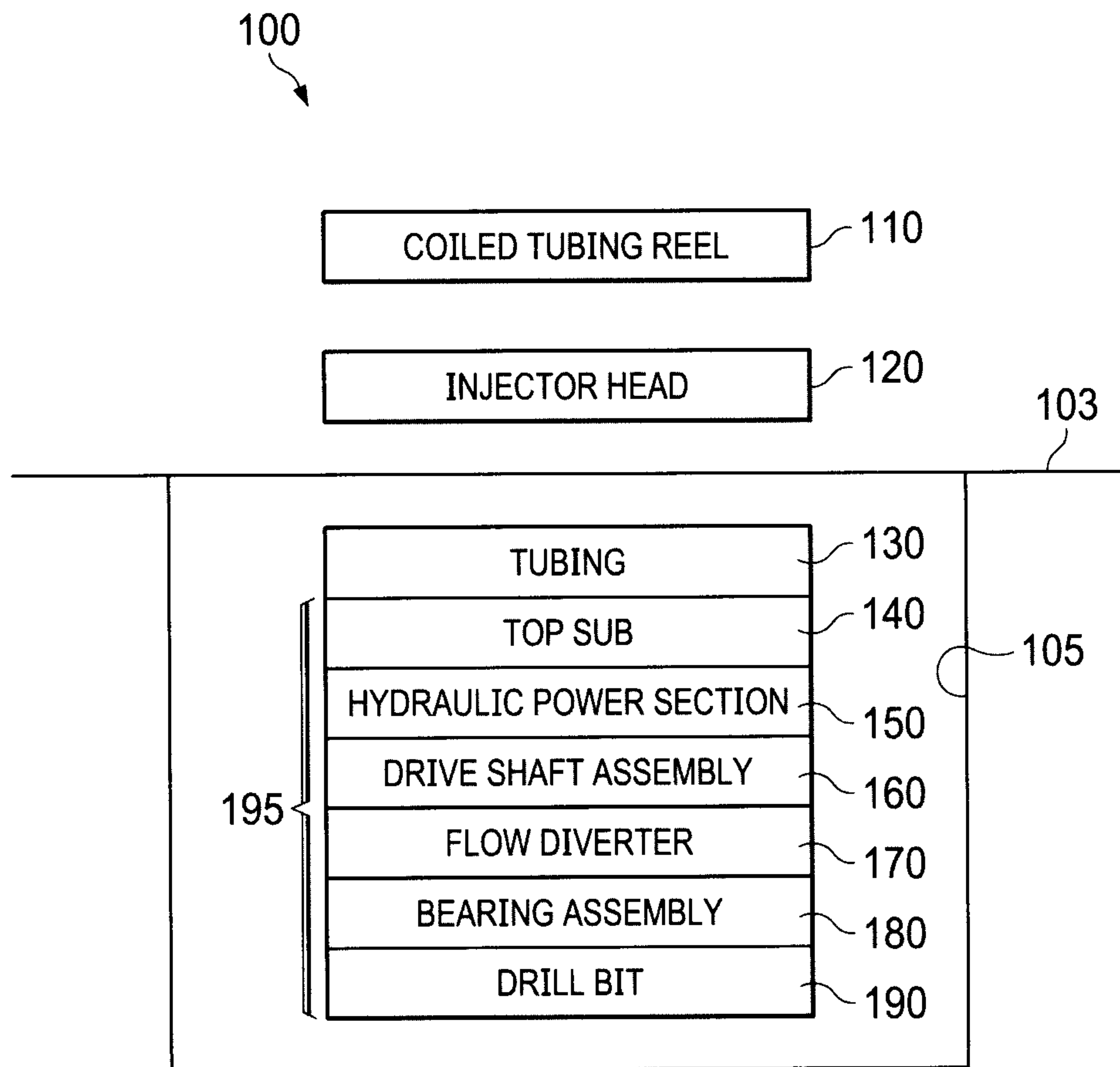
FIG. 1 PRIOR ART
