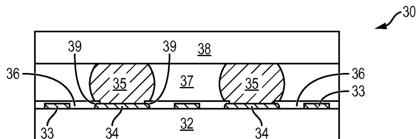
FIG. 3 (PRIOR ART)
