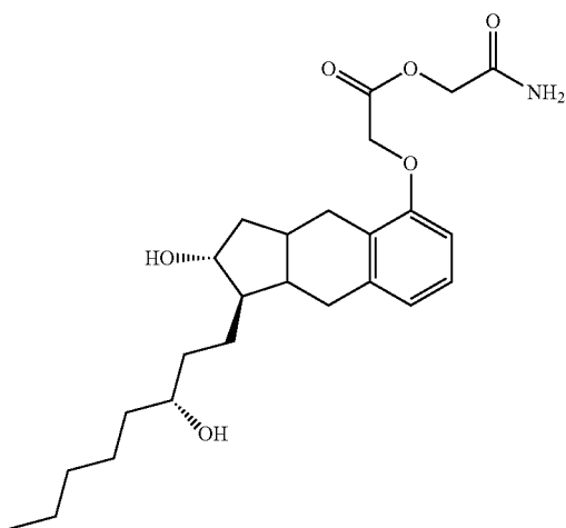
C 25 H 37 NO 6 Exact Mass: 447.26 Mol. Wt.: 447.56 C, 67.09; H, 8.33; N, 3.13; O, 21.45 Treprostinil glycolamide ester
