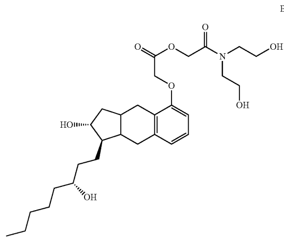
C 29 H 45 NO 8 Exact Mass: 535.31 Mol. Wt.: 535.67 C, 65.02; H, 8.47; N, 2.61; O, 23.89
