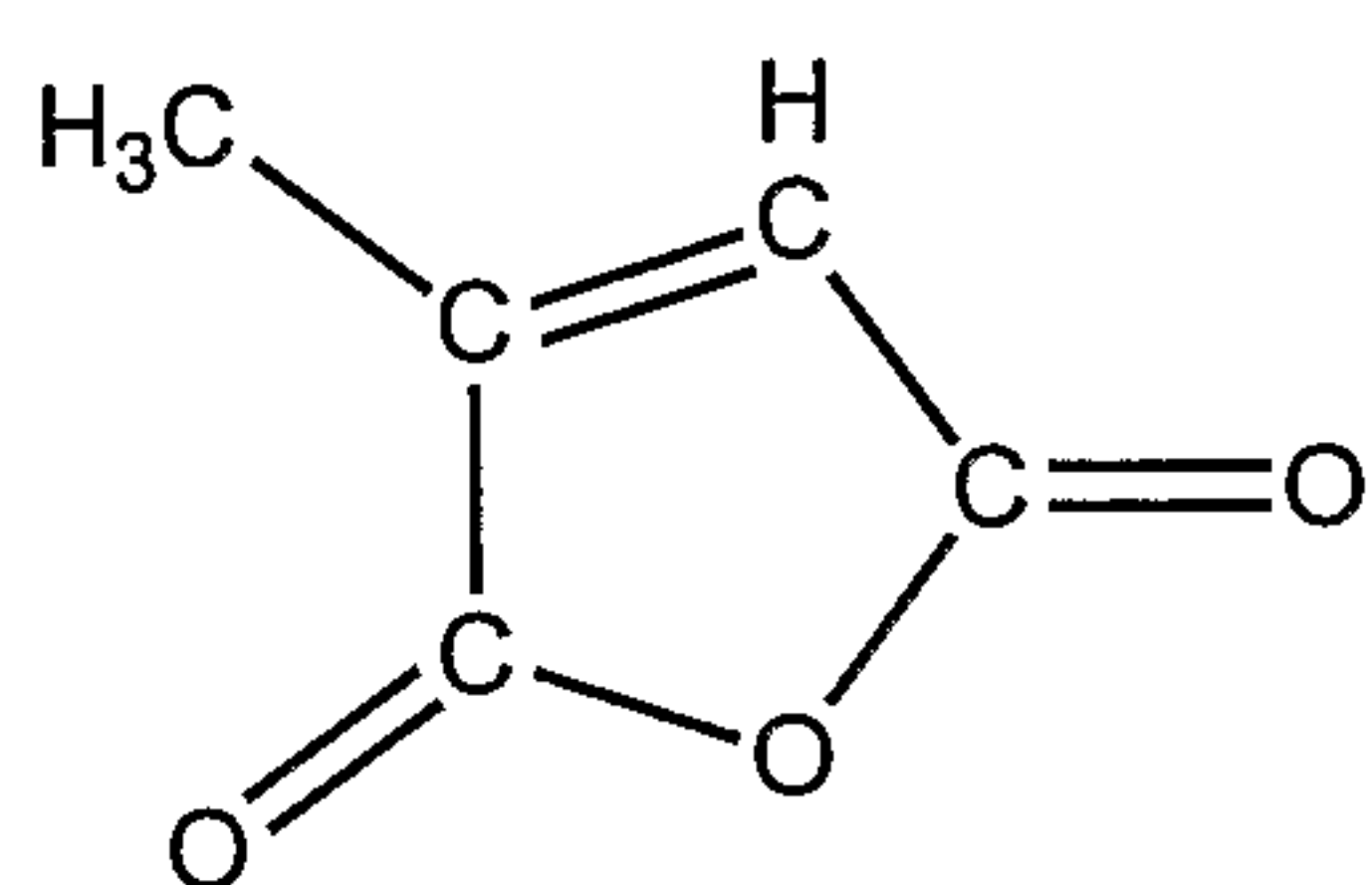
Citraconic Anhydride
