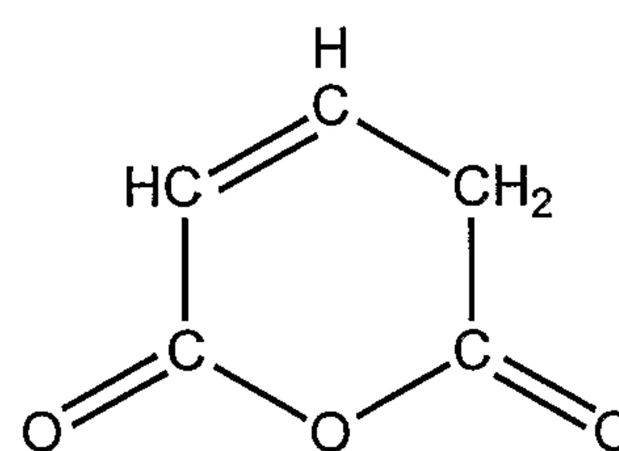
2-Pentendioic Anhydride
