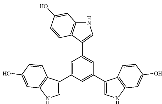
Scheme 3: Chemical structure of compound 2.
